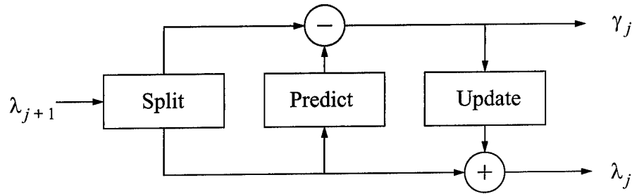
Figure 46. Canonical structure in implementing 1-D discrete forward wavelet transform with lifting.
