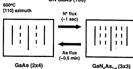
Fig. 1 RHEED Pattern evolution under N^* and As fluxes. Note time scales. GaNAs pattern is commensurate w/ substrate. Reaction is reversible, if N^* exposure time is limited to a few sec.
