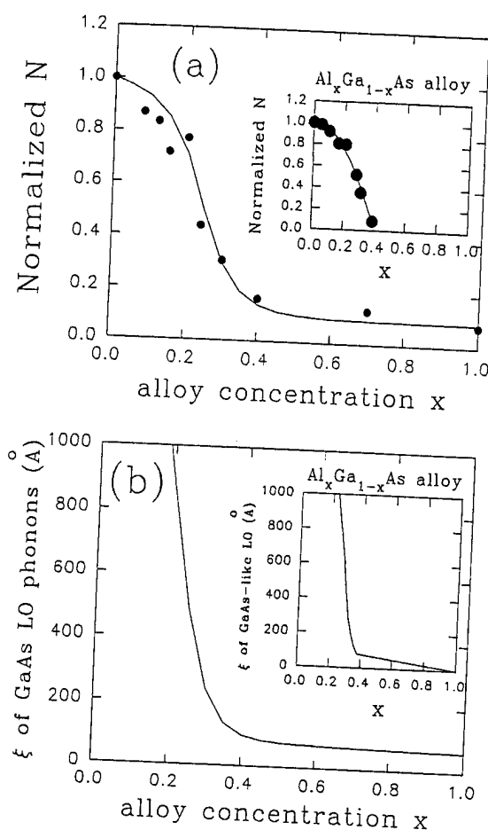
Fig. 3. (a) The normalized (to bulk GaAs under the same experimental conditions) hot phonon occupation number of \text{GaAs}/\text{Al}_x\text{Ga}_{1-x}\text{As} multiple quantum well as a function of x . The results were averaged over picosecond and cw excitations, in the temperature range 10–300 K. The line is a fit as a guide to the eye. (Inset) The normalized and properly corrected (for the band gap change with x ) hot phonon occupation number as a function of x for the \text{Al}_x\text{Ga}_{1-x}\text{As} alloys. (b) The coherence length obtained from the solid lines of Fig. 3(a), assuming a coherence length of infinity for the bulk GaAs LO phonon, and a phenomenological wave function \Psi = \exp(iq_0z) \exp(-z^2/\xi^2) . (Inset) The same as (b) for the \text{Al}_x\text{Ga}_{1-x}\text{As} alloys.
