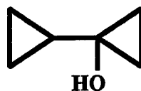
2: 1-cyclopropyl-cyclopropan-1-ol
