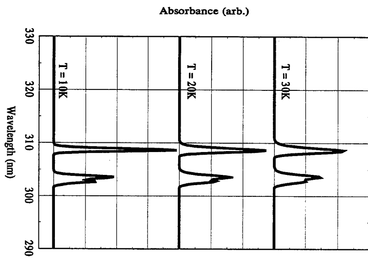
ALAr4 Absorption Spectra
