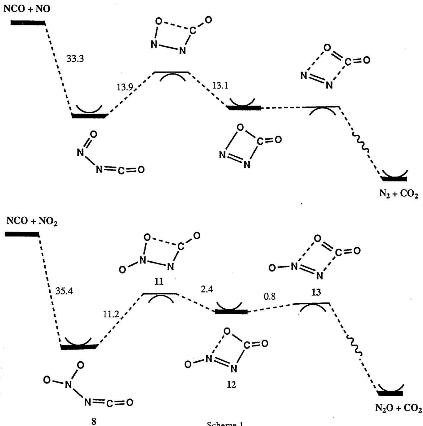
Scheme 1
