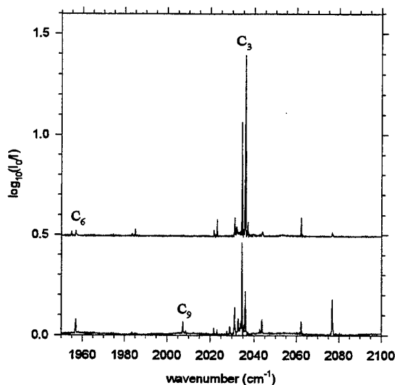
Figure 6. IR Absorptions of Carbon Clusters in pH_2 at T = 2 K. The sample was prepared by laser ablation of graphite. The top trace shows the as-deposited sample, with: T = 2 K, \lambda_{abl} = 308 nm, \Phi_{abl} \approx 8 \times 10^7 W/cm ^2 , 100 mJ/pulse, 10 Hz repetition rate, 30 minute C_n deposition time, H_2 inlet flow rate \approx 120 mmol/hr, l = 1.2 mm. The bottom trace shows the sample again at 2 K, after warming to 4 K. Resolution is 0.15 cm^{-1} FWHM.
