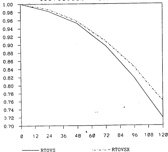
T79L18 DATA ASSIMILATION TEST 500 MB EAST PAC HEIGHT ANOMALY COR 1997110112 - 1997113012
