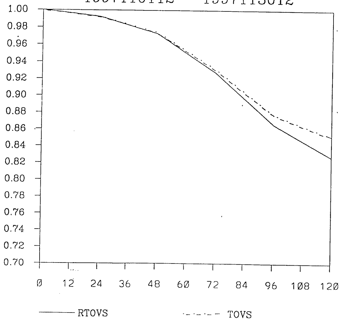
Figure 2: A comparison of the average 500 mb height anomaly correlation using the retrievals from the older TOVS algorithm and from the new RTOVS algorithm in the T79L18 version of NOGAPS over the Atlantic Ocean for the month of November 1997.
