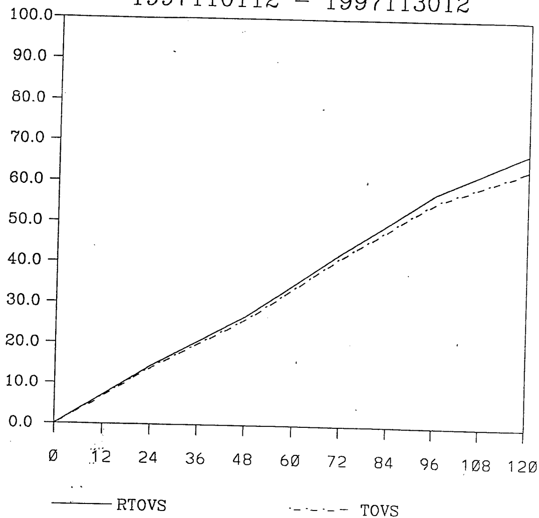
Figure 5: A comparison of the average 500 mb height root mean square error over the Atlantic Ocean for the month of November 1997 using the retrievals from the older TOVS algorithm and from the new RTOVS algorithm in the T79L18 version of NOGAPS.
