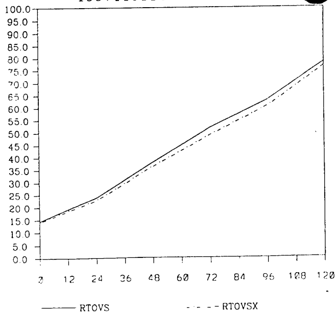
T79L18 DATA RAOB COMPARISON 500 MB ASIA RMS HEIGHT ERROR 1997110112 - 1997113012
