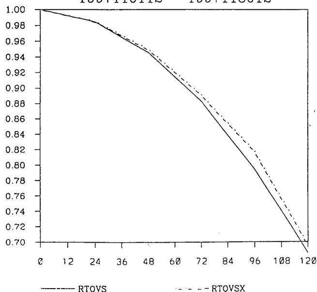
T79L18 DATA ASSIMILATION TEST 500 MB EURASIA HEIGHT ANOMALY COR 1997110112 - 1997113012
