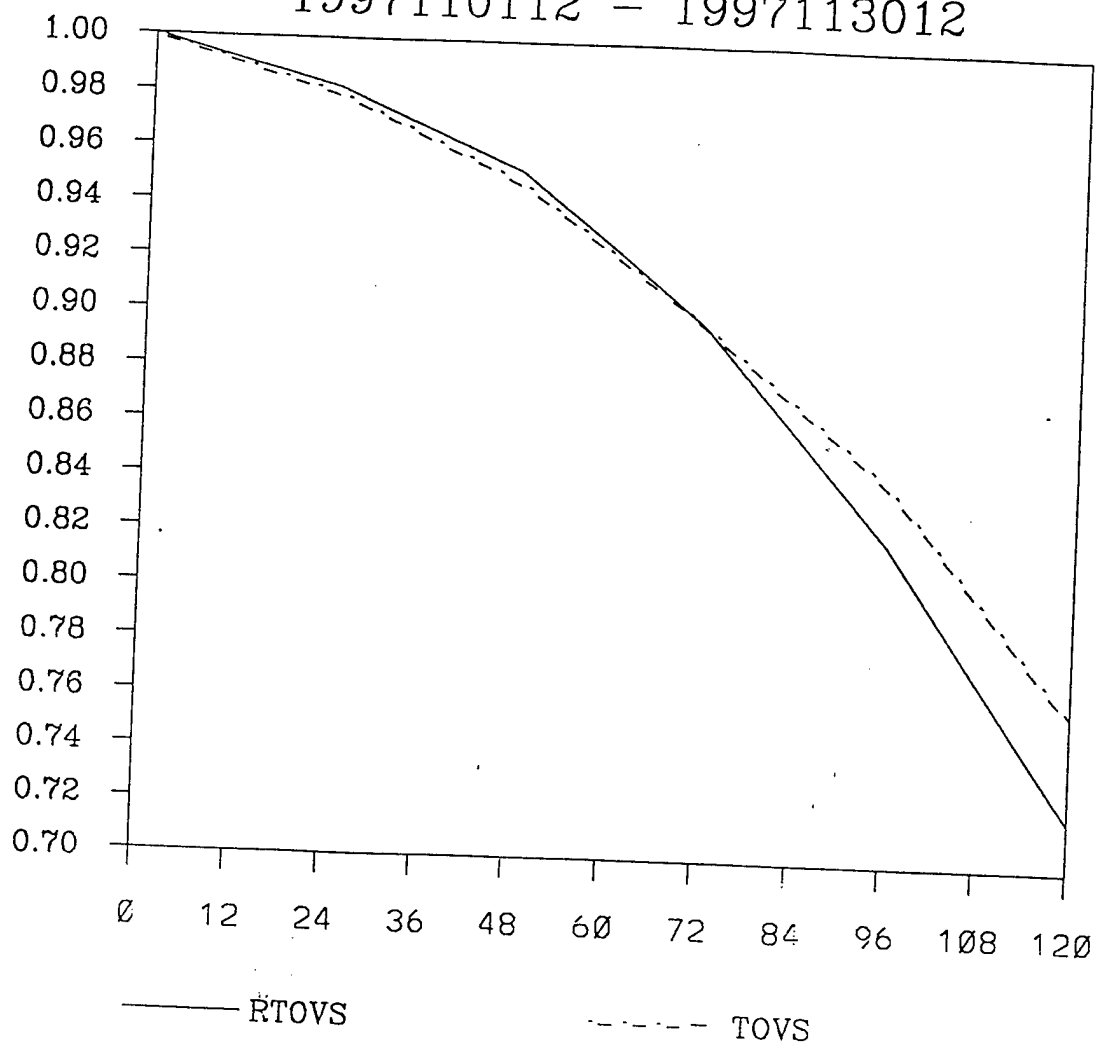
Figure 3: A comparison of the average 500 mb height anomaly correlation over the Eastern Pacific Ocean for the month of November 1997 using the retrievals from the older TOVS algorithm and from the new RTOVS algorithm in the T79L18 version of NOGAPS.
