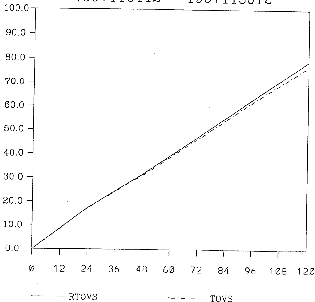
Figure 4: A comparison of the average Northern Hemisphere's 500 mb height root mean square error for the month of November 1997 using the retrievals from the older TOVS algorithm and from the new RTOVS algorithm in the T79L18 version of NOGAPS. The x axis is forecast hours (0-120 hours) and the y axis is root mean square error in meters.
