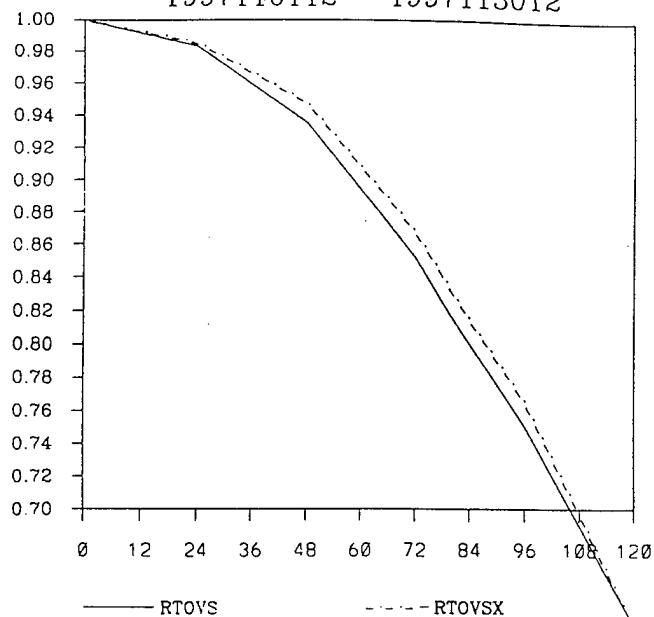
T79L18 DATA ASSIMILATION TEST 500 MB N AMERICA HEIGHT ANOMALY COR 1997110112 - 1997113012
