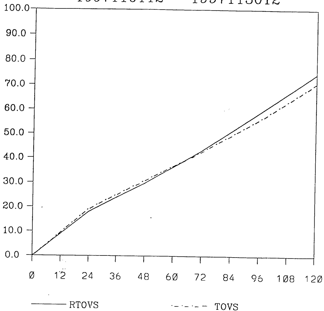
Figure 6: A comparison of the average 500 mb height mean square error over the Eastern Pacific Ocean for the month of November 1997 using the retrievals from the older TOVS algorithm and from the new RTOVS algorithm in the T79L18 version of NOGAPS.
