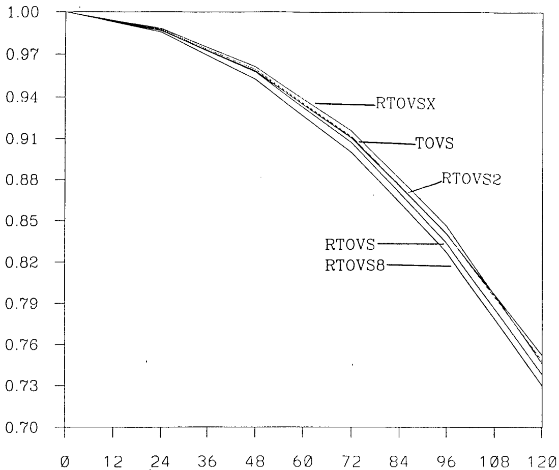
Figure 8: A comparison of the average Northern Hemisphere's 500 mb height anomaly correlation for the month of November 1997 using TOVS, the new RTOVS retrievals, and 3 different satellite errors for the RTOVS data, RTOVS2, RTOVS8, and RTOVSX (see the text for details). All test were conducted with the T79L18 version of NOGAPS.
