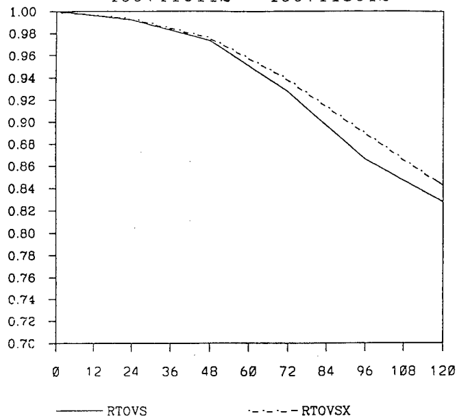
T79L18 DATA ASSIMILATION TEST 500 MB ATLANTIC HEIGHT ANOMALY COR 1997110112 - 1997113012
