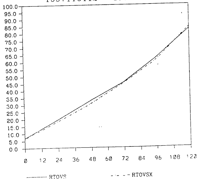
T79L18 DATA RAOB COMPARISON 500 MB EUROPE RMS HEIGHT ERROR 1997110112 - 1997113012
