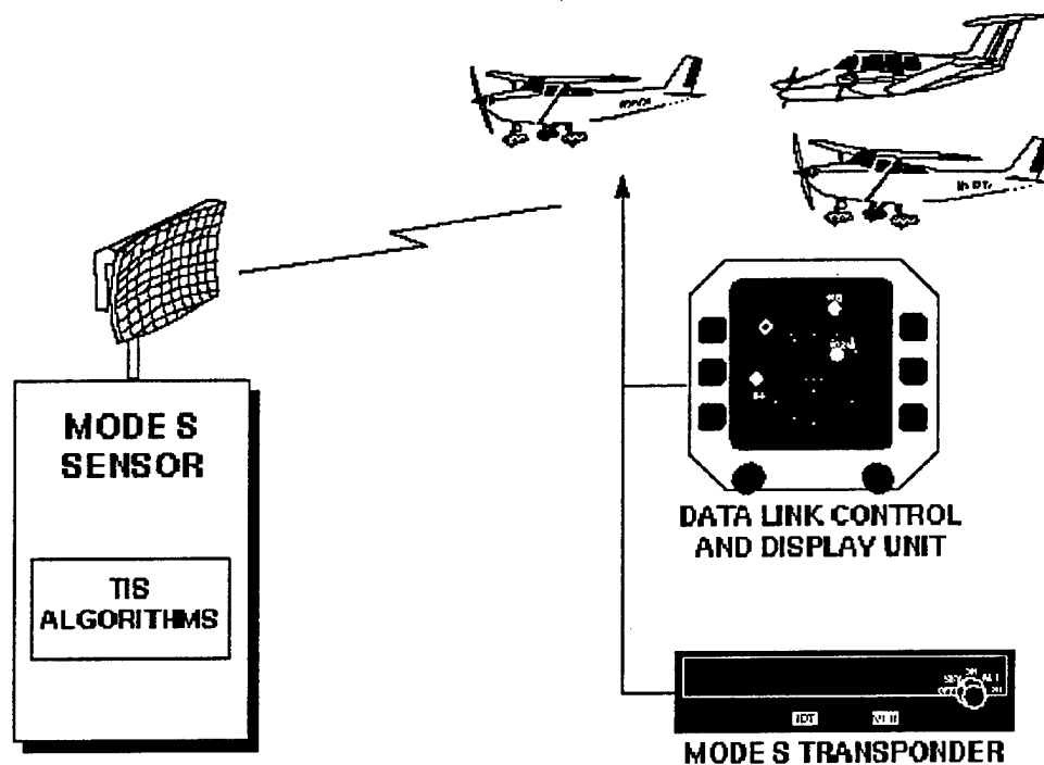
FIGURE 3.1- 1. FUNCTIONAL ELEMENTS OF TIS
