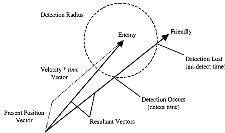
Figure C-3. Scheduling Detections
