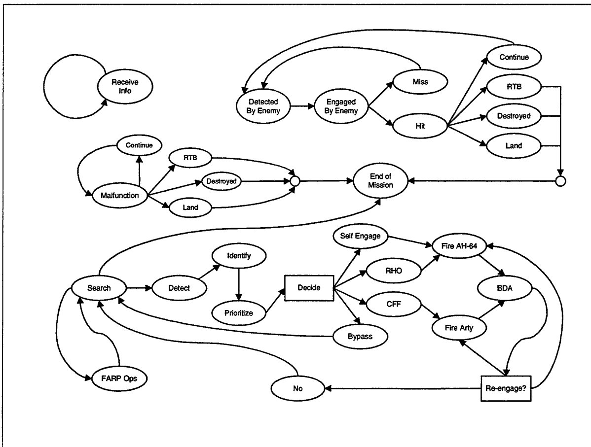
Figure 4. Simulation Flow
