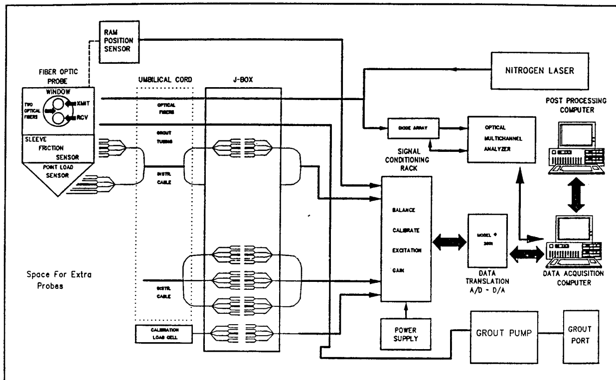
FIGURE 4-1. TRI-SERVICES SCAPS
