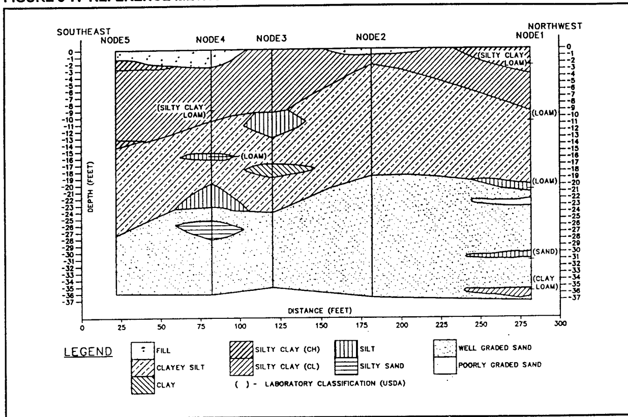
FIGURE 3-7. REFERENCE METHOD STRATIGRAPHIC CROSS SECTION—ATLANTIC SITE
