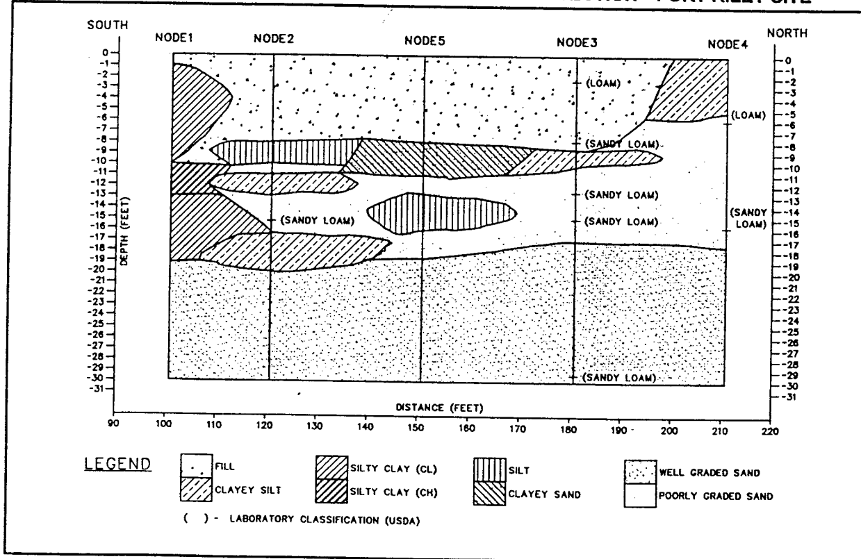
FIGURE 3-9. REFERENCE METHOD STRATIGRAPHIC CROSS SECTION—FORT RILEY SITE
