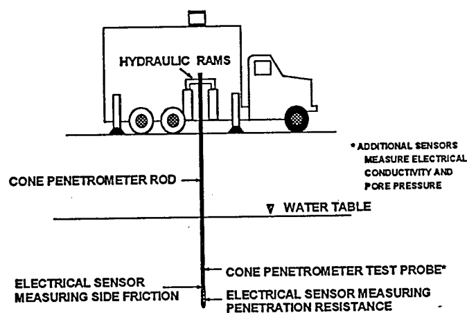
Figure 1. Cone Penetrometer
