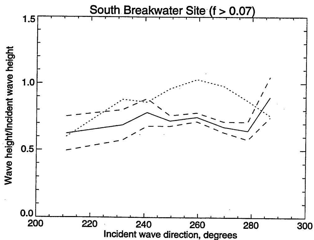
Figure 16. Regression results, south breakwater site
