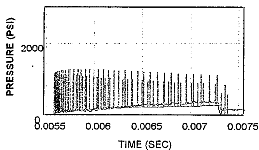
PRESSURE-TIME CURVES
