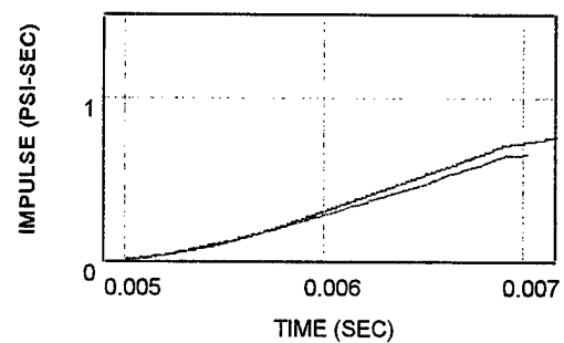
IMPULSE-TIME CURVES
