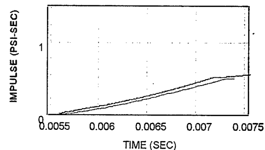
IMPULSE-TIME CURVES
