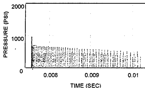
PRESSURE-TIME CURVES
