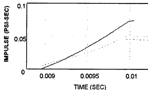
IMPULSE-TIME CURVES
