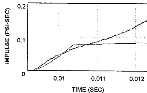
IMPULSE-TIME CURVES
