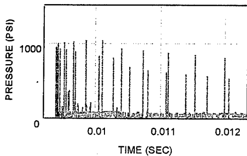
PRESSURE-TIME CURVES
