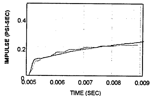
IMPULSE-TIME CURVES
