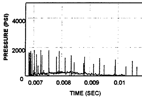
PRESSURE-TIME CURVES
