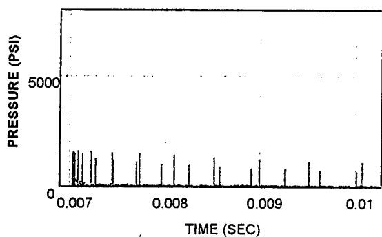
PRESSURE-TIME CURVES
