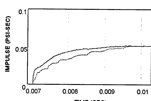
IMPULSE-TIME CURVES
