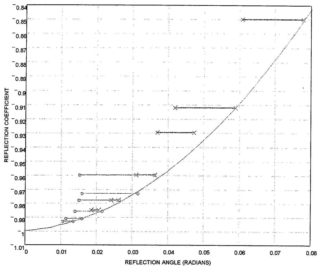
Figure 18. D-Sabre Reflection Coefficients Versus Angle
