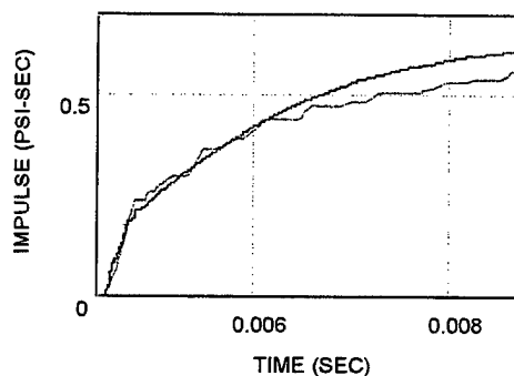
IMPULSE-TIME CURVES
