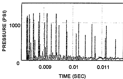
PRESSURE-TIME CURVES
