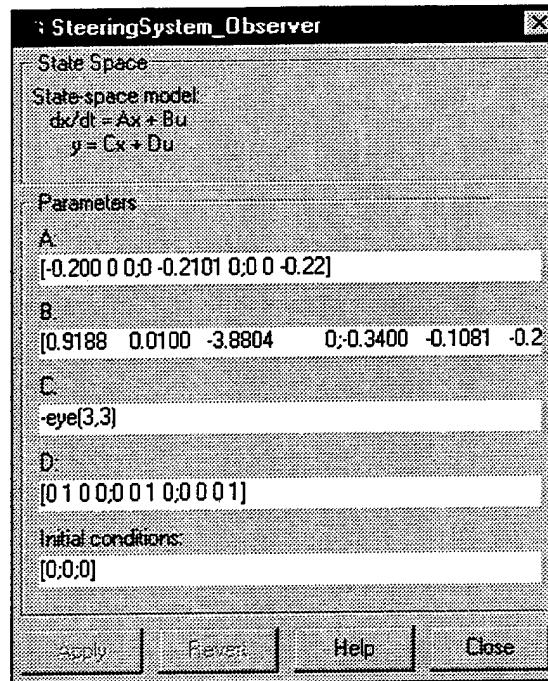
Figure 4.16 Steering System Observer Input Block
