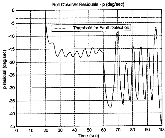
Figure 5.21 Roll Observer Residual p for Scenario 6
