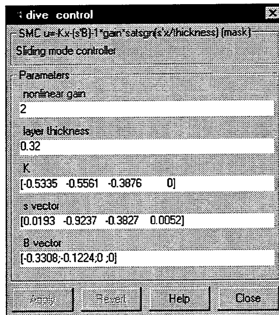
Figure 4.8 Dive Control Input Block
