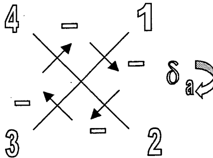
Figure 4.24 Roll Command, \delta_a , Example (Stern View)
