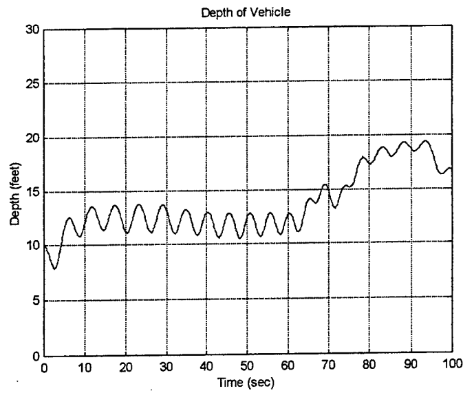
Figure 5.19 Depth of Vehicle for Scenario 6
