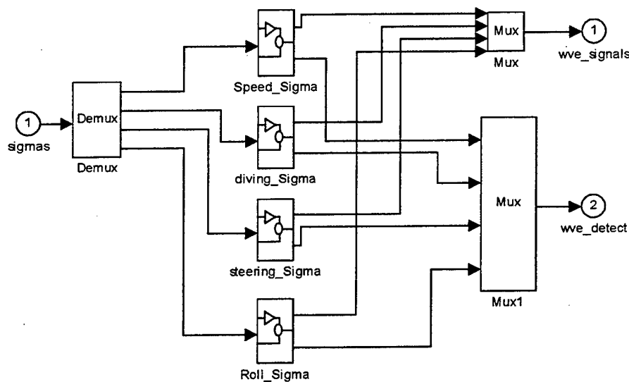
Figure 4.14 Wave Motion Detector Block Diagram
