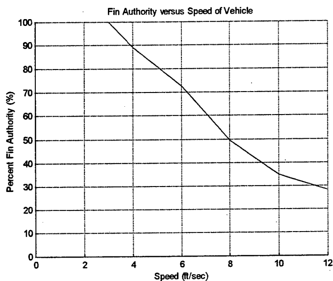
Figure 5.27 Percent Fin Authority versus Speed of Vehicle Expended for 2% mismatch of Weight and Buoyancy
