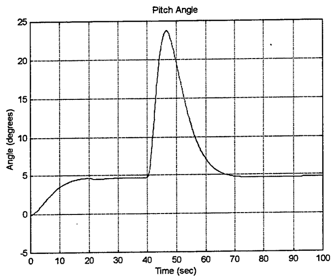
Figure 5.7 Pitch Angle for Scenario 2
