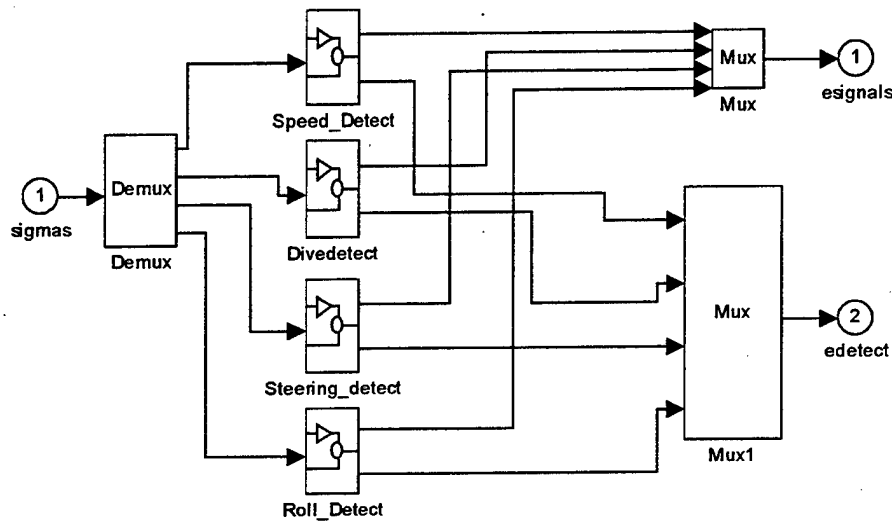
Figure 4.12 Servo Error Detector Block Diagram
