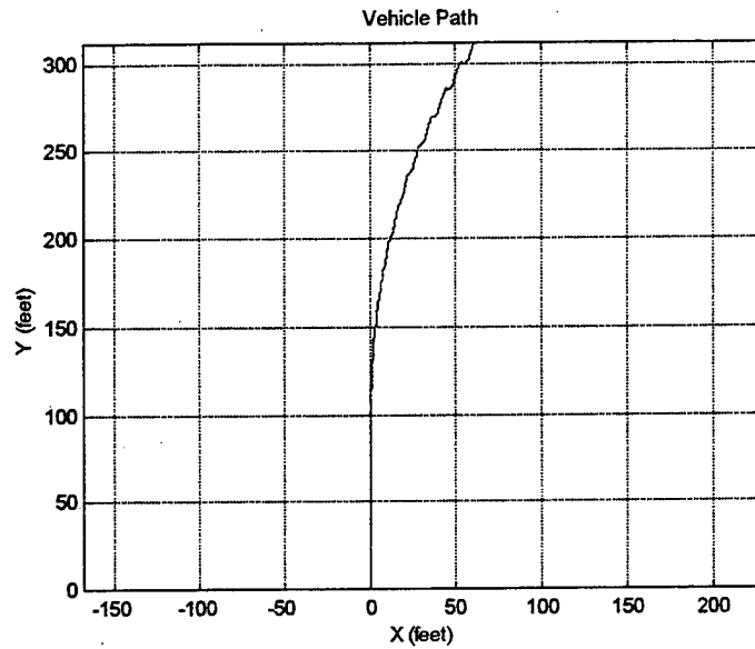
Figure 5.24 Vehicle Path for Scenario 8
