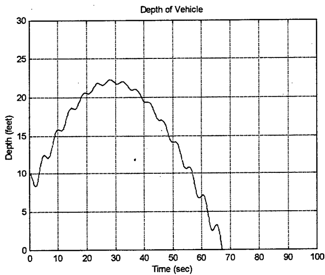
Figure 5.25 Depth of Vehicle for Scenario 8
