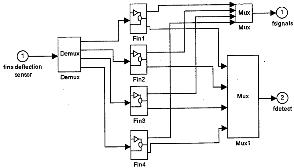
Figure 4.13 Fins Deflection Detector Block Diagram
