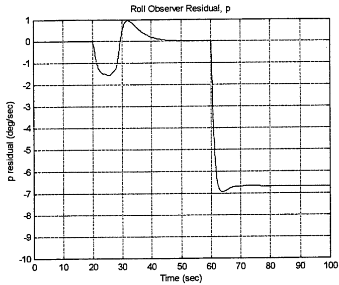
Figure 5.22 Roll Observer Residual, p , for Scenario 7
