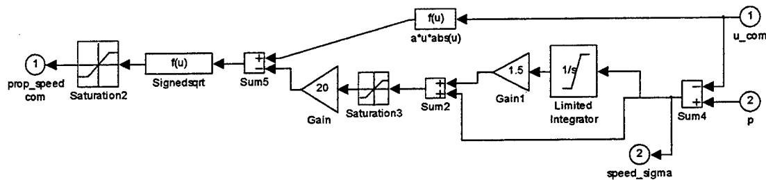
Figure 4.11 Speed Control System
