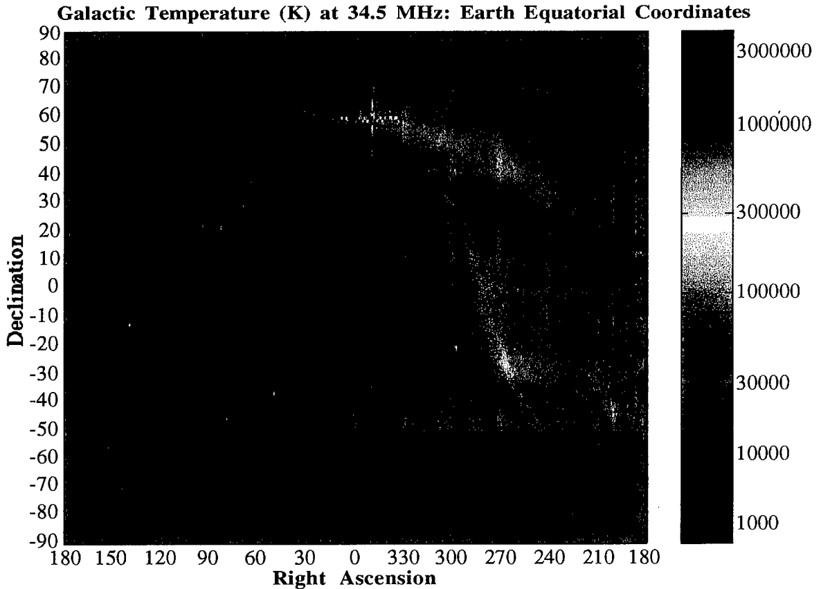
Figure 2. All-Sky Temperature Survey at 34.5 MHz
