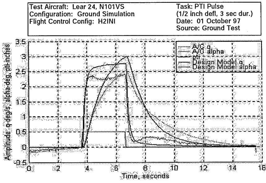
Figure C3 Ground Test Closed-Loop q and \alpha Time Responses - H2INI
