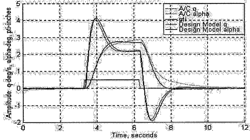
Figure C5 Ground Test Closed-Loop q and \alpha Time Responses - MXAOA
