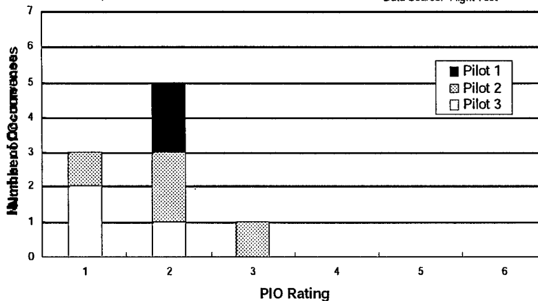
Figure D12 Horizontal Offset Landing PIO Ratings - H2INI
