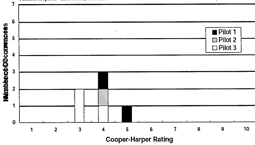
Figure D15 Horizontal Offset Landing Cooper-Harper Ratings - H2AIN
