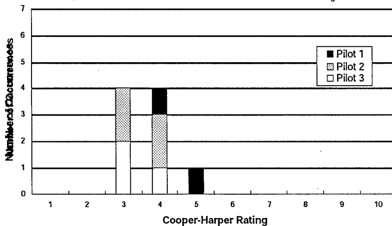
Figure D11 Horizontal Offset Landing Cooper-Harper Ratings - H2INI
