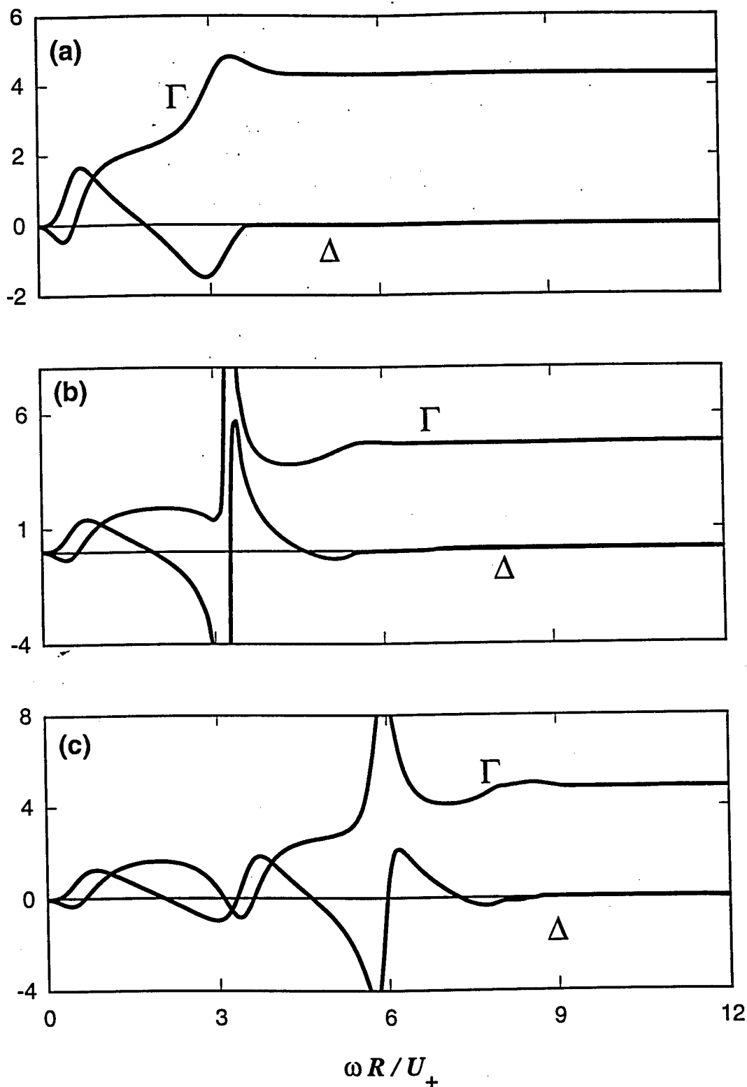
Figure 2. Normalized real and imaginary parts \mathcal{K}(\omega)/2R = \Gamma(\omega) - i\Delta(\omega) of the conductivity of a circular aperture for (a) U_-/U_+ = 0 , (b) 0.2 , (c) 0.4 , (d) 0.6 , (e) 0.8 , (f) 1.0 .
