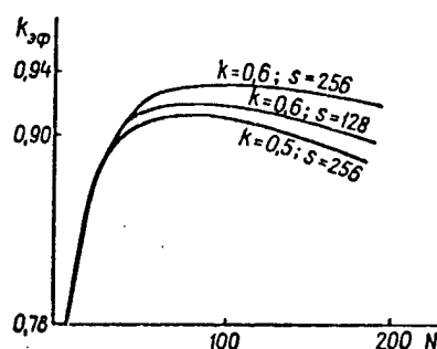
Figure 2. Dependence of k_{\exists\phi}(N)
