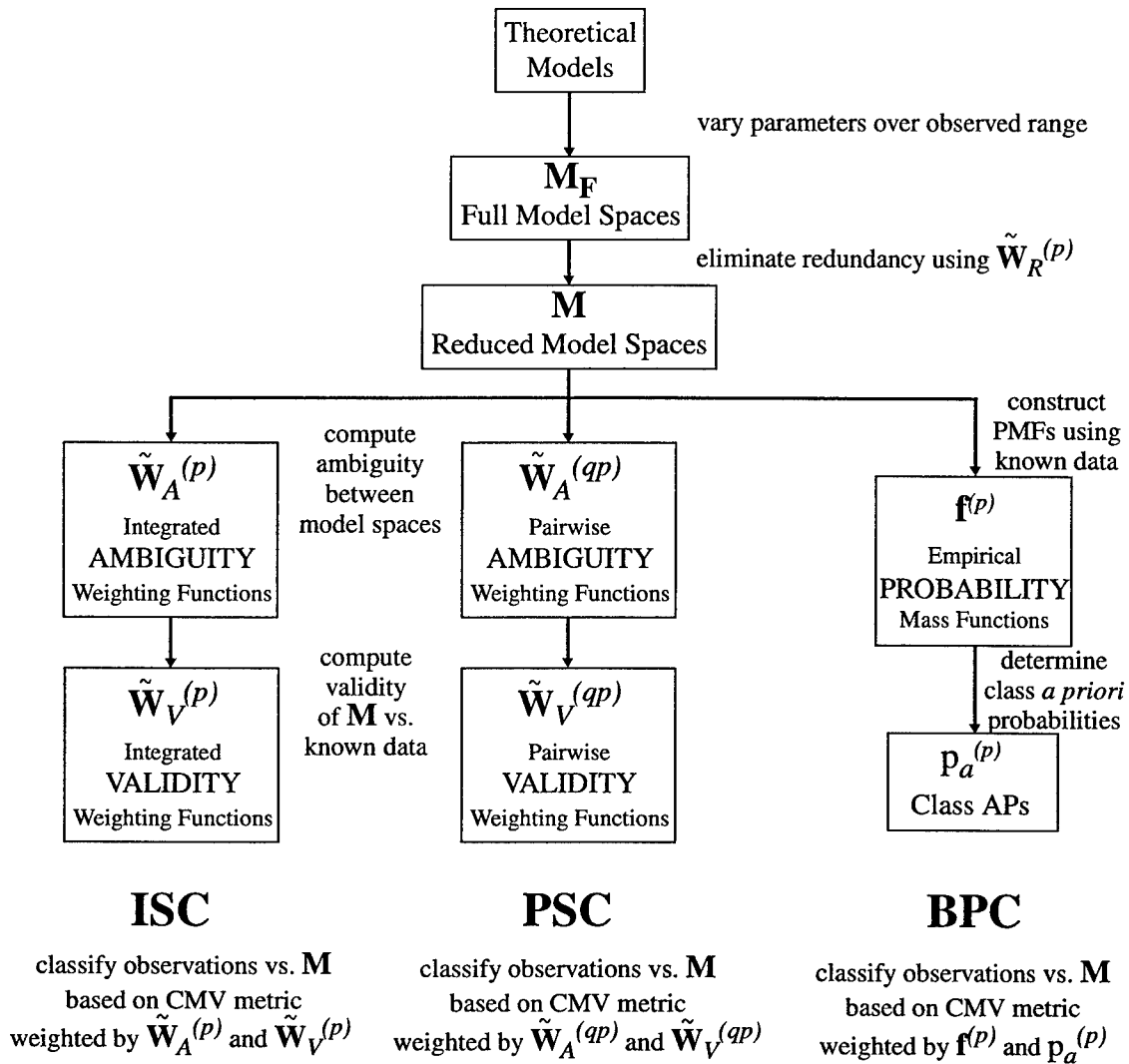
Figure 4-3 Diagram of the CMVC approach. Model spaces for each class p are constructed based on the theoretical models, and redundancy is eliminated by applying the redundancy weighting function \tilde{W}_R^{(p)} . Ambiguity and validity are accounted for via ambiguity and validity weighting functions, \tilde{W}_A^{(p)} and \tilde{W}_V^{(p)} in the ISC (Integrated Score Classifier), \tilde{W}_A^{(qp)} and \tilde{W}_V^{(qp)} in the PSC (Pairwise Score Classifier), or the probability mass function f^{(p)} and the a priori probabilities p_a^{(p)} in the BPC (Bayesian Probability Classifier). The CMV metric for classification is given in (EQ 4.2).
