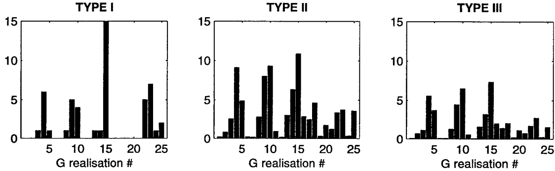
Figure 4-8 Class-support TYPE I , TYPE II and TYPE III PMFs f^{(3)} , computed using (EQ 4.12), for the simplified model space G (a first-order representation of the model space for the GB scattering class). For TYPE II and TYPE III f, t_f = 0.5 \max(C_{f_{ij}}^{(p)}) . The validation set V^{(3)} contains 50 observed echo spectra from a single siphonophore ( Agalma okeni ).
