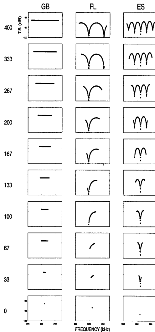
Figure 2-11 Effect of bandwidth reduction on the magnitude of the Fourier transform of clean signals (top row, plotted as TS in dB). For these realisations, the band-pass filter is centered at ~550 kHz. Remaining bandwidth (value to left of rows, in kHz) decreases down the columns.
