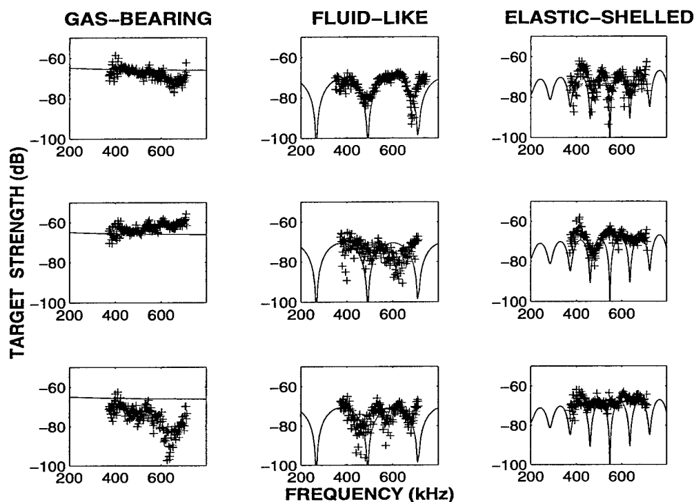
Figure 3-1 Echo spectra of a selected set of experimental data plotted with theoretical models for each class. GB model: spherical gas bubble plus fluid-like tissue model (EQ 3.1) with echo from gas dominating scattering; GB data: single siphonophore Agalma okeni (Animal 93-18). FL model: ray summation including two rays, one from front interface, one from back interface (EQ 3.4); FL data: decapod shrimp Palaemonetes vulgaris (top) and euphausiid Meganyctiphanes norvegica , (Animal 93-33). ES model: ray summation including only first partial circumnavigation of Lamb wave (EQ 3.6); ES data: two pteropods Limacina retroversa (Animals 93-29 (top) and 93-30).
