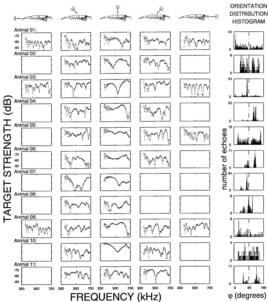
Figure 5-10 Examples of echo spectra received from 11 krill (Animals 01 through 11, rows) at 5 angles of orientation, with acoustic wave incident at \phi \approx 0^\circ, 45^\circ, 90^\circ, 135^\circ, 180^\circ (\pm 15^\circ) (first 5 columns); empty plots indicate that the animal did not assume that orientation during the experiment. Histogram of orientation distribution for each animal during insonification shown at right.
