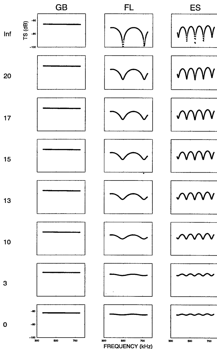
Figure 2-9 Effect of addition of ensemble-averaged noise to clean signals (top row) on the magnitude of the Fourier transform (plotted as TS in dB). SNR (in dB) decreases down the columns (value at left).
