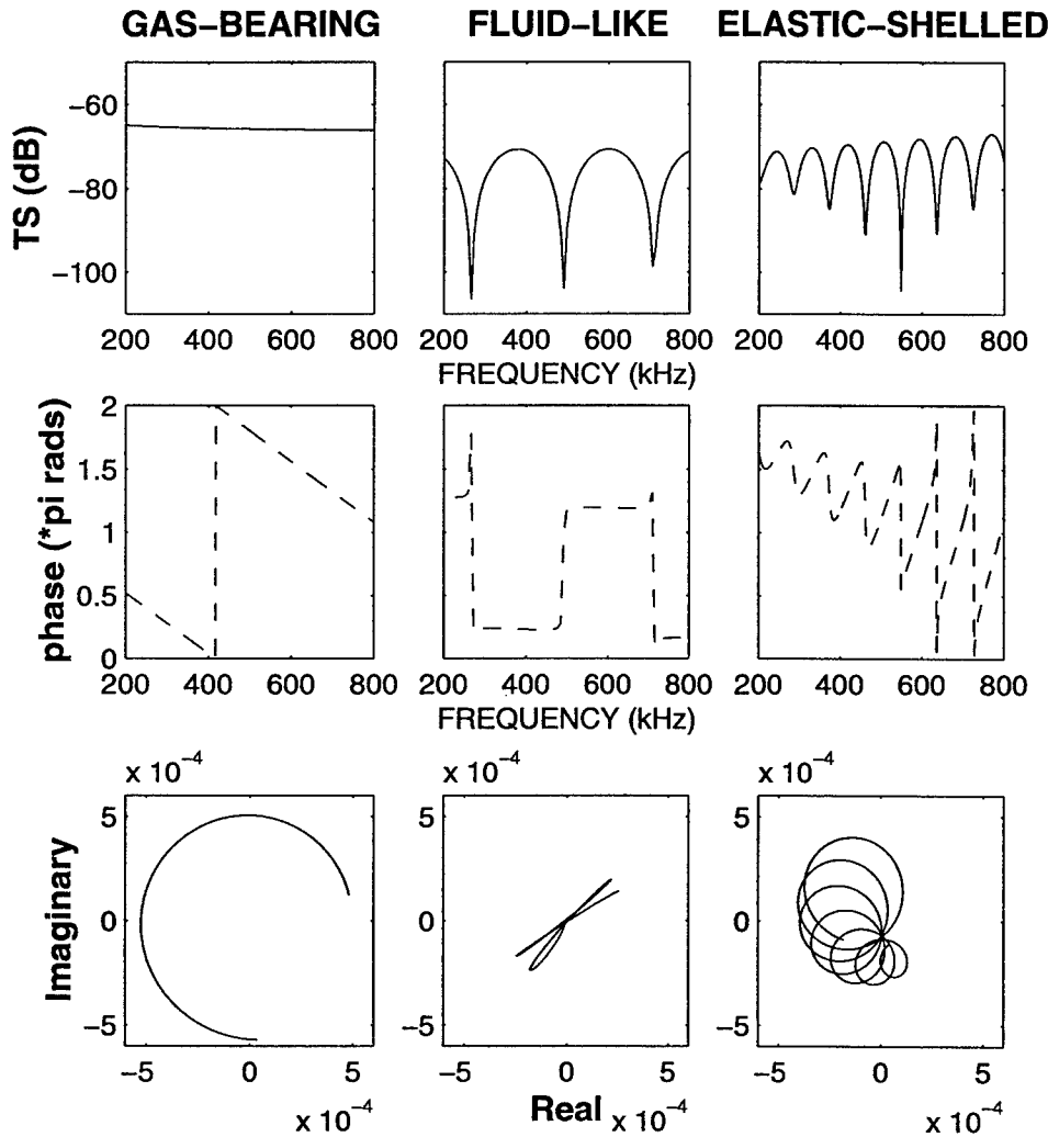
Figure 2-6 Characteristics of the theoretical-model-generated clean signals. Top row is |S(\omega)| , the magnitude of the Fourier transform of s(t) , plotted as target strength (TS) in dB. Second row is the phase of S(\omega) , computed as \tan^{-1}(\text{Re}[S(\omega)]/\text{Im}[S(\omega)]) . Bottom row is the phasor diagram, showing plot of \text{Im}[S(\omega)] vs. \text{Re}[S(\omega)] over the frequency band 200 kHz - 800 kHz. Theoretical models plotted above are explicitly described in (EQ 3.1) with b_j = 0 (GB), (EQ 3.2) with N = 2 (FL) and (EQ 3.5) with the series truncated to include only the first partial circumnavigation (ES).
