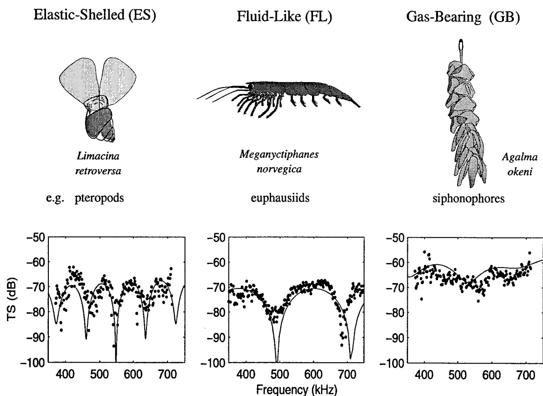
Figure 4-1 Representative zooplankton from the three scattering classes. Echoes collected from broadband insonifications of animals in each class are plotted (points) together with theoretical models (solid line) that describe the acoustic scattering from these three classes of animals under certain conditions. Details of these models are included in Stanton et al. (1996).
