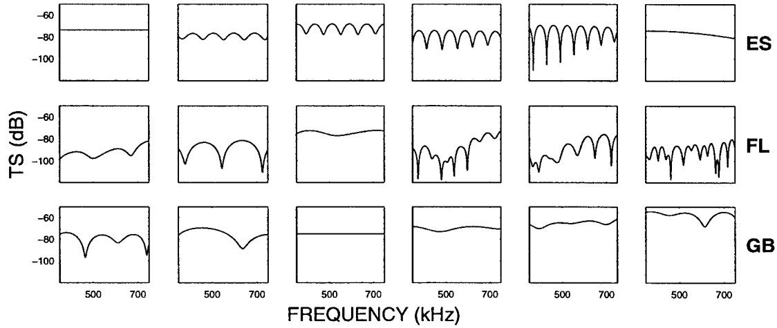
Figure 4-9 Selected examples of model realisations from the three model spaces ES (top row), FL (second row) and GB (bottom row) as generated by varying the parameters of the theoretical scattering models. The 600 realisations in the full ES model space \mathbf{M}_F^{(1)} were generated using (EQ 4.13) with c/c_l = 8 , \Re = 0.84 , varying F_{spec} and F_l between 0 and 1, and \bar{a} between 0.5 and 1 mm. \mathbf{M}_F^{(2)} is composed of 700 FL realisations, generated using (EQ 4.14) with g = 1.0357 and h = 1.0279 , varying \beta_{tilt} between 0 and 180^\circ , a between 1 and 3 mm, and using 5 different shapes (digitised from actual video images of euphausiids). The 800 realisations in the full GB model space \mathbf{M}_F^{(3)} were generated using (EQ 4.15) with g = 0.0012 , h = 0.22 , and N = 6 , and varying F_{tiss} between 0 and 1, a between 0 and 1.75 mm, and \bar{\epsilon}_j between \min(\lambda)/(N - 1) and \max(\lambda)/(N - 1) .
