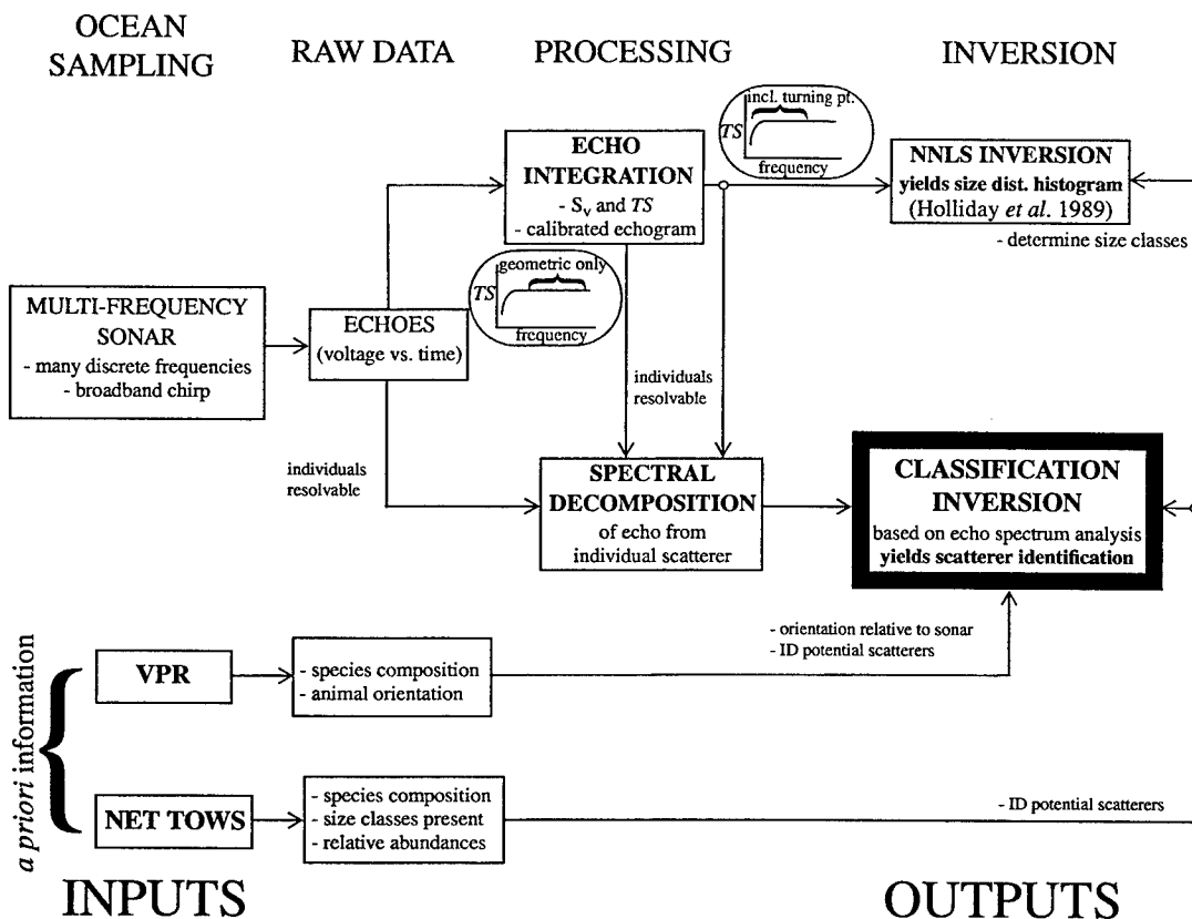
Figure 4-2 Approaches to solving the inverse problem for zooplankton. If frequency sampling brackets the turning point between the Rayleigh and geometric regimes, a non-negative least-squares (NNLS) inversion can be used to estimate the size distribution of a zooplankton assemblage. If echoes from individual zooplankton are resolvable and frequency sampling is virtually continuous, a CLASSIFICATION INVERSION can be performed to categorise individual zooplankton according to their frequency-dependent scattering characteristics. A priori information may be obtained via simultaneous net samples and/or VPR (Video Plankton Recorder) samples.
