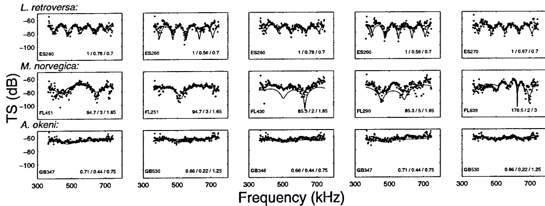
Figure 4-12 Selected examples of PSC-inverted best match echo classifications for five observations each of a pteropod L. retroversa ( \bar{a} \approx 0.75 mm, top), a euphausiid M. norvegica ( a \approx 1.5 - 2 mm, middle), and a siphonophore A. okeni ( a \approx 0.6 - 1 mm, bottom), from the high-quality subset of 1993 data. Observations (points) plotted together with best match model realisations (solid line); best match scattering class and model realisation number shown at bottom left, parameter inversions given at bottom right (ES: F_{spec}/F_l/\bar{a} ; FL: \beta_{tilt}/shape\#/a ; GB: F_{tiss}/\epsilon_j/a ; \bar{a} and a in mm, \beta_{tilt} in degrees). PSC implemented including both ambiguity and validity weightings ( \bar{W}_A , \bar{W}_V ). Validation set V included half of the 1550 1993 observations. Classification threshold t was adjusted to include all CMV within the 3 dB-down range: t = 0.5\max(C_{ij}^{(p)}) .
