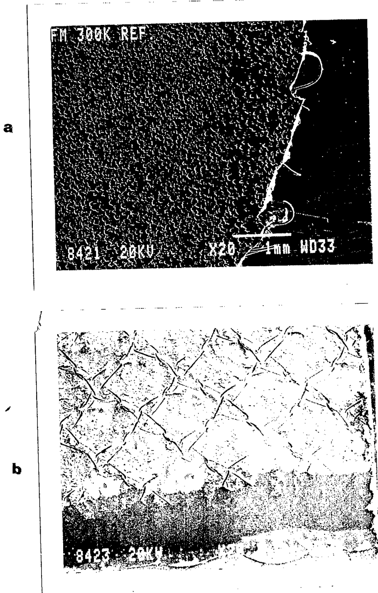
Fig. 3.4: SEM photographs of the surface failure morphology of SLS joints (table 3.1) with adhesive FM3002K, primer BR127.a: without treatment. b: anodized adherends.
