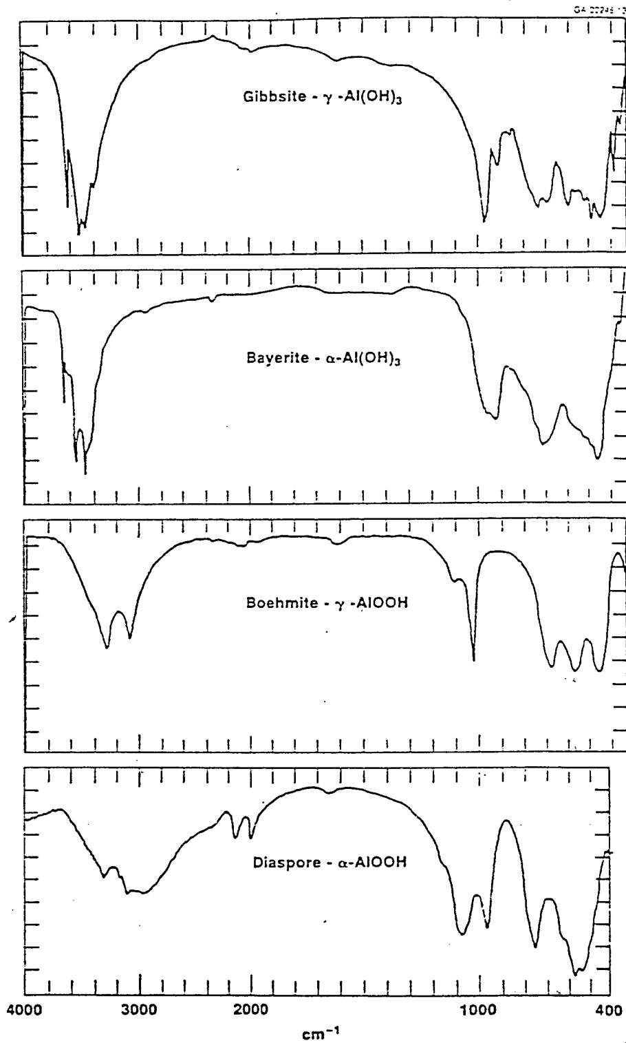
Fig.3.16: Infra Red spectra of various aluminum hydroxide(4).
