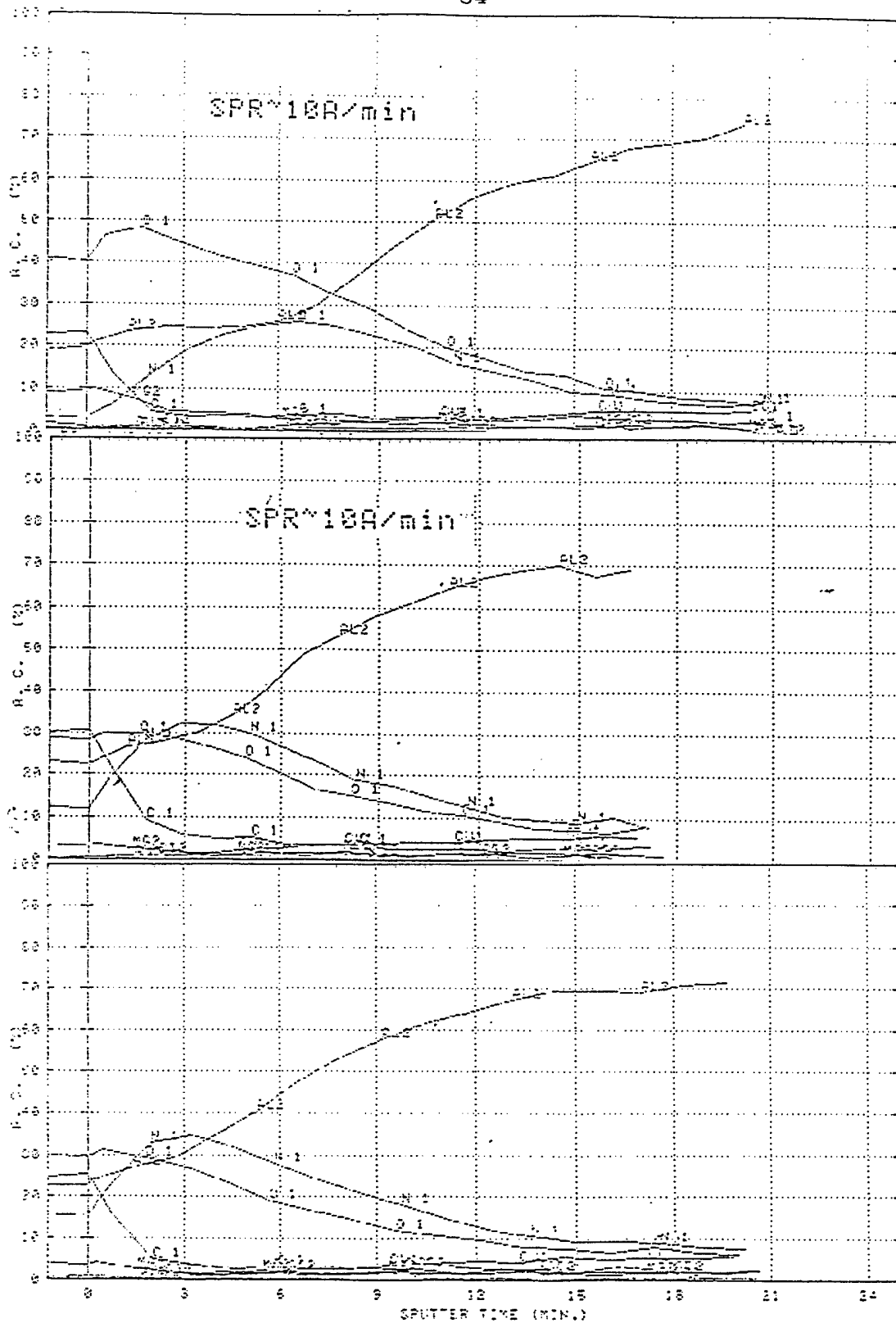
Fig. 3.22: Auger depth profile of Al irradiated at laser energy of 2.7 \text{ J/p} \cdot \text{cm}^2 . a. 10 pulses b. 50 pulses. c. 100 pulses.
