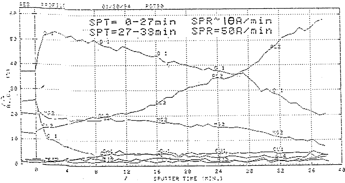
Fig. 3.19: Auger depth profile of Al irradiated at laser energy of 0.18\text{J/p}\cdot\text{cm}^2 . a. 2000 pulses b. 5000 pulses.
