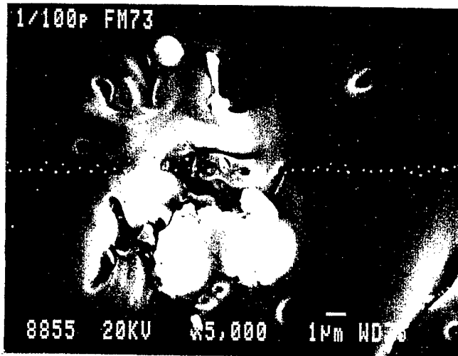
Fig. 3.13: SEM photographs of the surface failure morphology of SLS joints (table 3.4) with adhesive FM73, fresh primer BR127, laser energy 1\text{j/p}\cdot\text{cm}^2 , 100 pulses.
