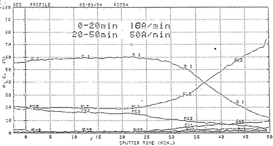
Fig. 3.20: Auger depth profile of Al irradiated at laser energy of 0.57\text{J/p}\cdot\text{cm}^2 . a.10 pulses b.1000 pulses.
