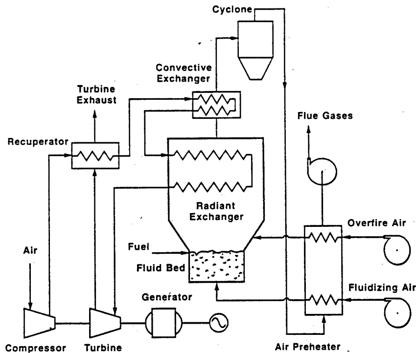
FIGURE 1. ENERGEIO's AGRIPOWER process schematic
