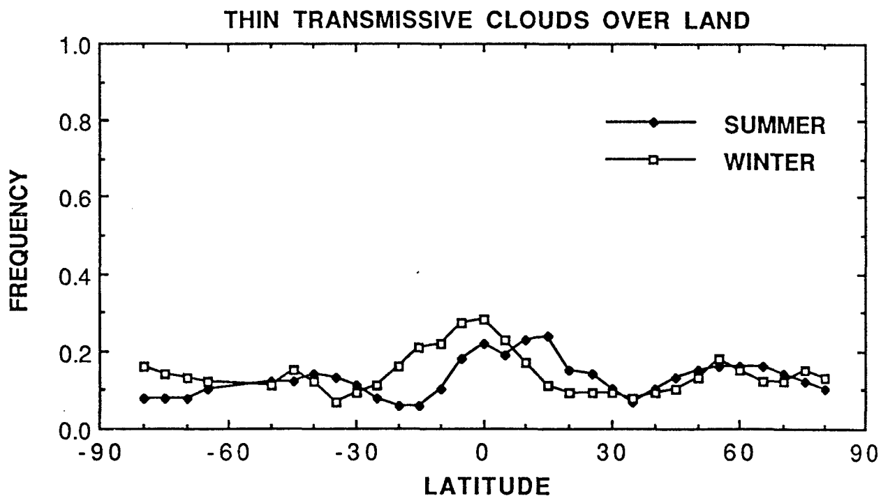
Figure 5: (a) The frequency of thin transmissive ( N_e less than .5) over ocean as a function of latitude for the summers (June, July, August) of 1989-90 and winters (December, January, February) 89-91 expressed as a fraction of all satellite observations, clear and cloudy combined. (b) The same over land.
