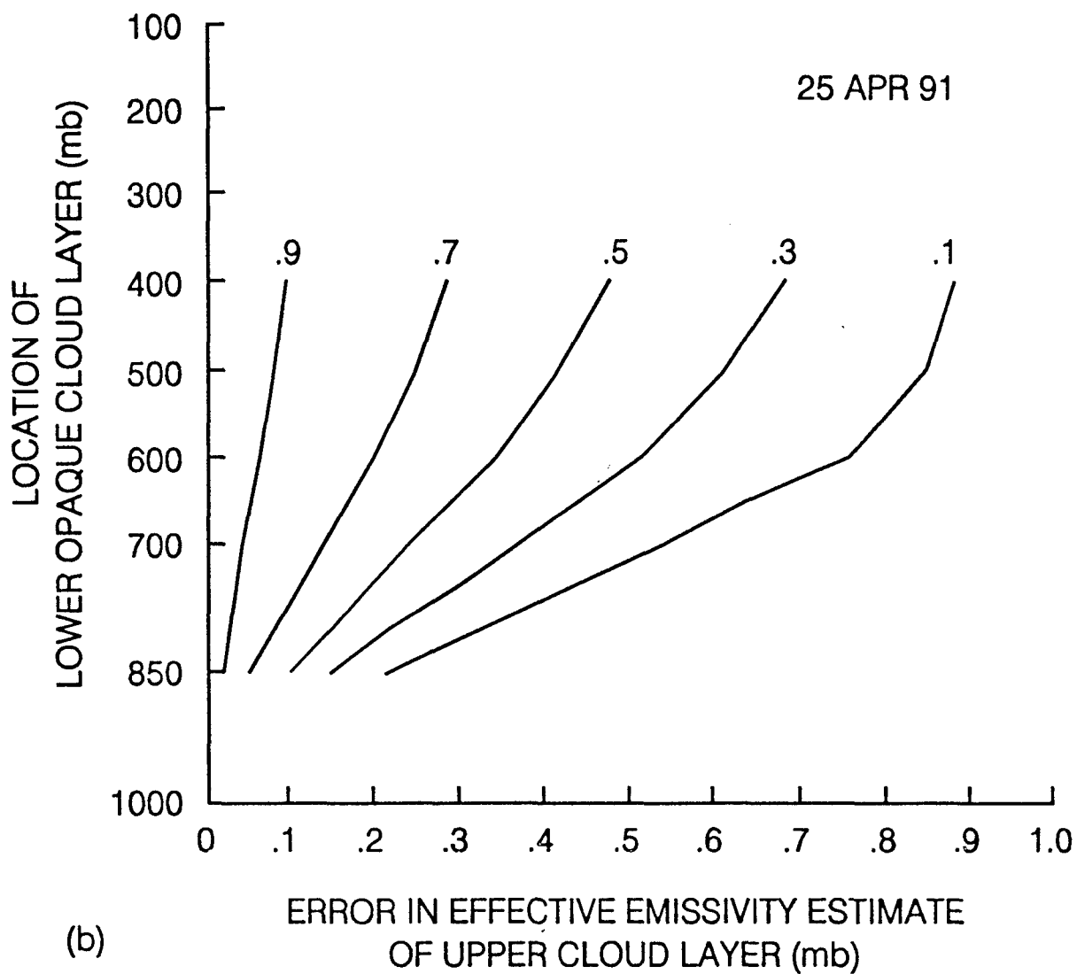
Figure 7: (b) The errors in effective emissivity (from the original solution of N_e ) as a function of height of the underlying opaque cloud layer.
