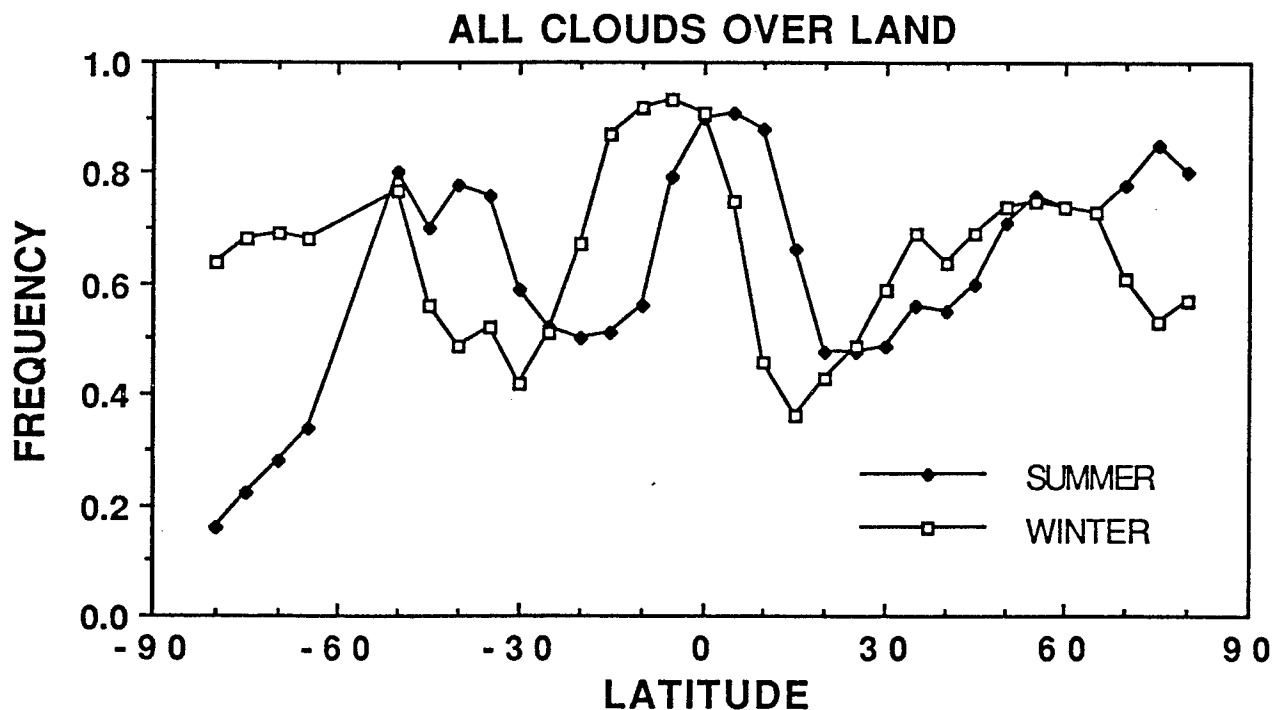
Figure 1: (a) The frequency of all clouds over ocean as a function of latitude for the summers (June, July, August) of 1989-90 and winters (December, January, February) 89-91 expressed as a fraction of all satellite observations, clear and cloudy combined. (b) The same over land.
