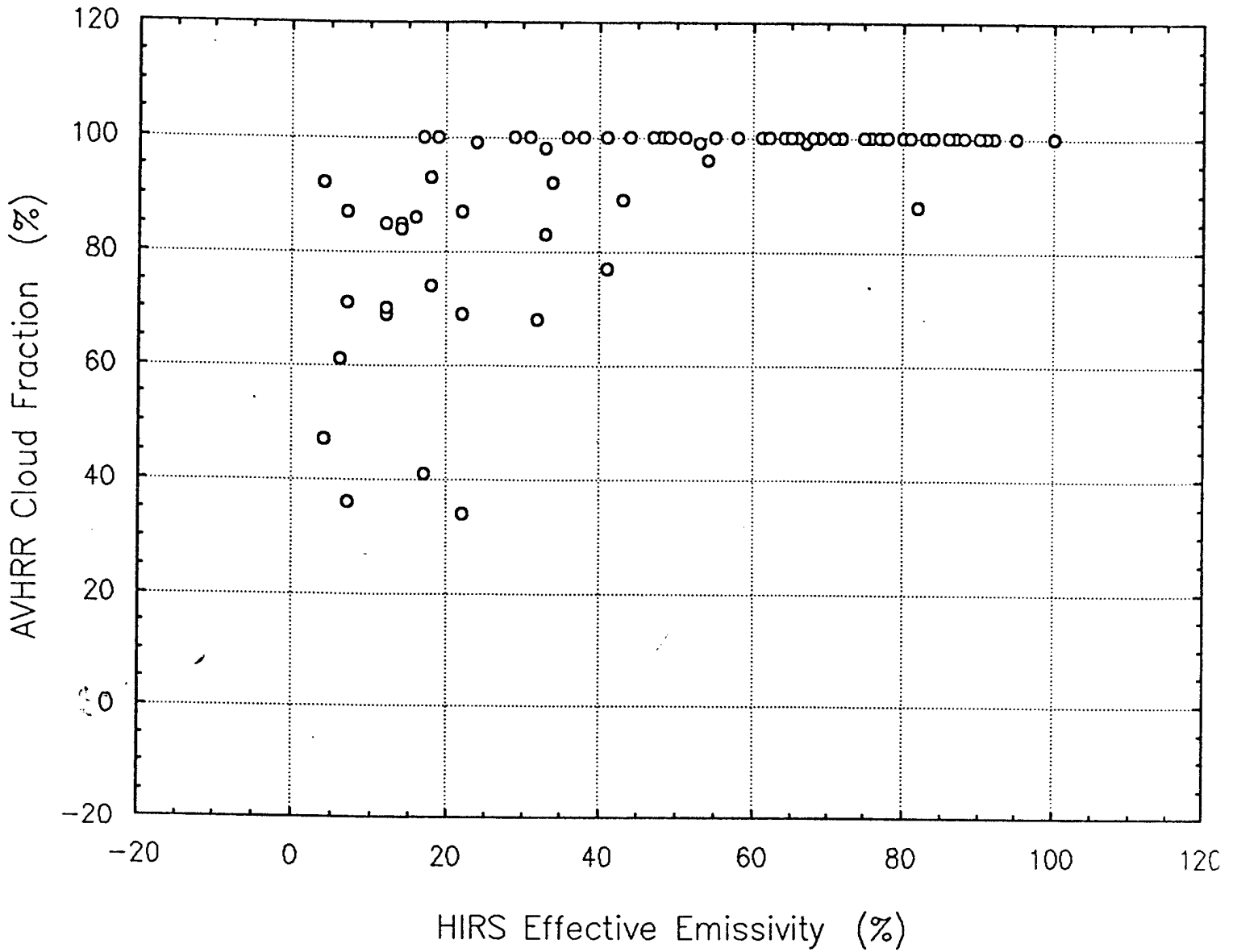
Figure 8: Plot of AVHRR cloud fraction N_A (determined from infrared brightness temperature comparison to surface temperature within a collocated HIRS FOV) versus the HIRS CO_2 slicing effective emissivity N_{eH} for 6 and 12 January 1994 over the Atlantic Ocean.
