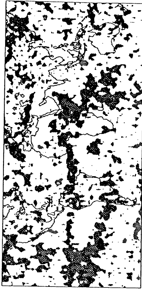
June through August, 1991-1990 difference
