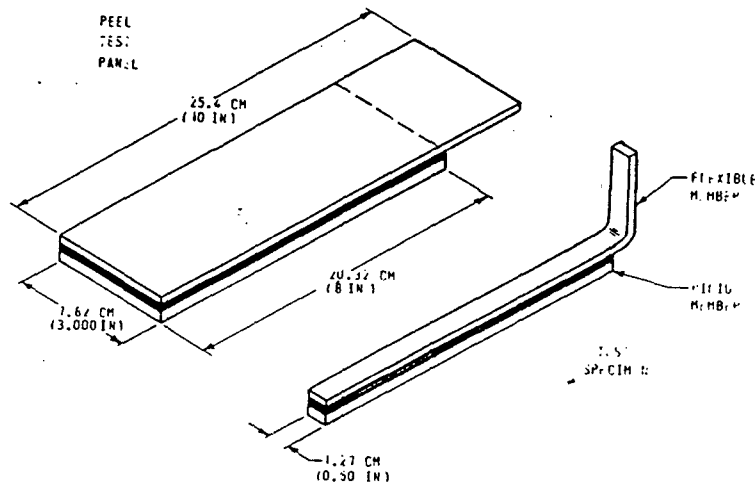
Fig. 2: Peel tests' adherends
