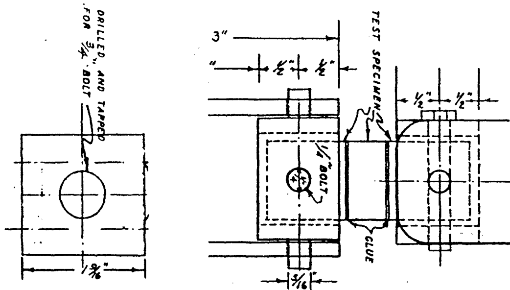
Fig. 2: Peel tests' adherends
