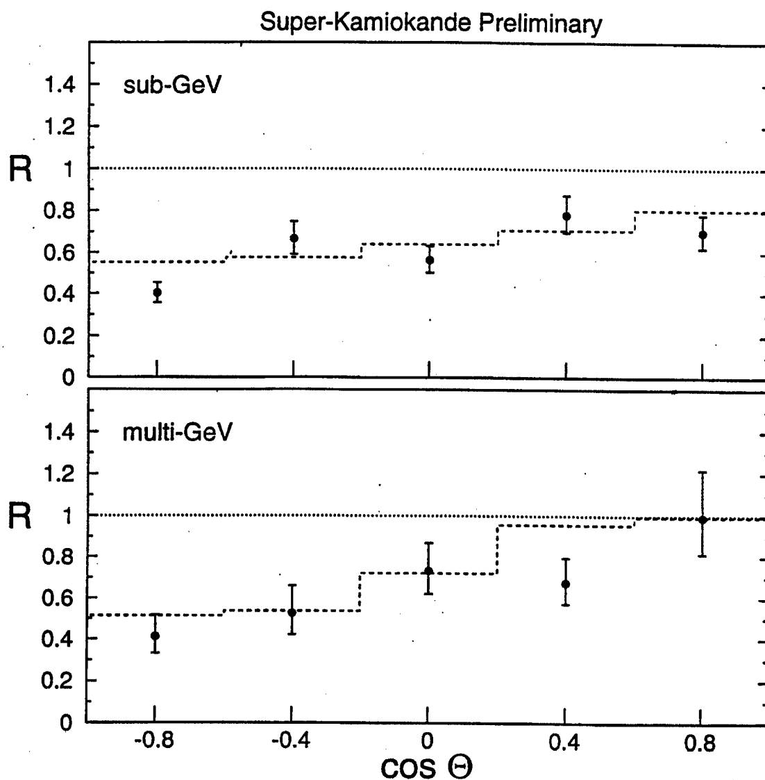
Figure 4.6 Currently, about 15% of university-based experimental physicists in the U.S. high-energy physics program probe the properties of elementary particles using non-accelerator experiments. In the Super-Kamiokande detector, for example, neutrinos produced in cosmic-ray interactions in the earth's atmosphere show indications of neutrino oscillations. The ratio of observed muon- to electron-neutrino interactions, divided by the ratio expected from Monte Carlo simulation assuming no neutrino oscillations, is shown as a function of the zenith angle ( \cos \theta = 1 corresponds to neutrinos coming from above). The upper figure is for neutrinos below 1 GeV, and the lower figure is for neutrinos above 1 GeV. The data are inconsistent with R = 1 (no neutrino oscillations). The dashed histogram shows a sample prediction for \nu_\mu \rightarrow \nu_\pi oscillations with \sin^2 2\theta = 1 ( \theta is the mixing angle) and \Delta m^2 = 0.005 \text{ eV}^2 .
