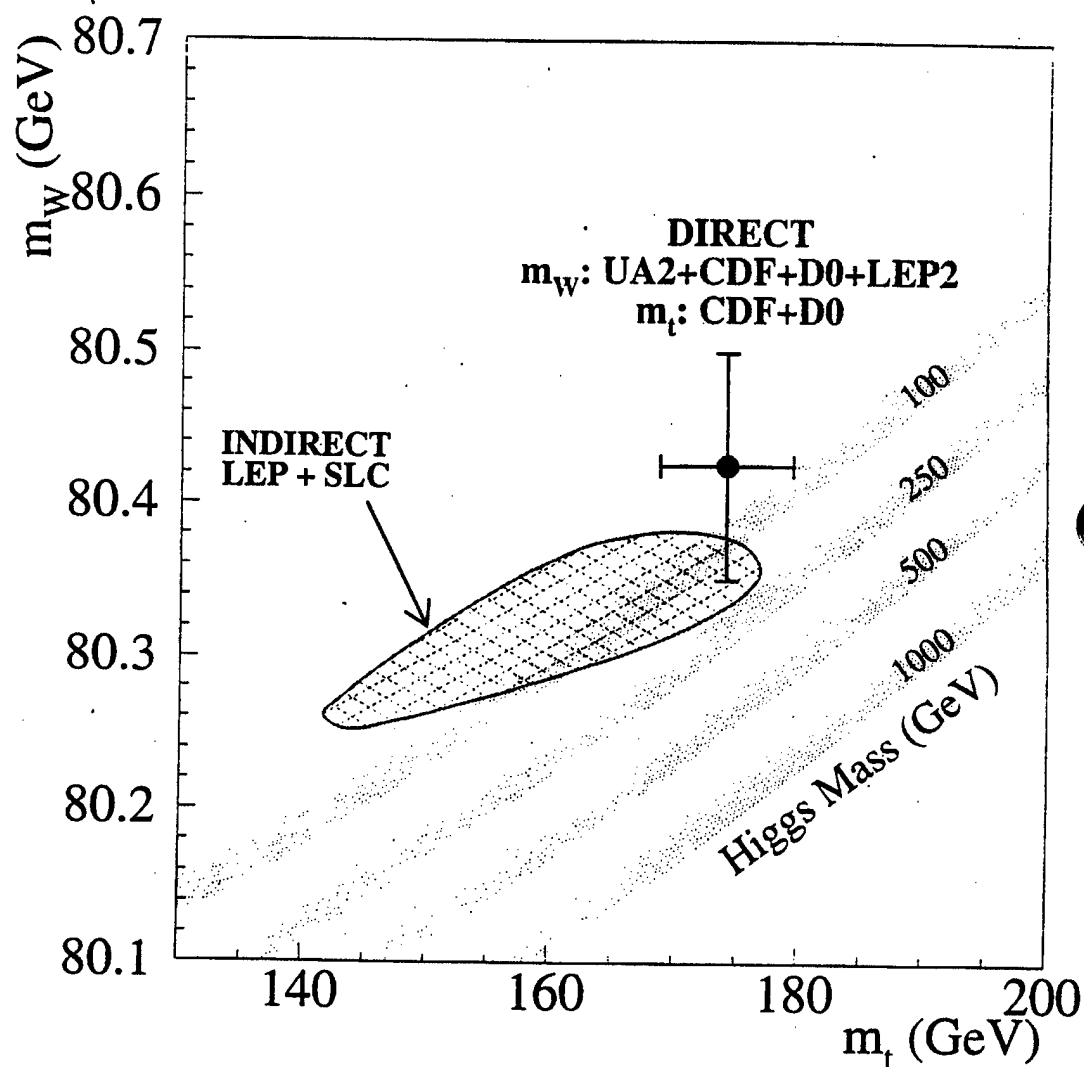
Figure 4.1 The Tevatron collider at Fermilab is the only accelerator in the world with sufficient energy to allow direct measurement of both the mass of the W boson and the mass of the top quark. The data point is the average of the direct experimental measurement of these masses, including data from Fermilab and from CERN. This information precisely tests the Standard Model and guides the search for the mechanism of electroweak-symmetry breaking, as shown by the shaded bands that give the predictions for specific Higgs boson masses. The cross-hatched area shows the region allowed at the 68% confidence level by the many precision measurements on Z boson properties made by experiments at CERN and SLAC.
