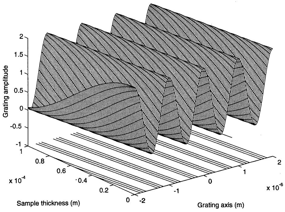
Fig. 3-4 Volume grating profile for 0.5^\circ \delta -angle.
