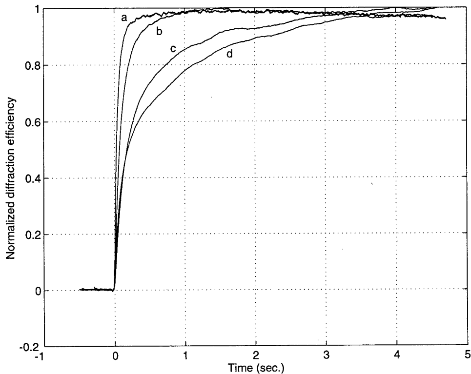
Fig. 5-5 Rise time behaviors of four BR films for a similar write intensity.
