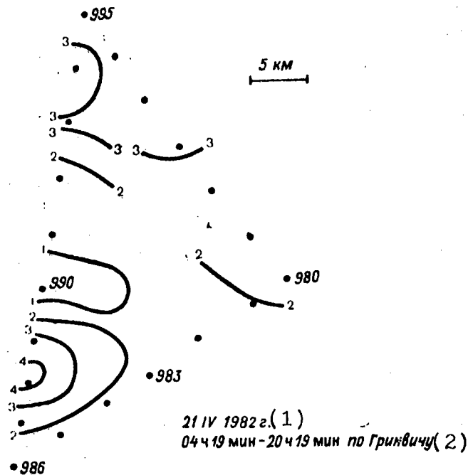
Figure 4.1. Horizontal Distribution of Chlorophyll a and Phaeopigments at a Depth of 0 m, mg/m 3
