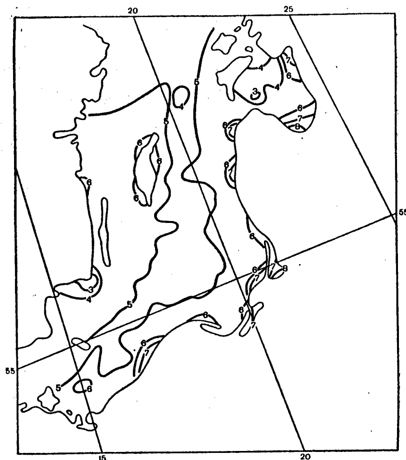
Figure 5.7. Surface Temperature of the Baltic Sea (°C) According to Data from the No 5 Meteor-2 Satellite. 25 April 1982, 1100 GMT
