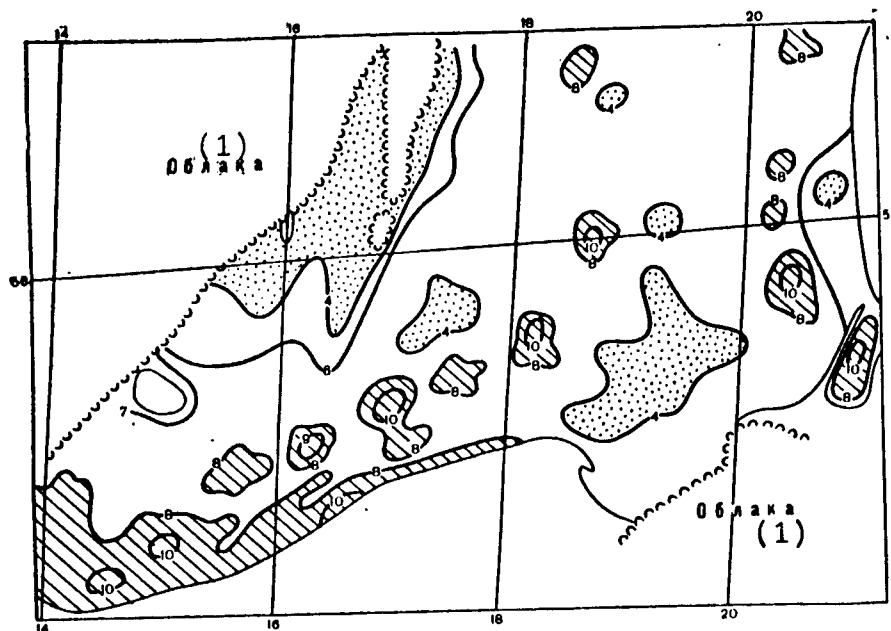
Figure 5.8. Surface Temperature of the Baltic Sea ( ^{\circ} C) According to NOAA-6 Satellite Data. 23 April 1982. Projection Close to the Projection of the Satellite Photograph
