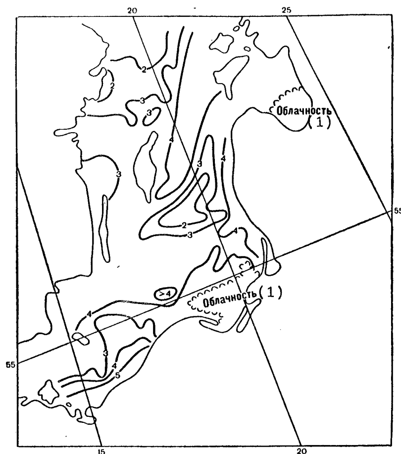
Figure 5.5. Surface Temperature of the Baltic Sea ( ^{\circ}\text{C} ) According to Data from the No 5 Meteor-2 Satellite. 25 April 1982, 0100 GMT
