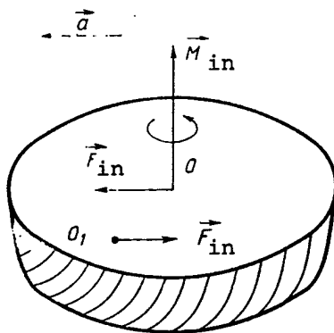
Figure 3. Possibility of OM twisting when the center of "rotation" and center of mass do not coincide under the effect of linear acceleration
