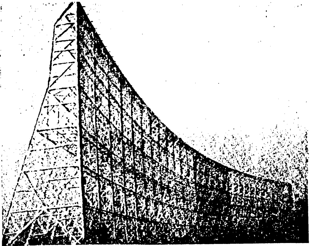
Main Mirror of Large Radiotele- scope at Nancay (France). The Radio- telescope consists of two reflectors and the size of the main mirror is 300 by 35 meters
