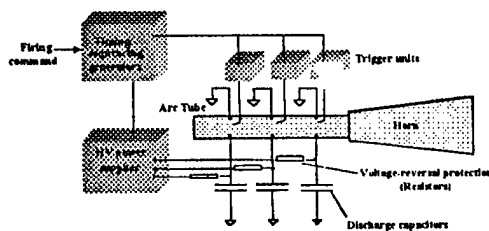
Figure 1. Block diagram of SADAG.
