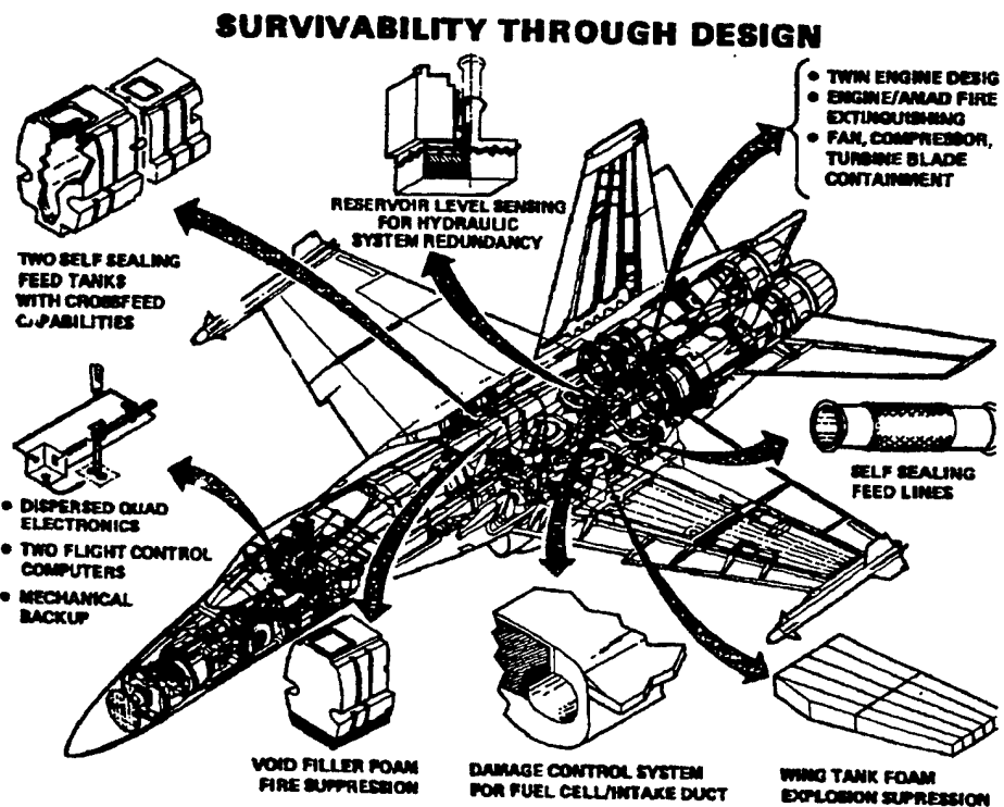
Fig. 2 Some Vulnerability Reduction Features on the F/A-18A (Courtesy of McDonnell Aerospace)
