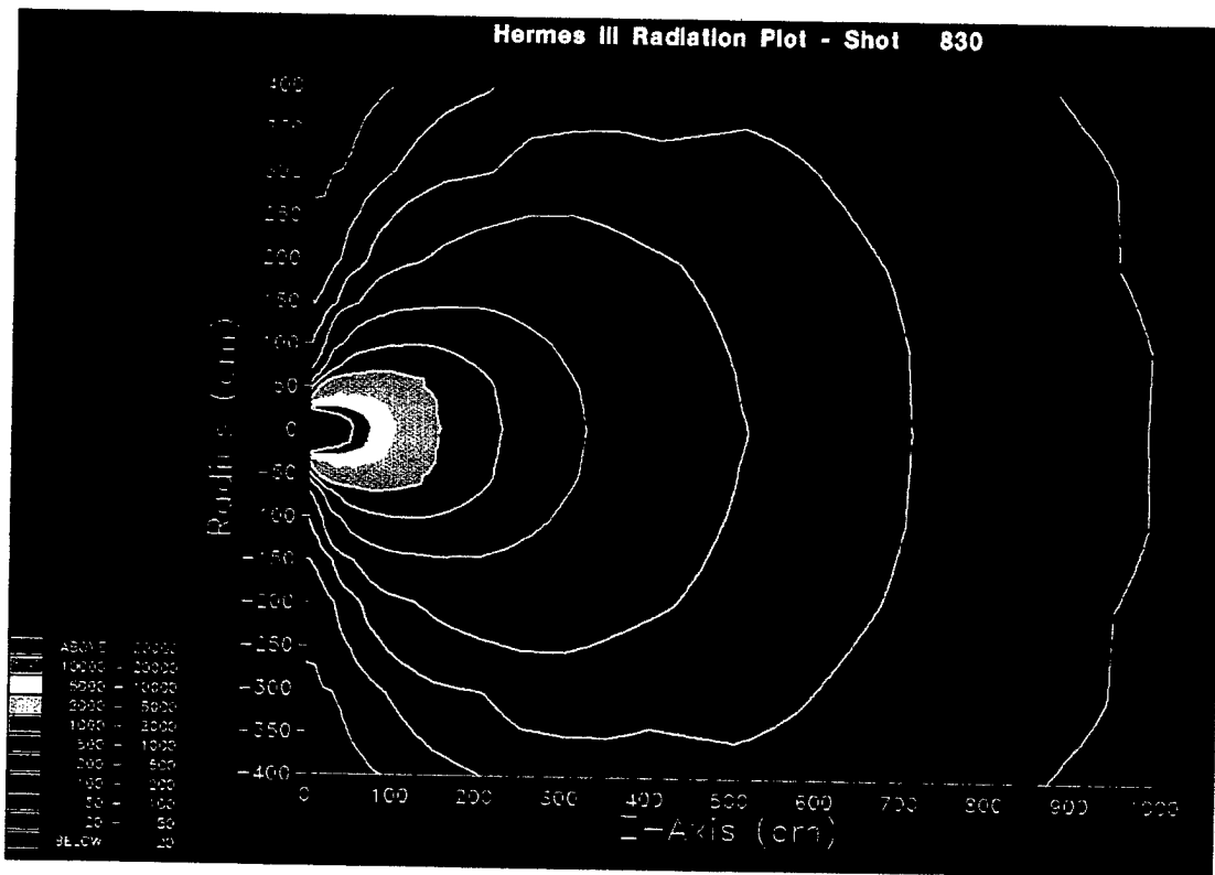
Fig. 6a - Isodose Contour Map for Planar-Anode Diode, 53 cm AK GAP
