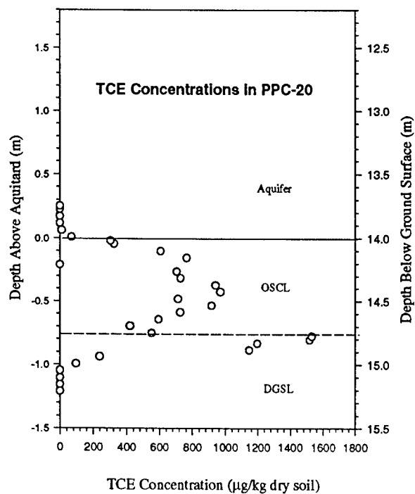
Figure 11. PPC Core Sampling Results for TCE in September 1997
