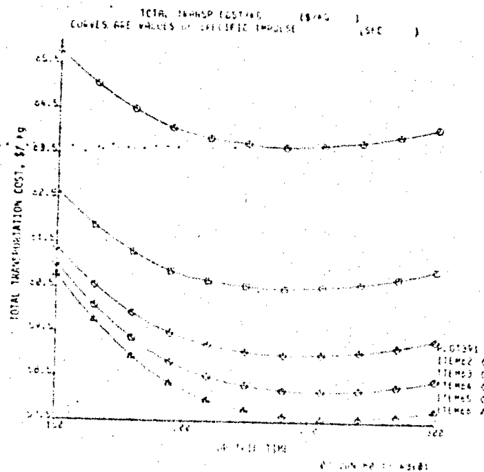
Figure 4.5-5. MPD EOTV: 3 Mil CG, Annealing, No Thermal/Startup (EOTVA)
