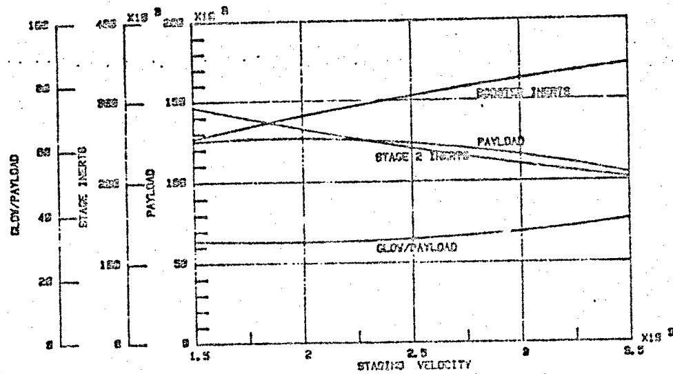
Figure 2.1-3. Series Burn-Glow = 4E6
