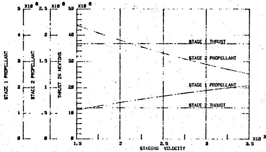
Figure 2.1-8. Parallel Burn--Glow-4E6
