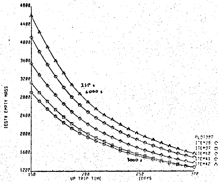
MPD EOTV with 150-micron (6-mil) cell covers, no annealing. Includes solar array thermal degradation and time delay.
