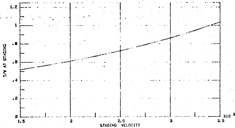
Figure 2.1-9. Parallel Burn--Glow-4E6
