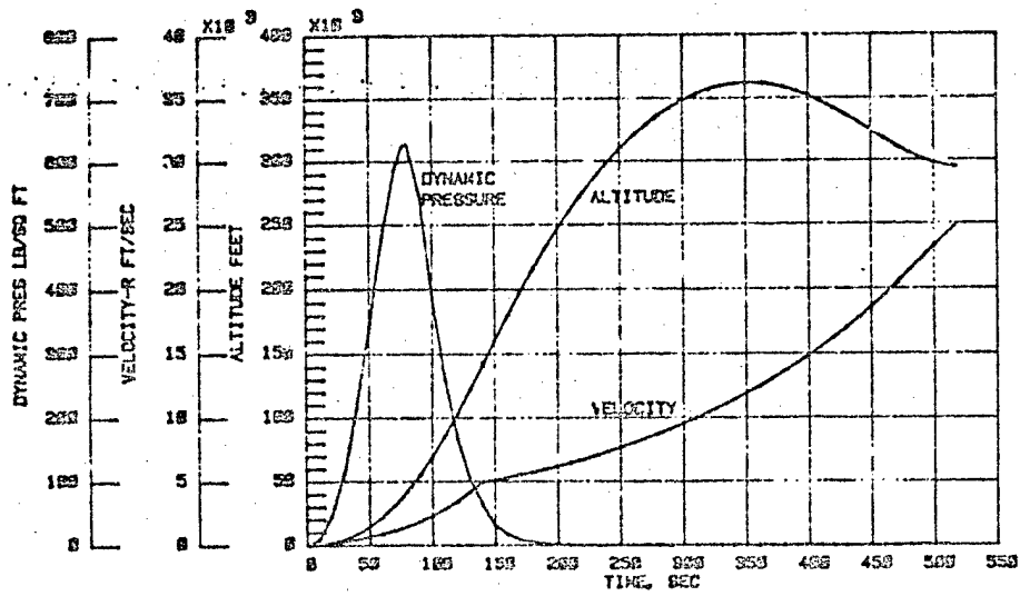
Figure 2.2-2. Small HLLV Reference Trajectory
