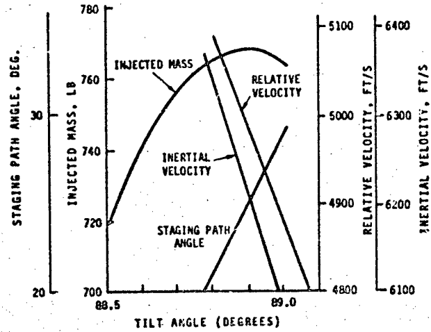
Figure 2.2-1. Staging Point Variation and Injected Mass
