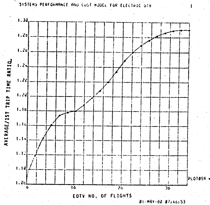
Figure 4.4-10. Systems Performance and Cost Model for Electric OTV
