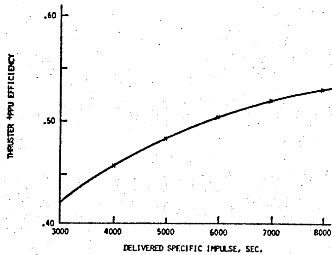
Figure 4.3-1. MPD Performance Projection
