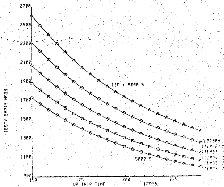
Ion engine EOTV with 150-micron (6-mil) cell covers, no annealing. No thermal degradation or time delay.
