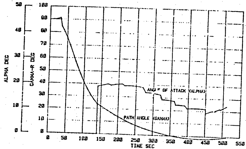
Figure 2.2-3. Small HLLV Reference Trajectory
