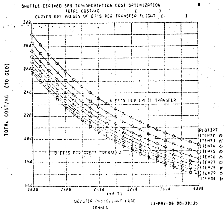
Figure 3.2-19. Shuttle-Derived SPS Transportation Cost Optimization
