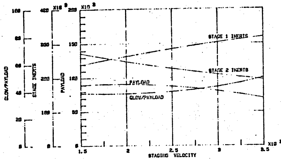
Figure 2.1-2. Series Burn-Glow = 3.5E6
