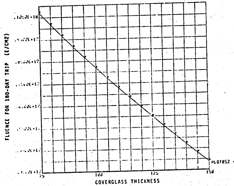
Figure 4.4-2. Systems Performance and Cost Model for Electric OTV
