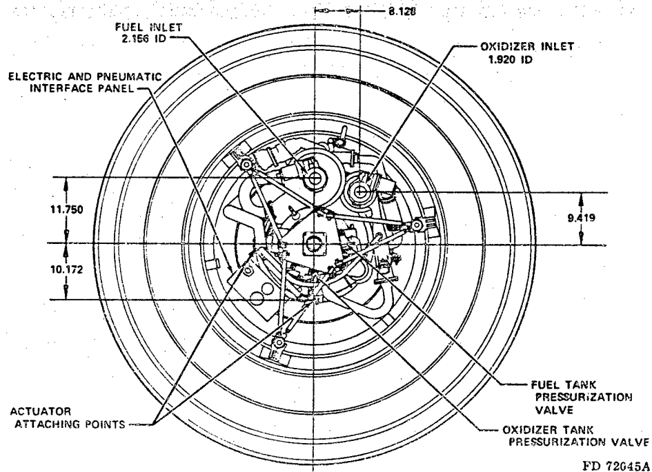
Figure 2-14. Derivative IIB Engine Installation Drawing (Sheet 2)
