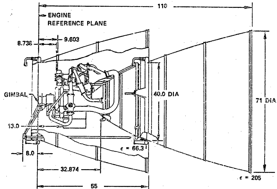
Figure 2-13. Derivative IIB Engine Installation Drawing (Sheet 1)
