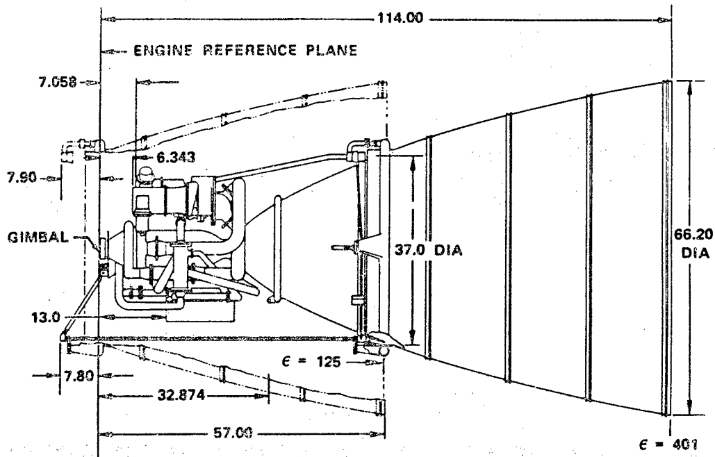
Figure 2-25. Category IV Engine Installation Drawing
