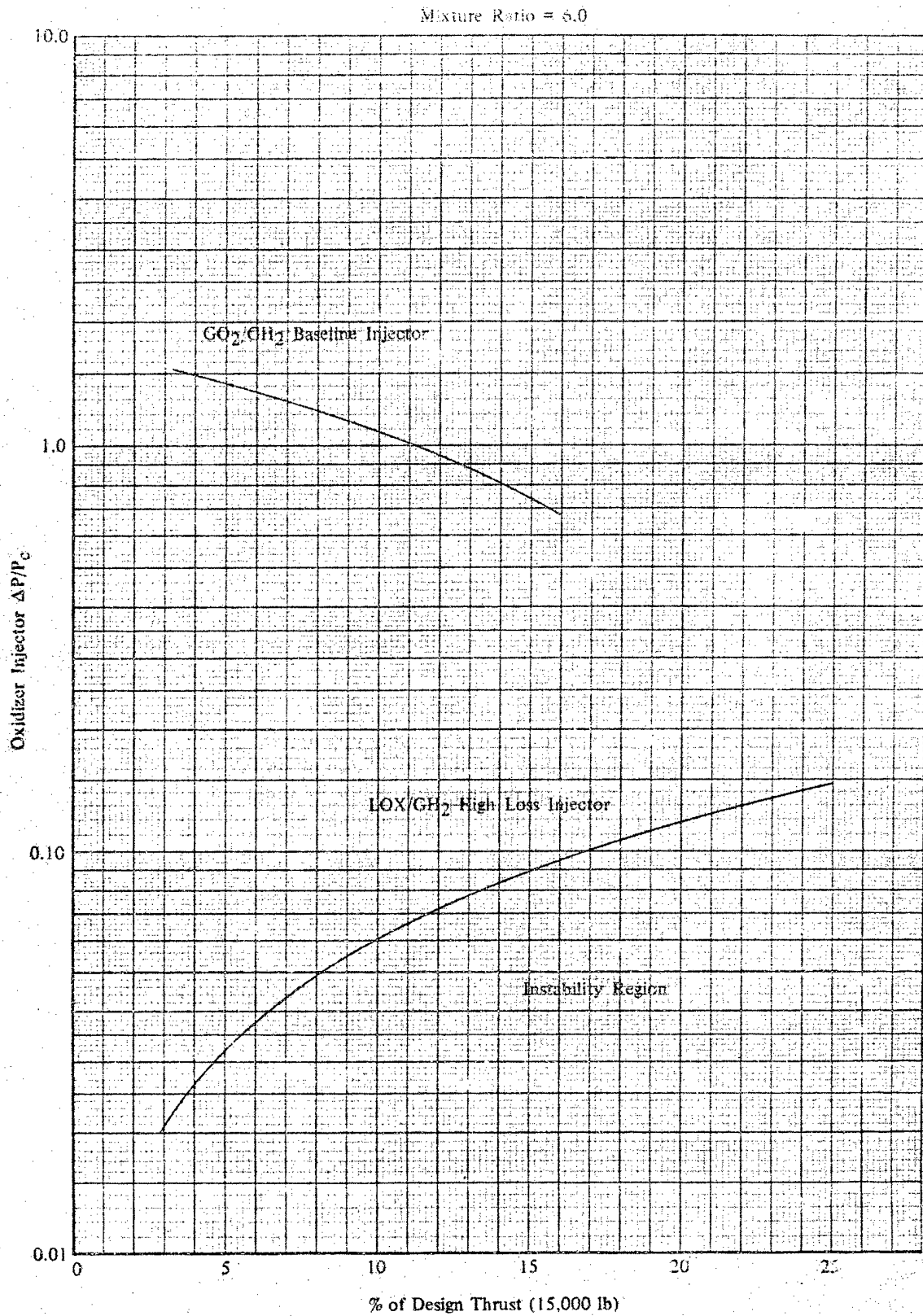
Figure 5-2. RL10 Derivative II Engines Injector Stability Characteristics
