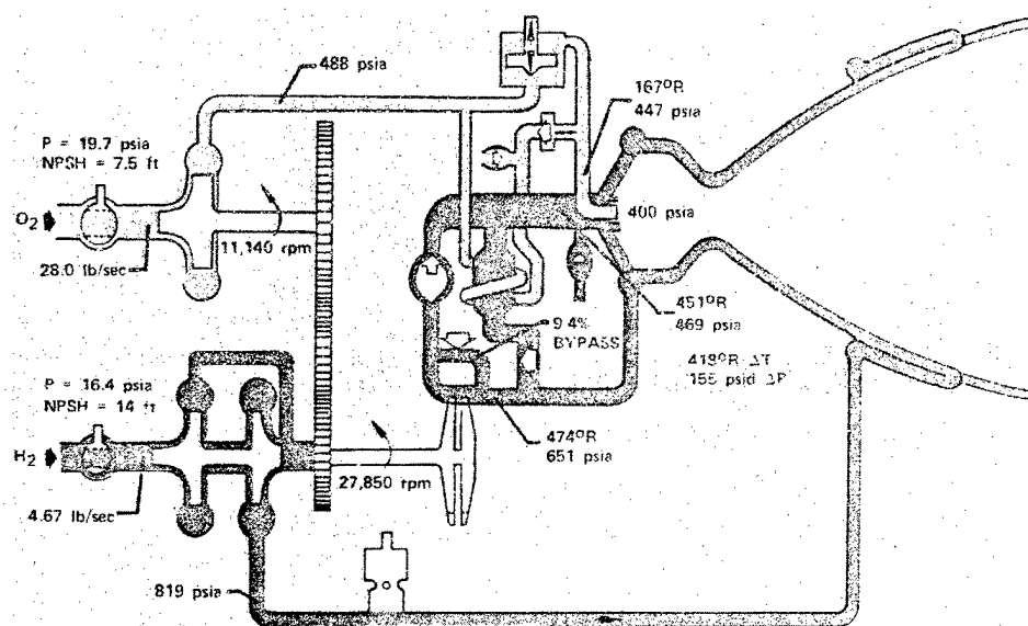
Figure 2-16. RL10 Derivative IIB Propellant Flow Schematic — Full Thrust (MR=6.0)
