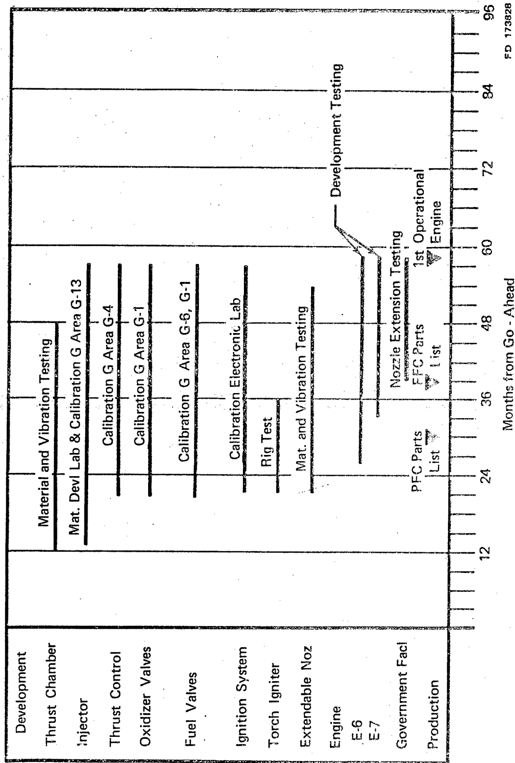
Figure 7-9. Derivative IIB - Development Program Total Test Plan
