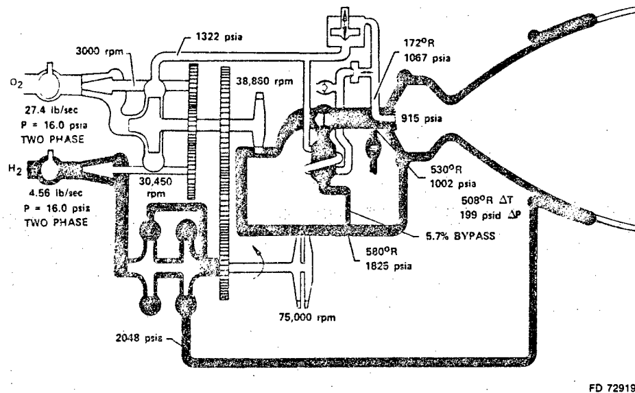
Figure 2-28. RL10 Category IV Propellant Flow Schematic — Full Thrust (MR=6.0)
