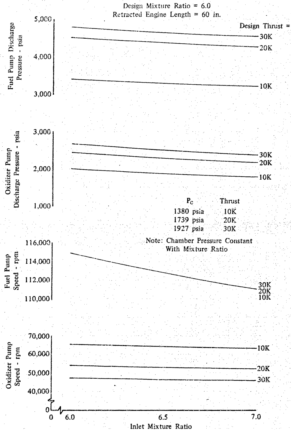
Figure 3-22. Advanced Expander Cycle Off-Design Pump Characteristics
