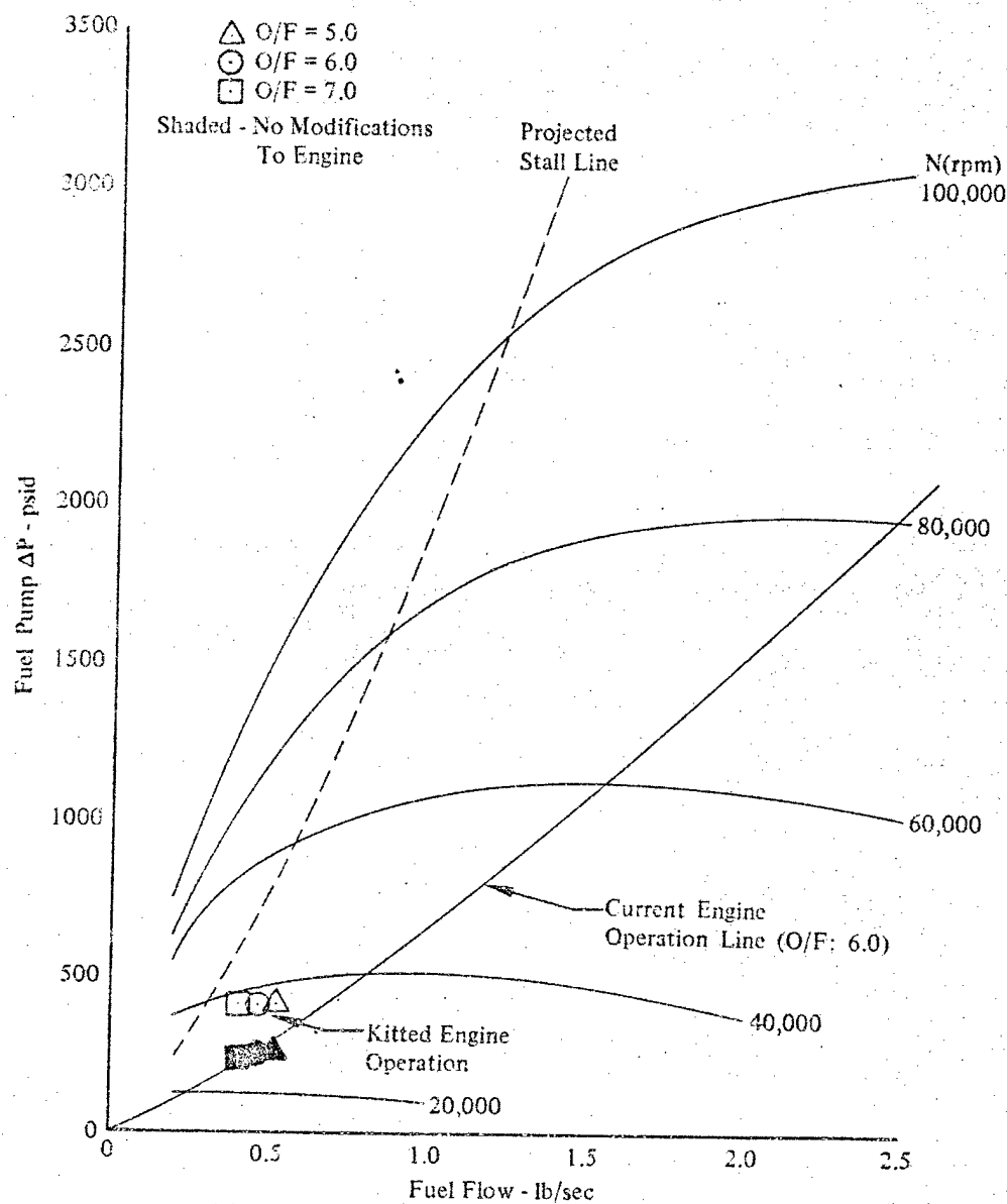
Figure 5-10. Effect of Chamber/Nozzle Kitting on Fuel Pump Operation at Low Thrust, Advanced Expander Engine
