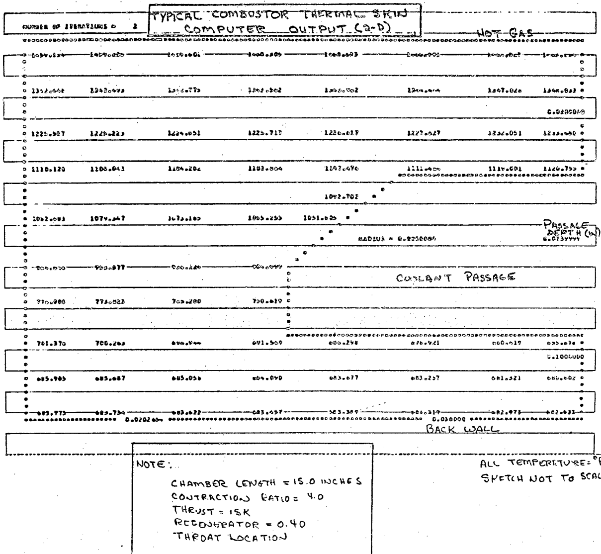
Figure 4-11. Detailed Thermal Map
