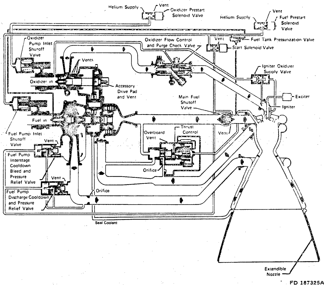
Figure 2-21. Propellant Flow Schematic for Derivative IIC Engine
