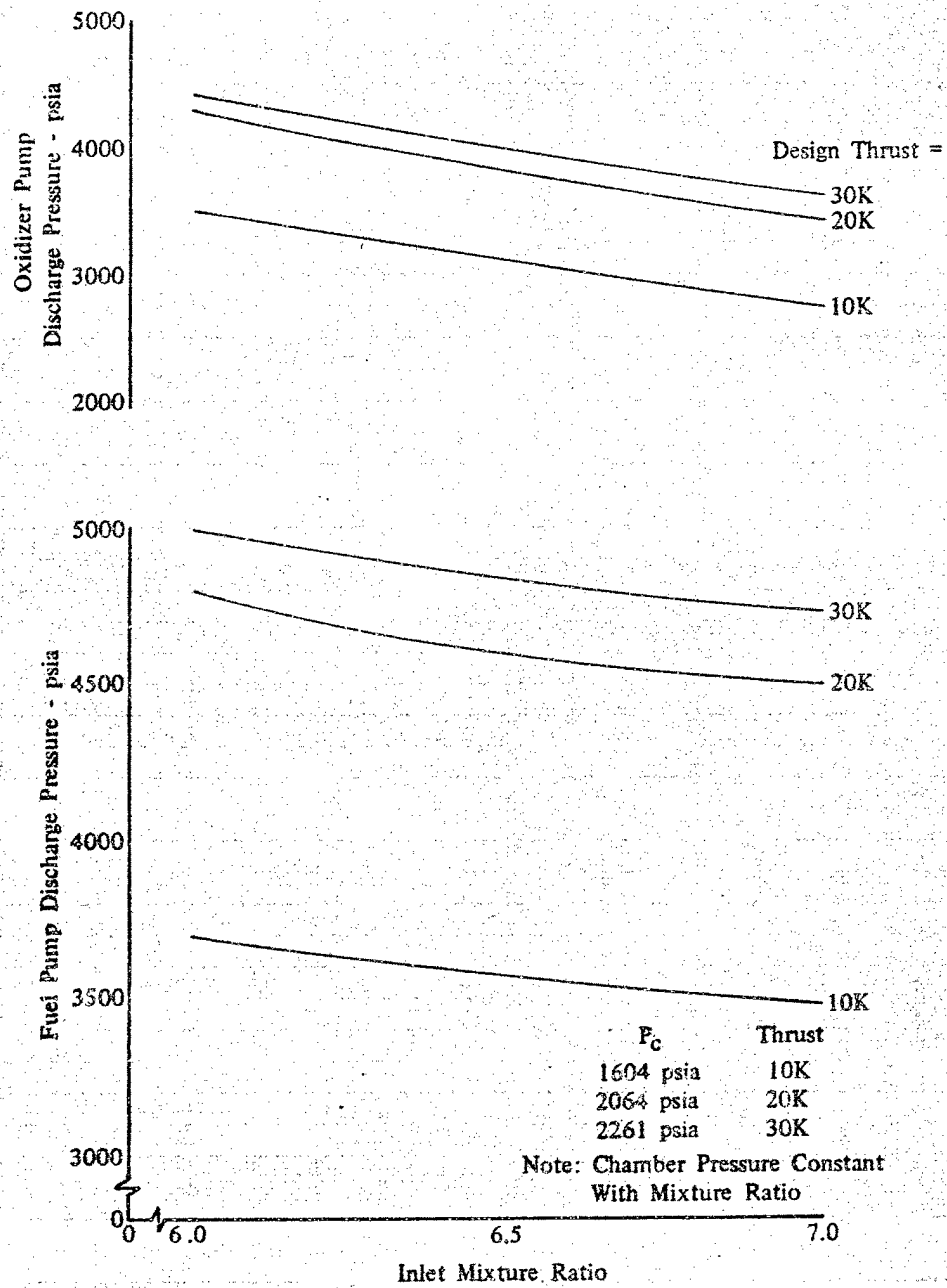
Figure 3-24. Staged Combustion Engine Off-Design Pump Discharge Characteristics
