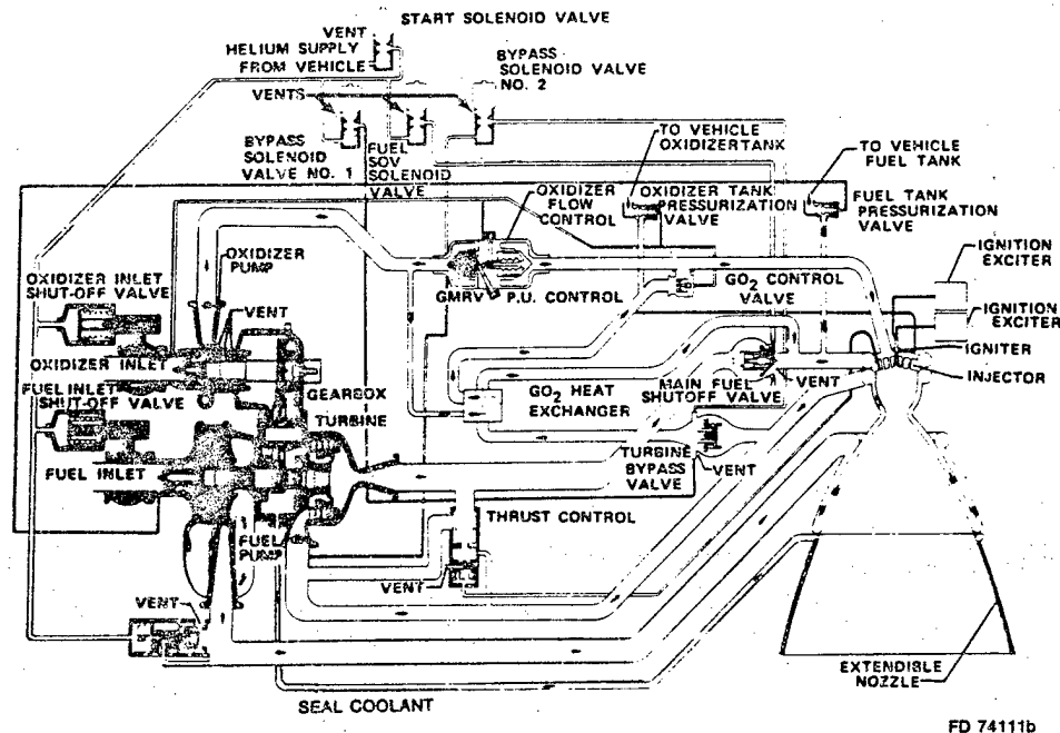
Figure 2-15. RL10 Derivative IIB Propellant Flow Schematic
