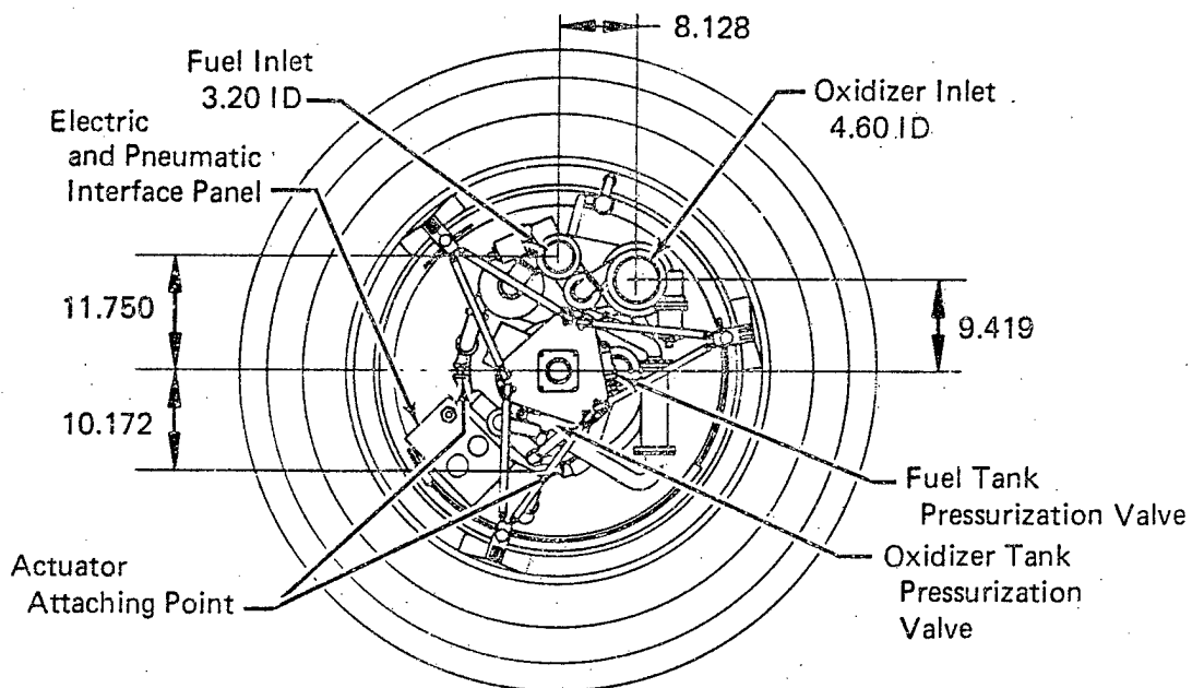
Figure 2-25. Category IV Engine Installation Drawing
