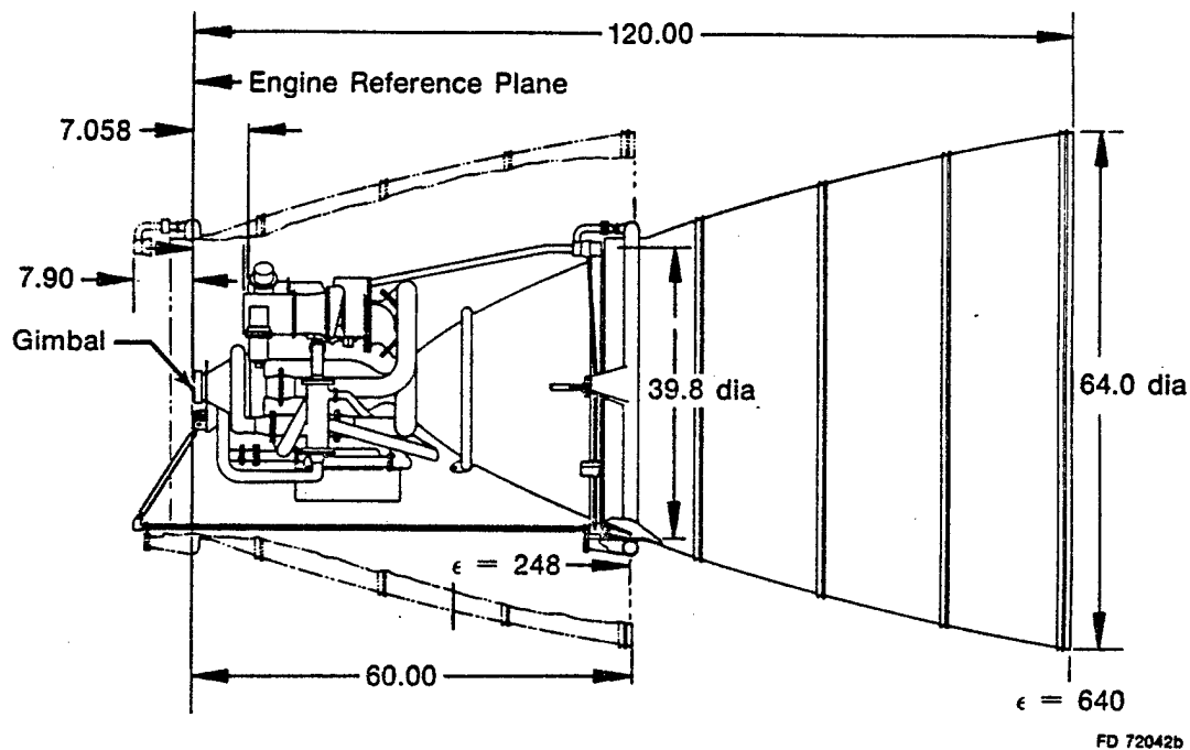
Figure 2-31. Advanced Expander Engine Installation Drawing
