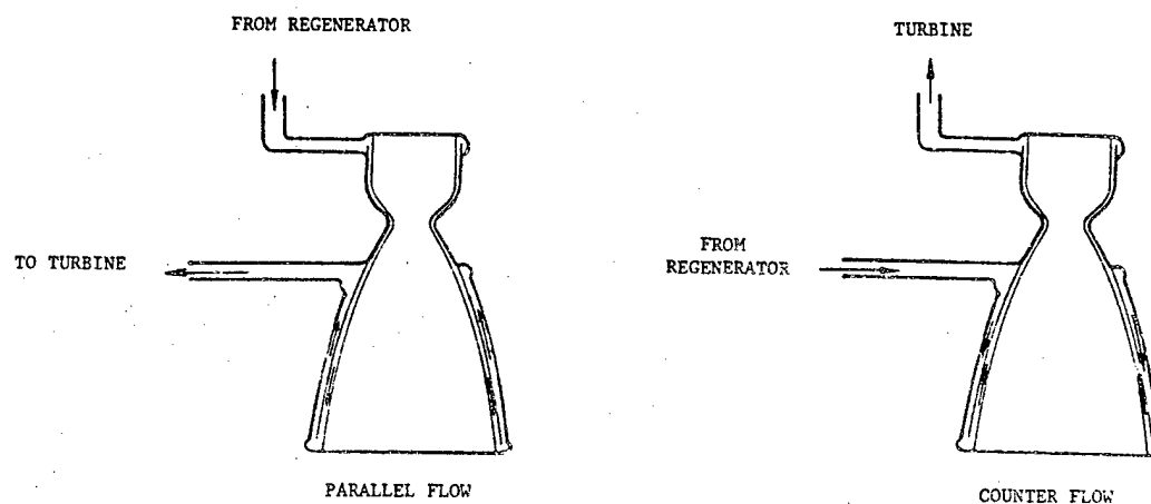
Figure 4-6. Parallel and Counterflow Chamber/Nozzle Coolant Flow Routing Schemes
