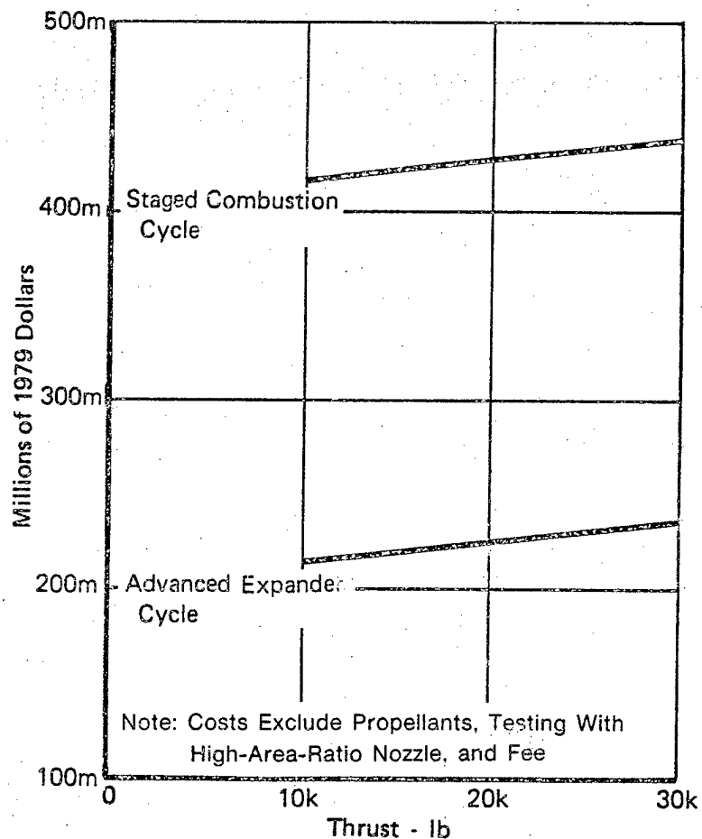
Figure 3-28. OTV Engine Parametric DDT&E Cost
