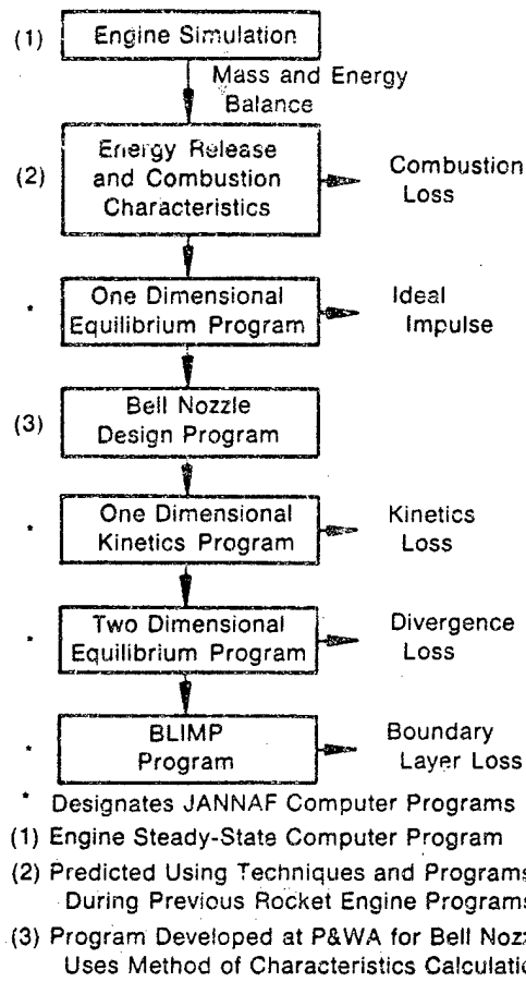
Figure 2-1. Performance Prediction Programs
