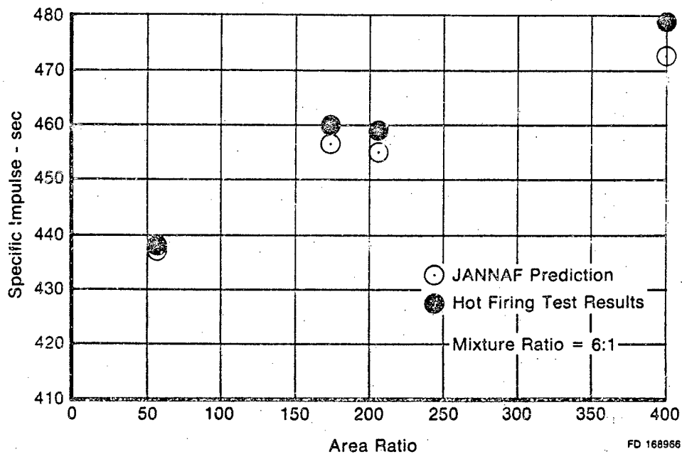
Figure 2-2. Comparison of JANNAF-Predicted Performance With Test Results
