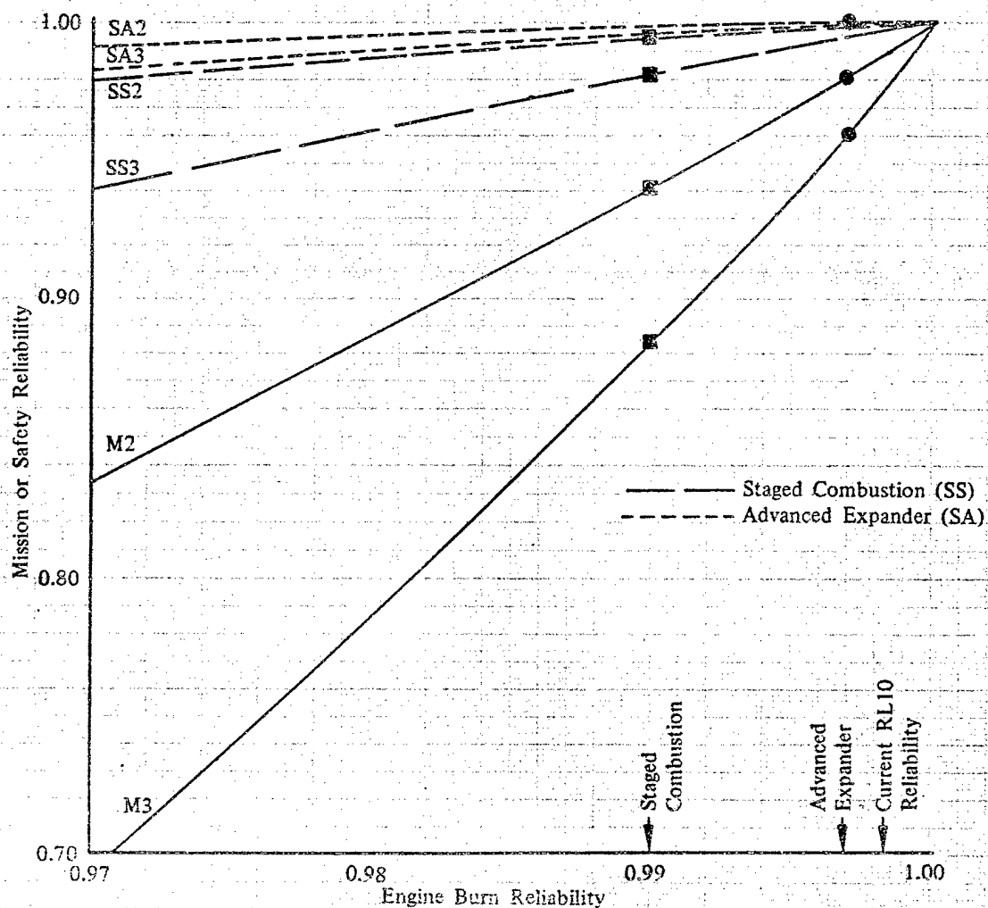
Figure 6-8. OTV Reliability With Advanced Engines
