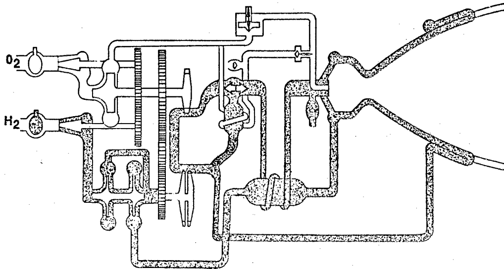
Figure 4-1. Advanced Expander Engine Configuration
