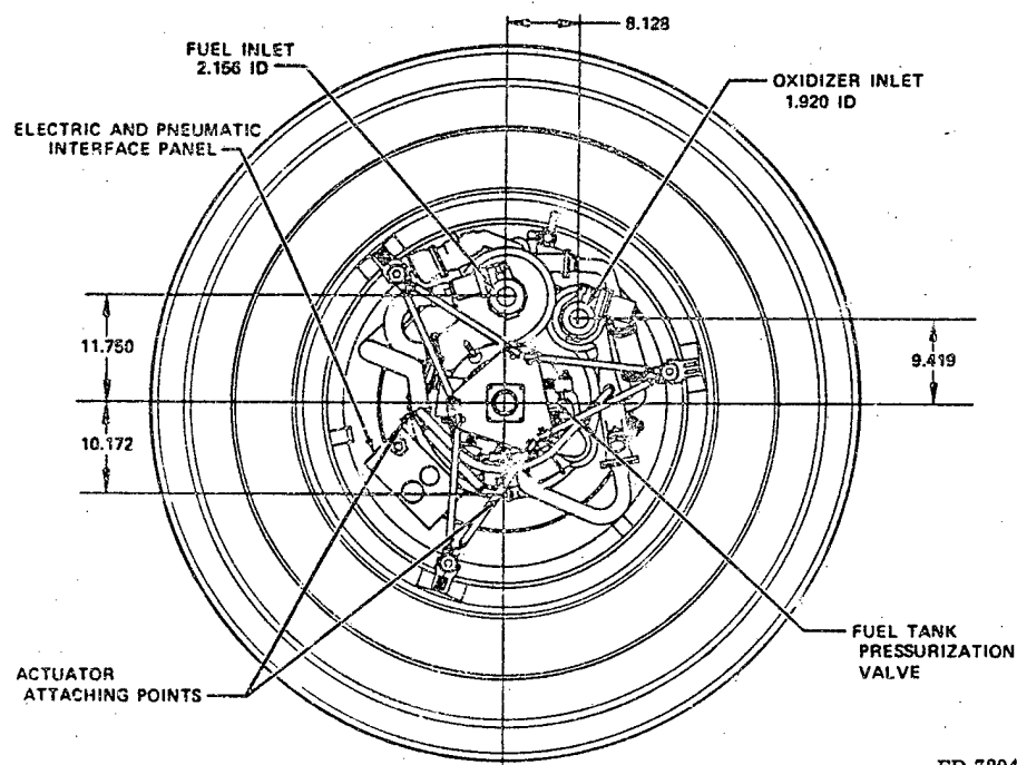
Figure 2-20. RL10 Derivative IIC Installation Drawing (Sheet 2)
