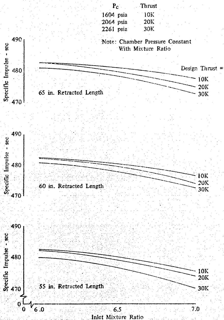
Figure 3-27. Staged Combustion Engine Off-Design Performance Characteristics
