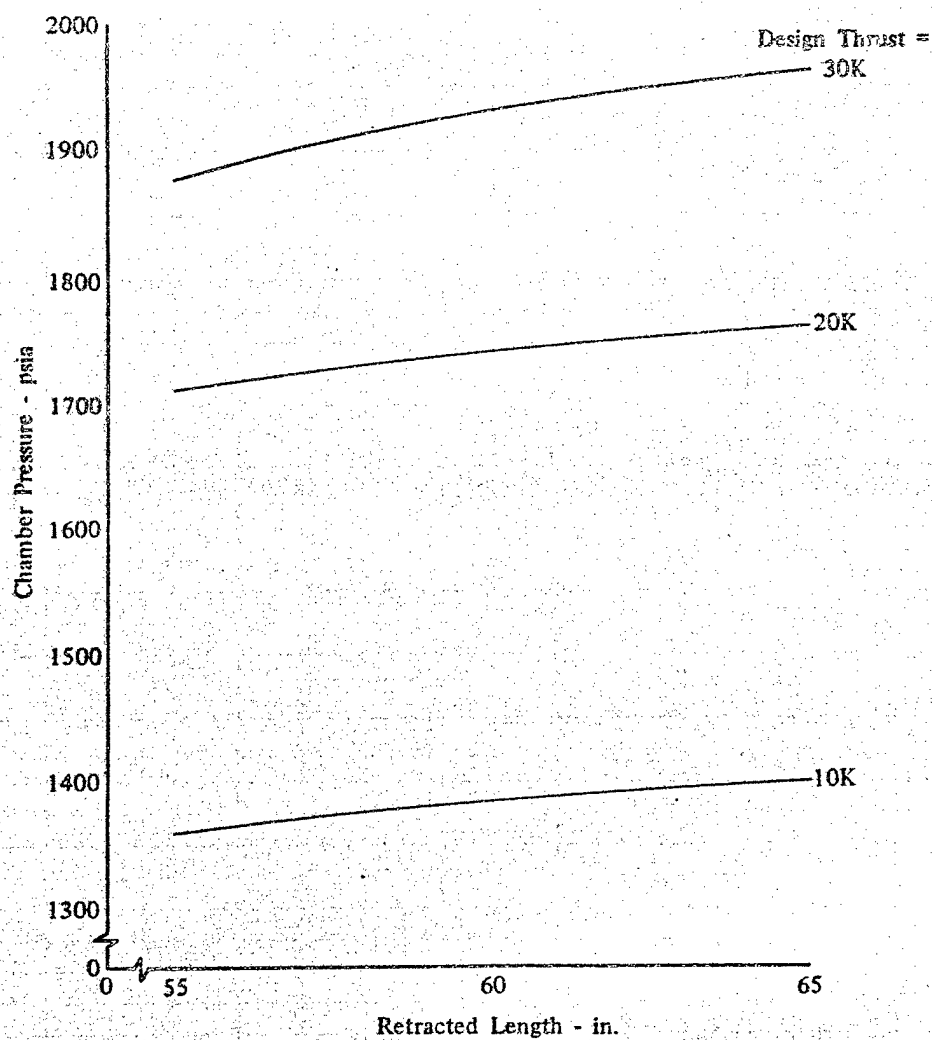
Figure 3-8. Advanced Expander Cycle Chamber Pressure Characteristics
