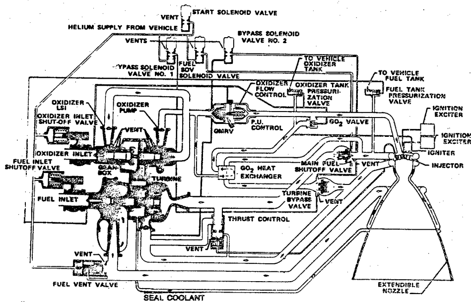
Figure 2-6. RL10 Derivative IIA — Propellant Flow Schematic
