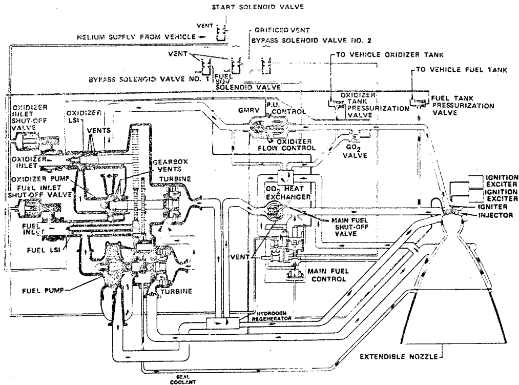
Figure 2-32. Advanced Expander Engine Propellant Flow Schematic
