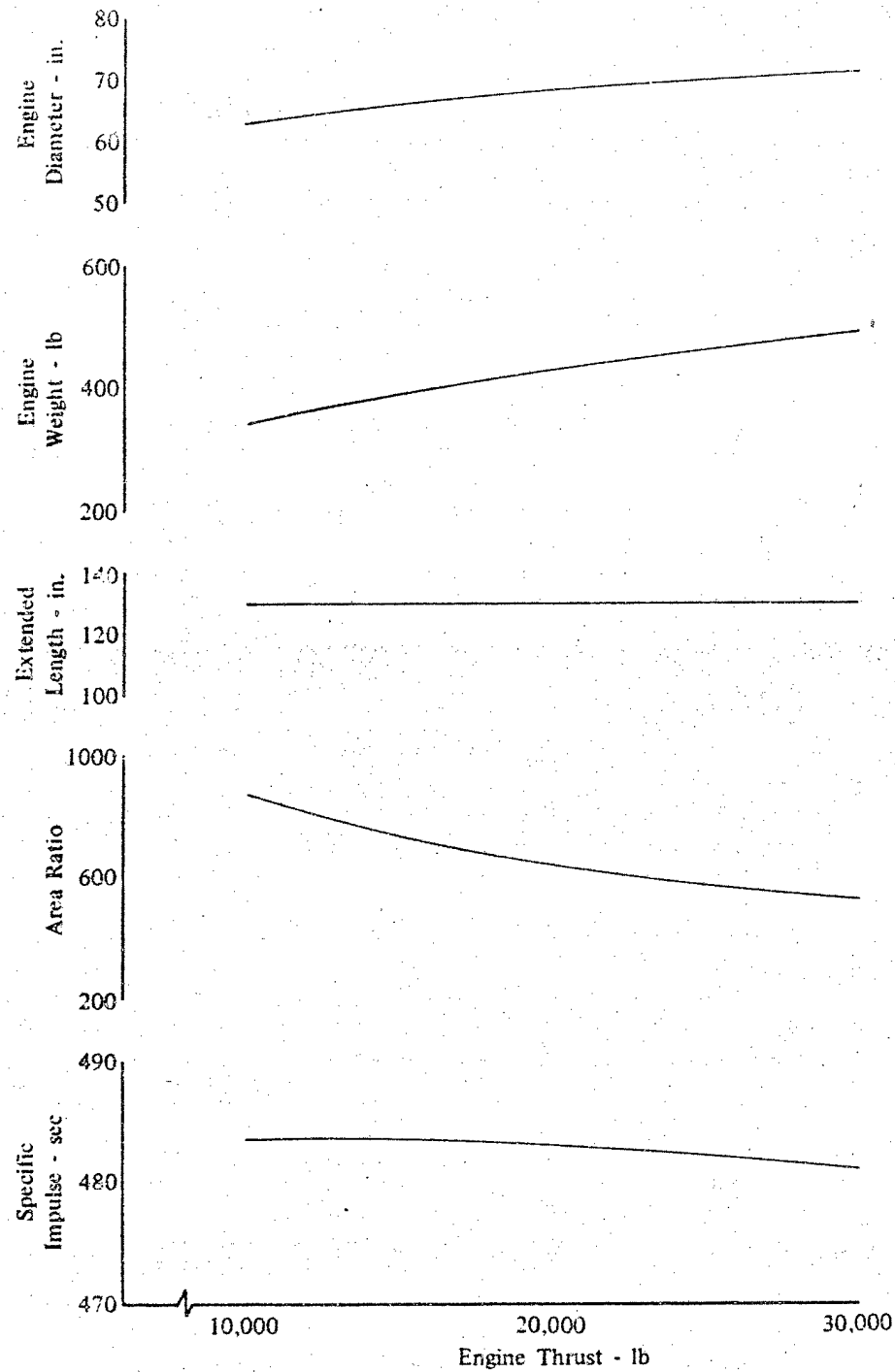
Figure 3-14. Advanced Expander Engine Parametric Characteristics (65 in. Retracted Length)
