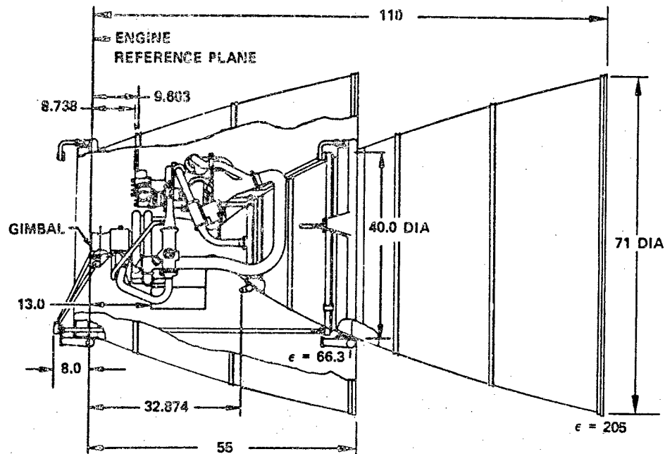
Figure 2-19. RL10 Derivative IIC Installation Drawing (Sheet 1)
