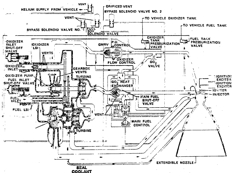
Figure 2-27. Category IV Propellant Flow Schematic
