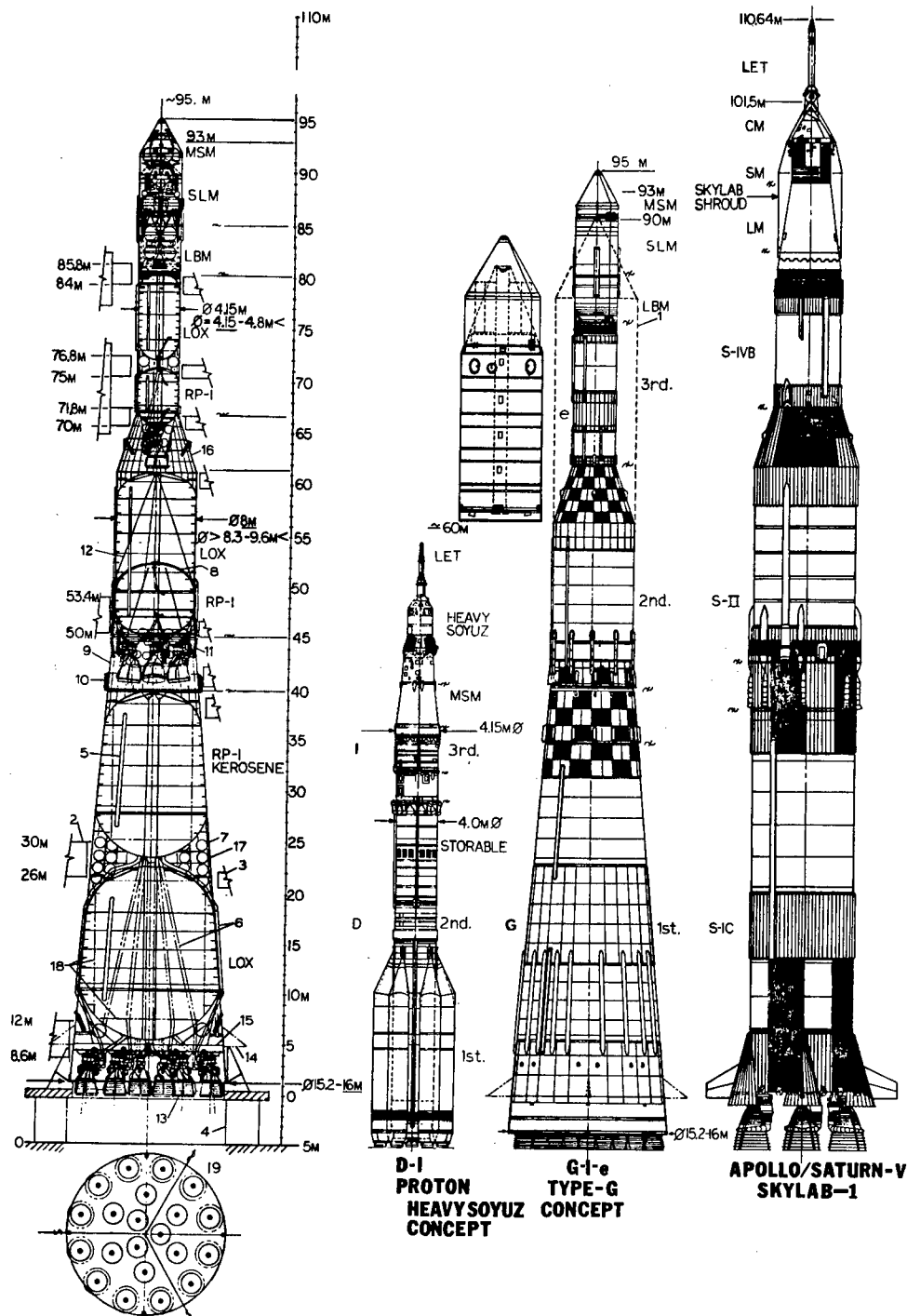
Figure 2-1.—Soviet Type G Booster, and U.S. Saturn V
