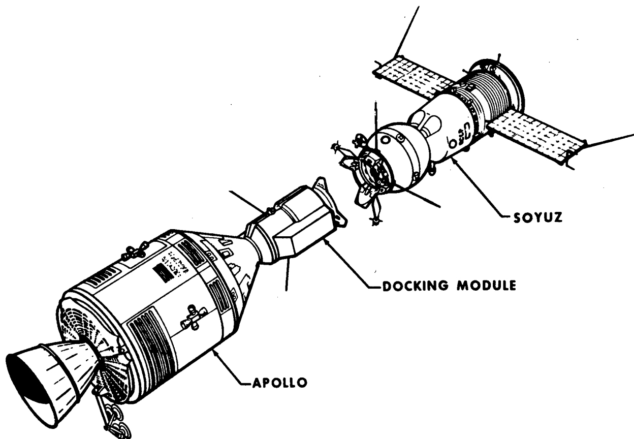
Figure 2-3.—Apollo Command Module and Soviet Soyuz Counterpart
