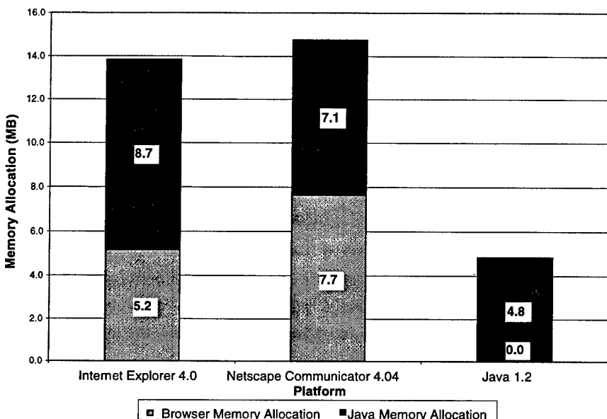
Figure 3: Memory Usage
