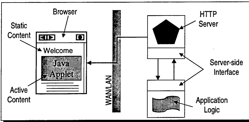
Figure 1: Browser-Based Design
