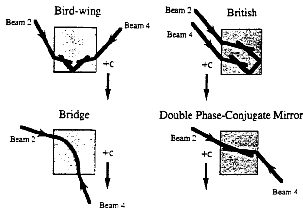
Fig. 1. Four different mutually pumped phase conjugators. The British and the bird-wing conjugators use internal reflections to guide the beams.
