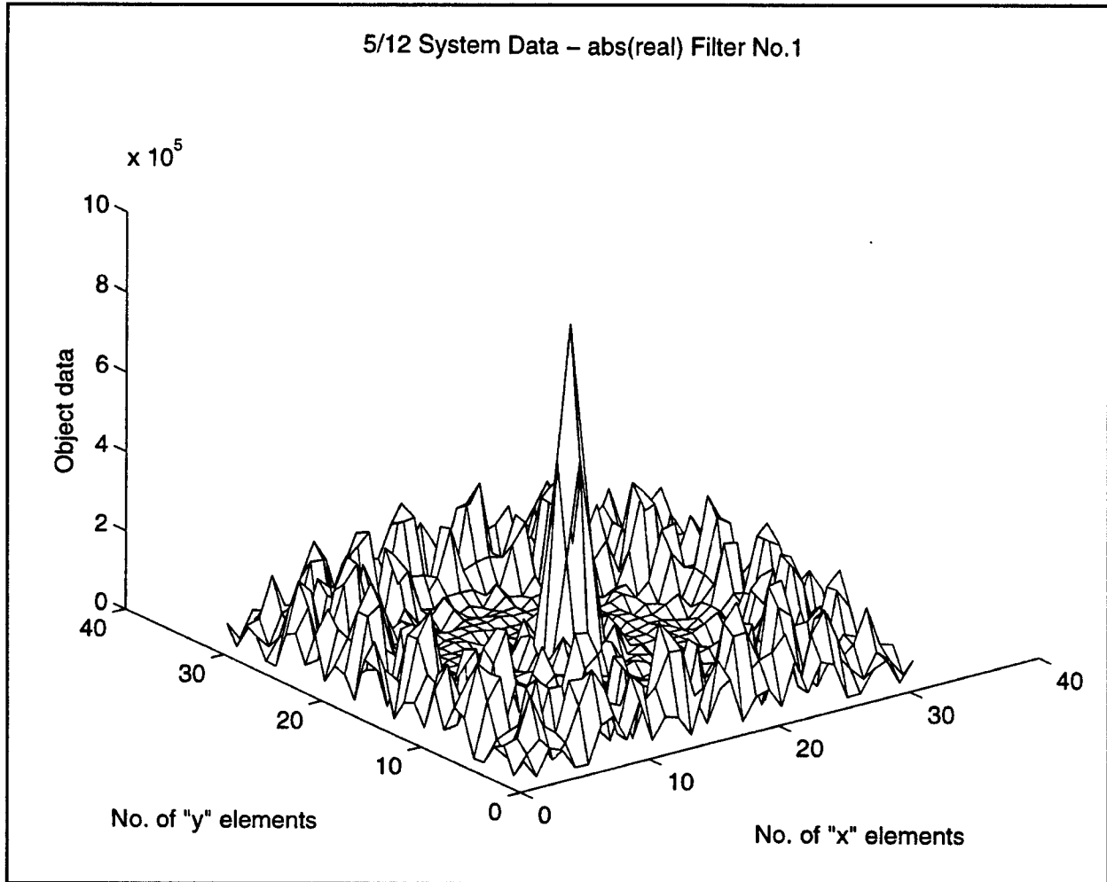
Figure B6. Image with old system at 1.0 GHz
