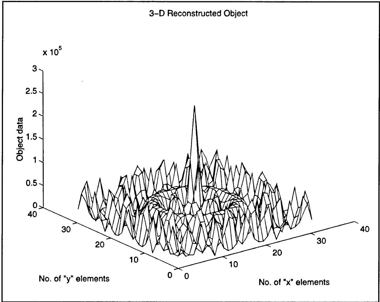
Figure B7. Image with new system at 1.0 GHz
