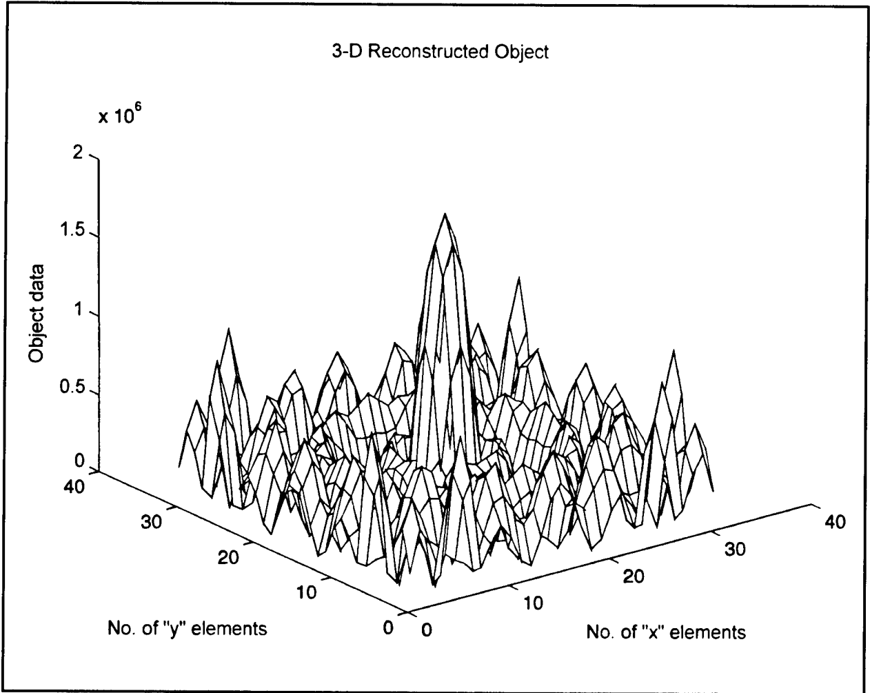
Figure B9. Image with new system at 2.0 GHz
