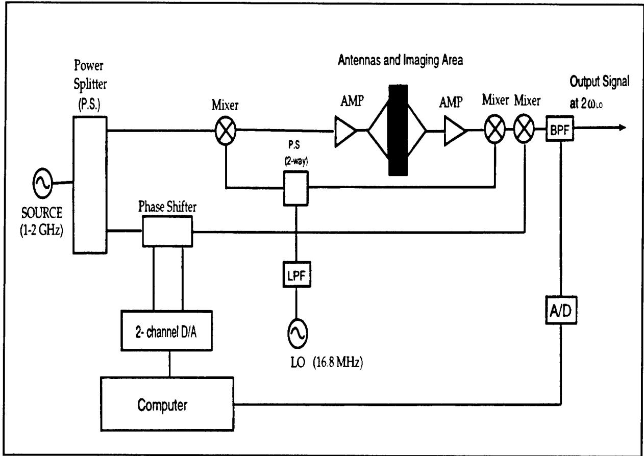
Figure B3. Old SFR system design
