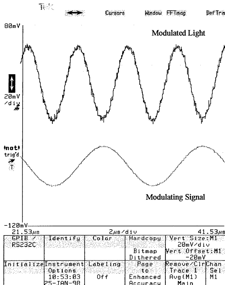
Figure 3.8. Inverted, double modulation of a modulator, V_{dc} set to peak intensity.
