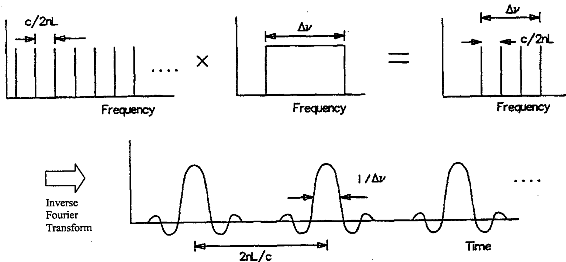
Figure 2.3. Frequency domain illustration of mode-locking, conversion to the time domain shows the mode-locked pulses. (After [Ref. 14].)
