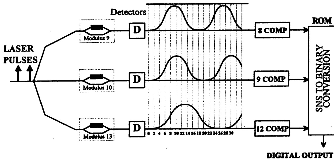
Figure 1.5. Symmetrical-numbering-system ADC. (From [Ref. 3].)
