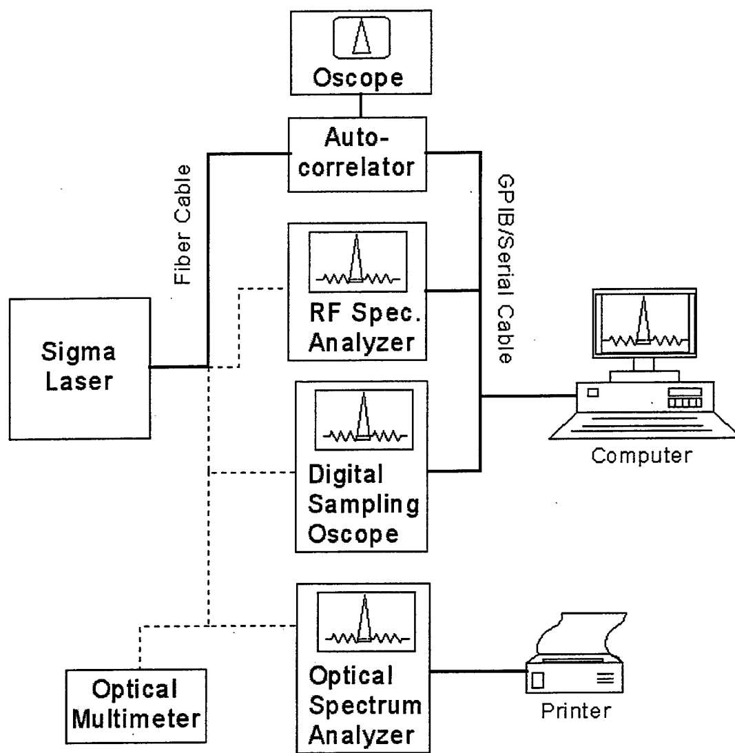
Figure 4.1. Test and measurement equipment layout with connections.
