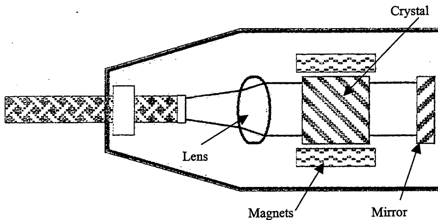
Figure 3.4. Faraday rotator mirror. (After [Ref. 38].)
