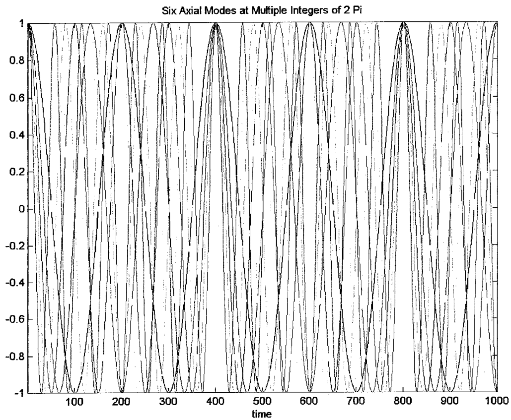
Figure 2.4b. Modes plotted together, note matching phase at time 400 and 800.
