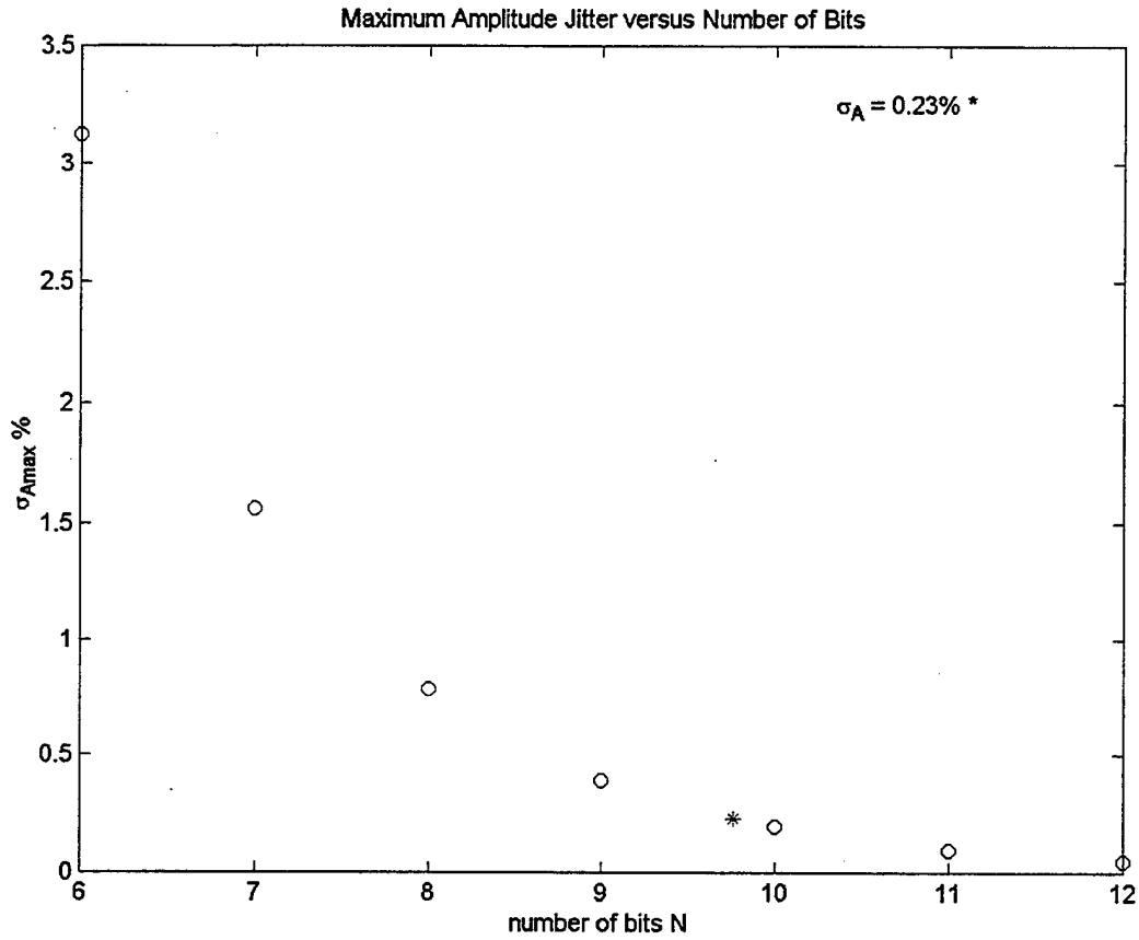
Figure 5.1. Maximum percentage of amplitude jitter versus number of bits.
