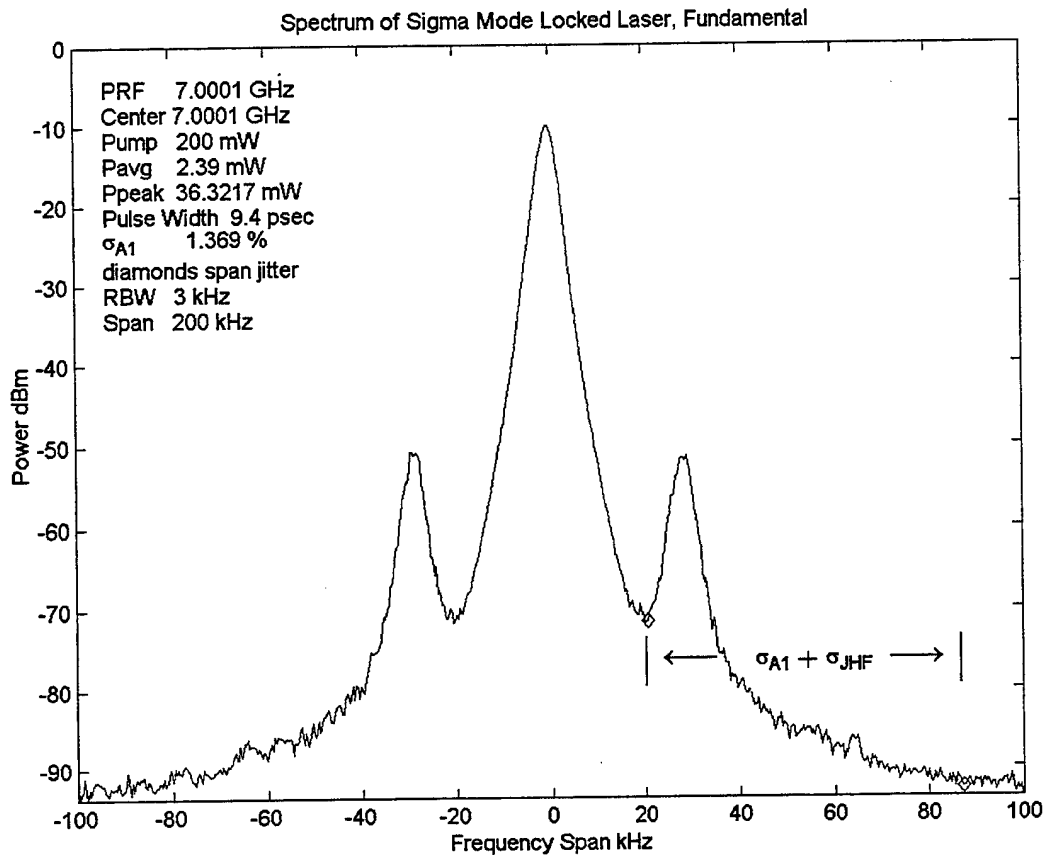
Figure 4.11. Fundamental mode-locked signal, 7 GHz PRF, 200 kHz span.
