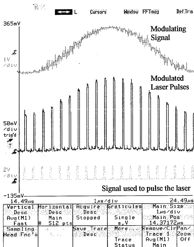
Figure 1.3. Laser pulses modulated by an analog signal.
