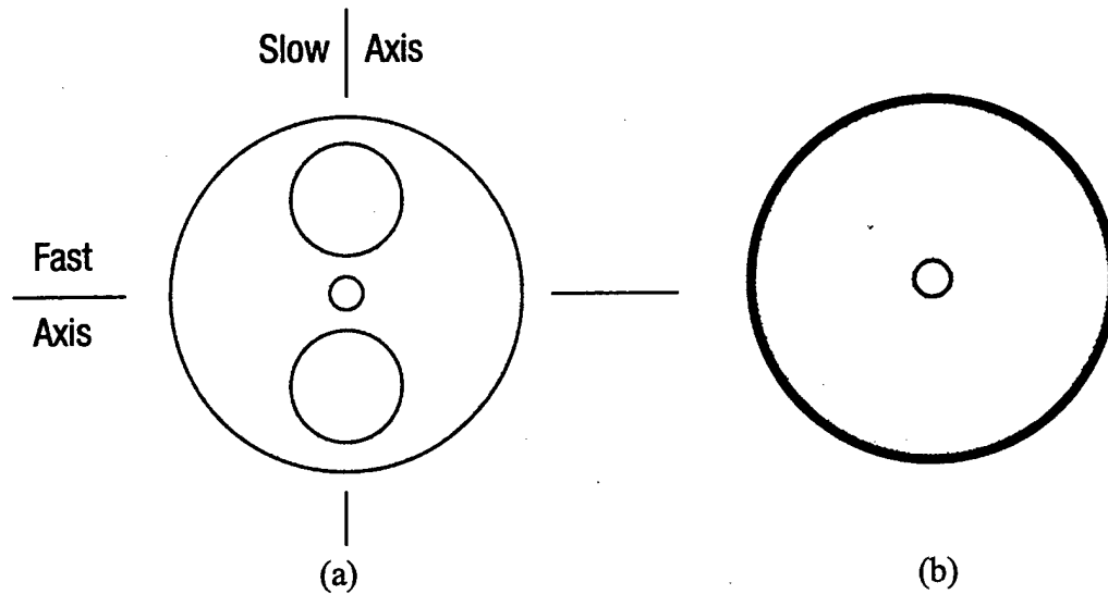
Figures 3.3 (a) PM and (b) SM fiber cross sections. (From [Ref. 37].)
