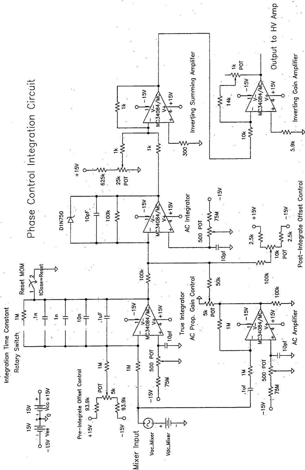
Figure 3.14. Integrating amplifier circuit. (After [Ref. 17].)
