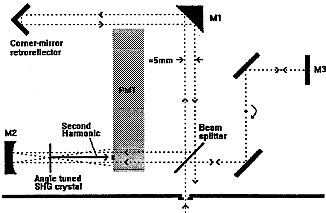
Figure 4.5. Internal layout of Femtochrome autocorrelator. (From [Ref. 64].)
