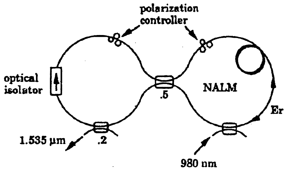
Figure 2.7b. Passively mode-locked figure-eight nonlinear-loop-mirror fiber laser. (From [Ref. 29].)
