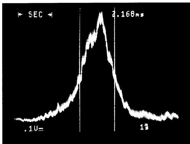
Figure 4.6b. Oscilloscope display of a autocorrelator pulse, 10 GHz PRF.
