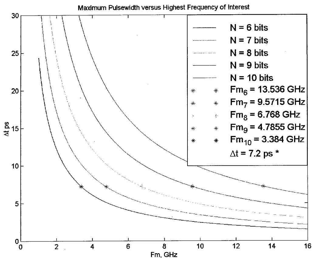
Figure 5.3. Maximum allowed pulsewidth versus highest frequency of interest.
