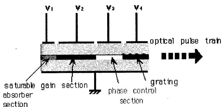
Figure 2.6. Passively mode-locked semiconductor laser. (From [Ref. 27].)
