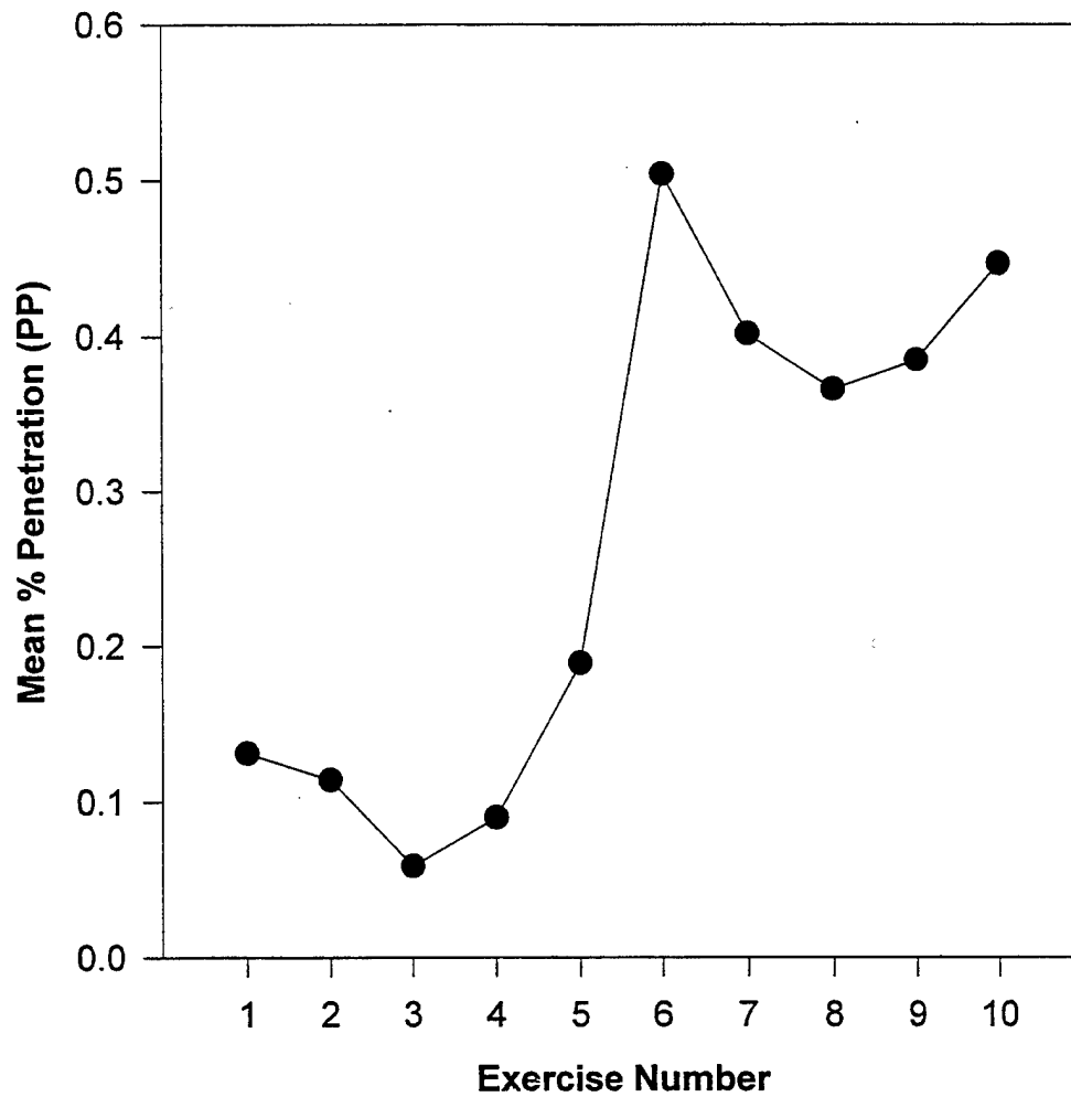
Figure 2. Plot of mean percent penetration vs. exercise number for CCBA/suit configuration.
