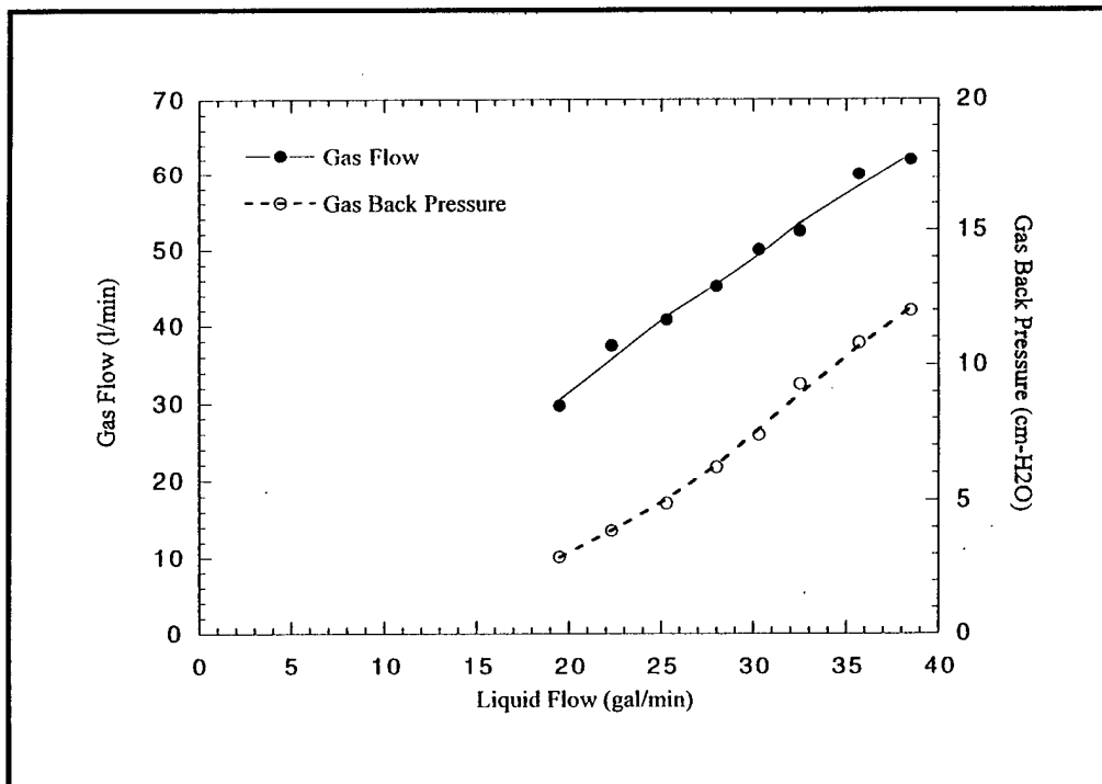
Figure 12. Gas back pressure, experiment #1, model 1584.
