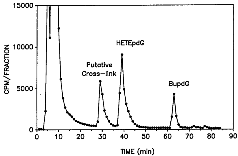
Figure 3. HPLC Profile of 32 P-postlabeled Nucleotides from DNA of Human Fibroblasts Exposed to SM in Cell Culture. DNA, isolated from fibroblasts that had been exposed to 100 \mu M SM for 1 h, was digested and subjected to postlabeling as described in reference 47. Labeled nucleotides were separated by HPLC on a C 18 column; 1 min fractions were collected and counted. A peak labeled "putative cross-link" eluted in front of the principal DNA adduct, HETEpdG, and the internal standard peak, BupdG.
