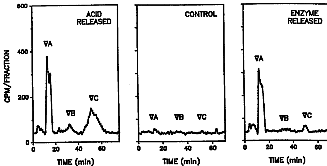
Figure 7. HPLC Profiles of Bases Released from Ring-opened SM-modified DNA. Retention times are indicated for optical markers of: A, ro-HETEG; B, HETEA; and C, HETEG. The panels from left to right show radioactivity released by acid depurination, control incubation with buffer alone, or incubation with Fpg protein for 15 min at 37°C (see text for details).
