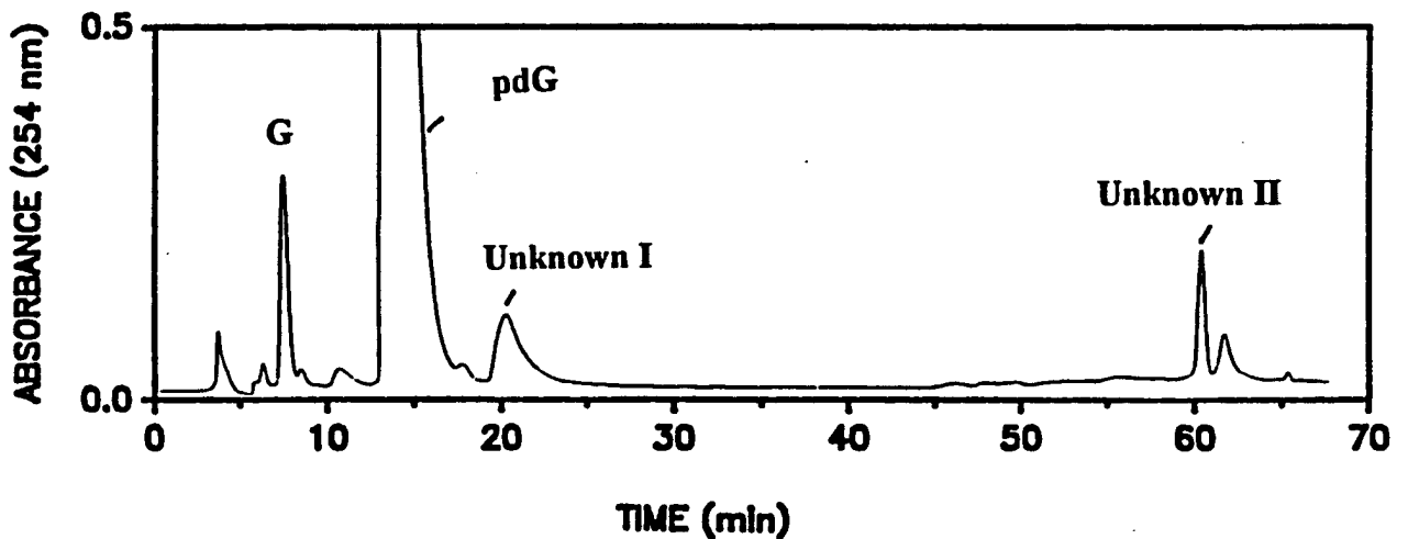
Figure 4. HPLC Profile of Products Obtained in the Reaction Shown in Figure 2. A sample of the reaction products was eluted from a C 18 column using a slower gradient than that used in Figure 3.
