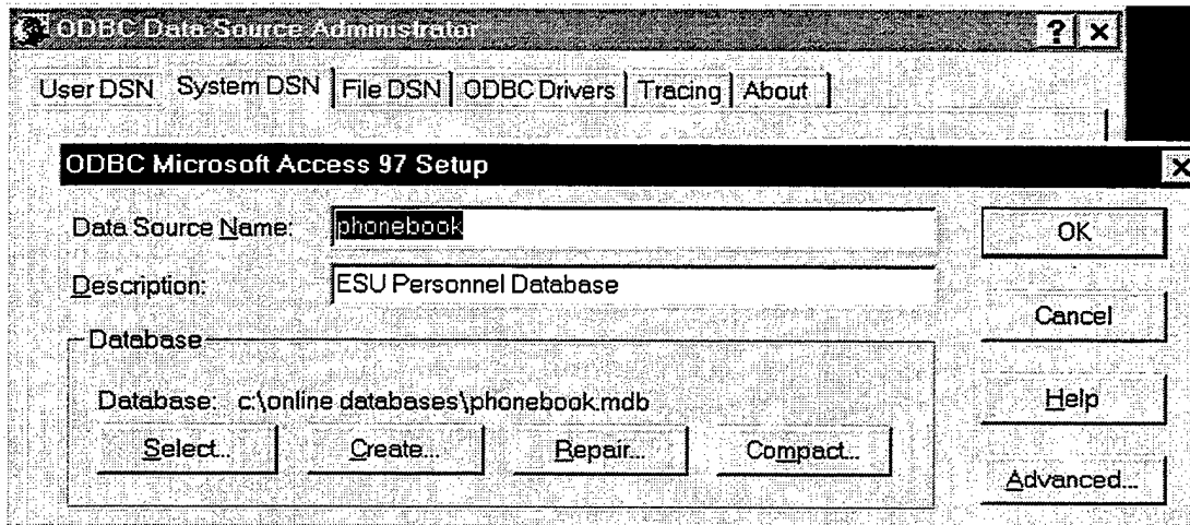
Figure 7.2 ODBC System DSN Setup Window
