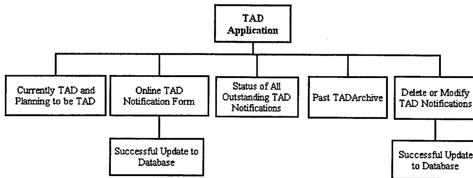
Figure 8.21 TAD Application Navigation Structure
