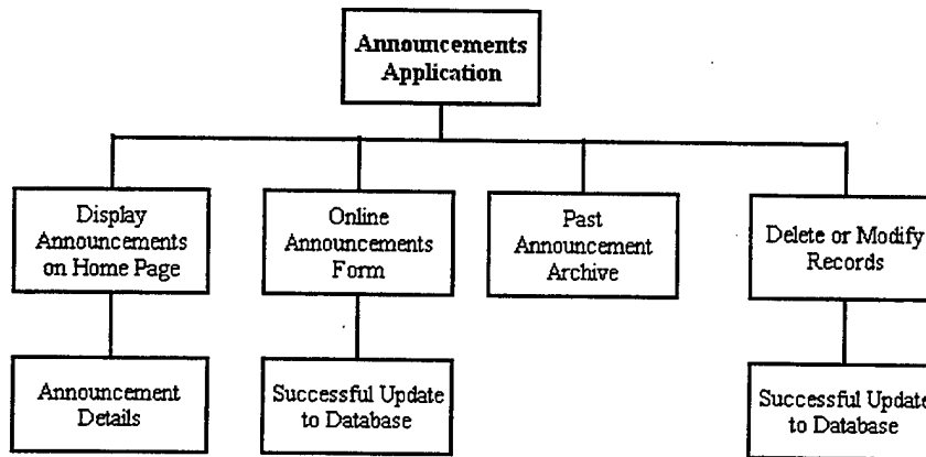
Figure 8.26 Announcement Application Navigation Structure
