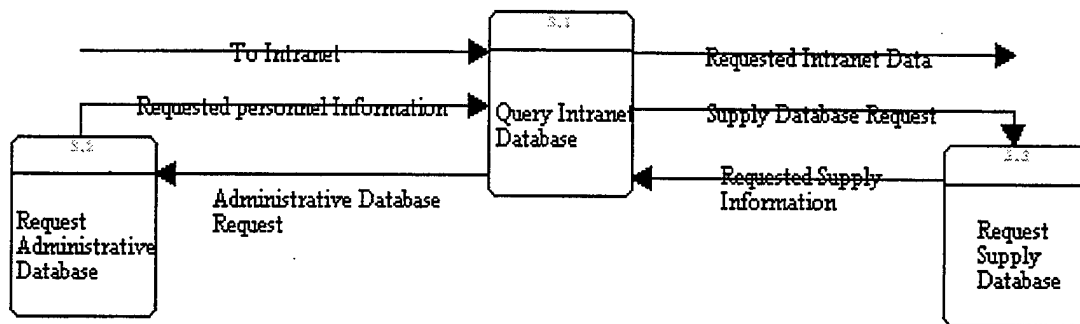
Figure 5.6 Level 1 DFD for Intranet
