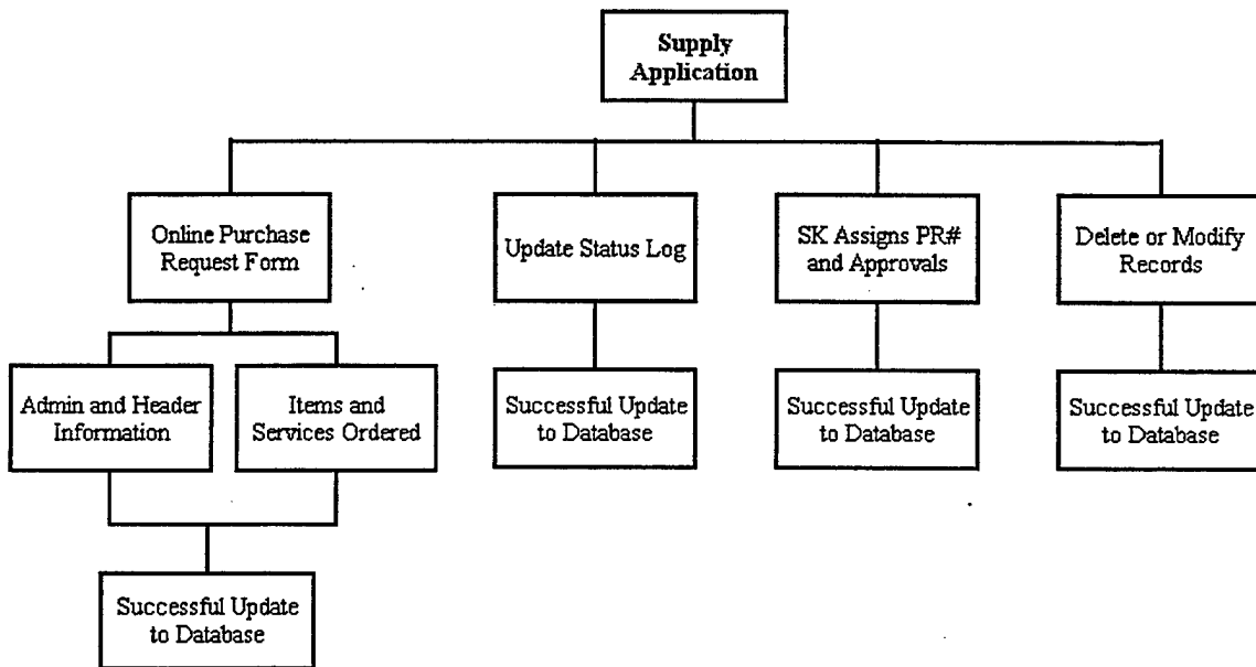
Figure 8.40 Supply Application Navigation Structure
