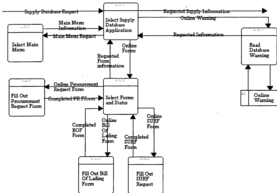
Figure 5.7 Level 2 DFD of Supply Application
