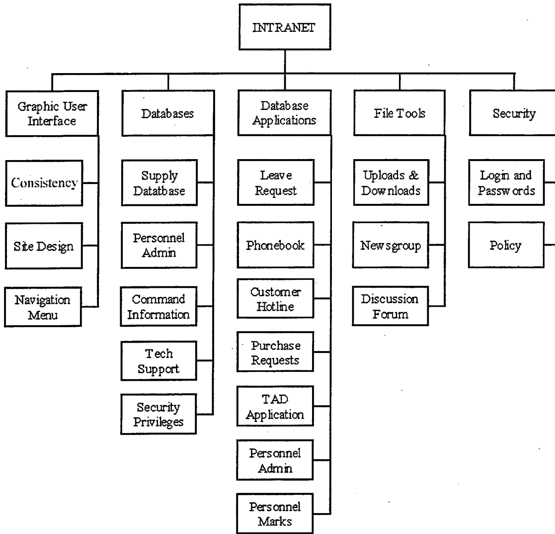
Figure 5.9 Functional Decomposition Diagram of ESU Intranet
