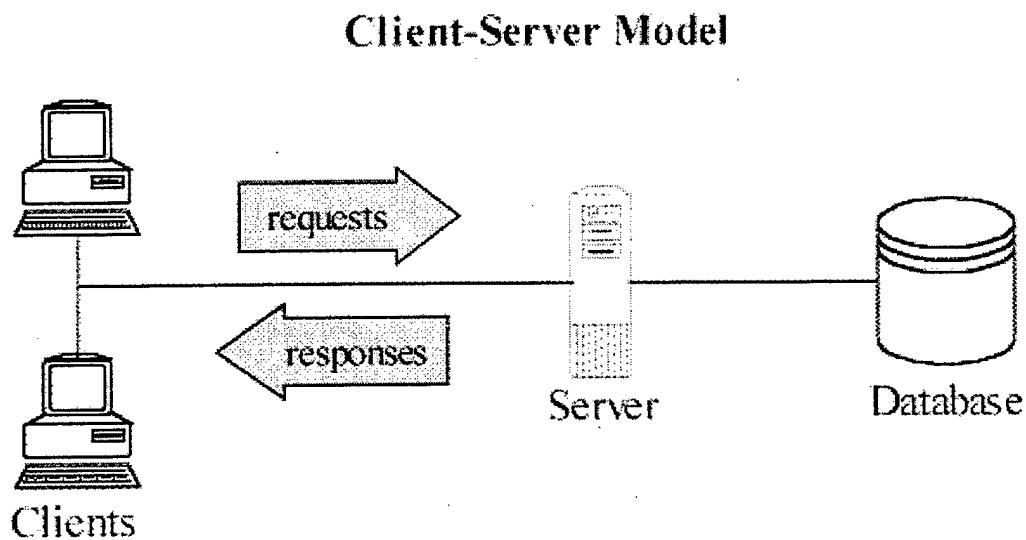
Figure 2.2 Client-Server Model
