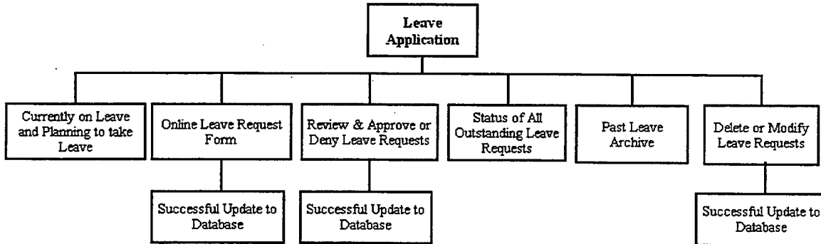
Figure 8.12 Leave Admin Application Navigation Structure
