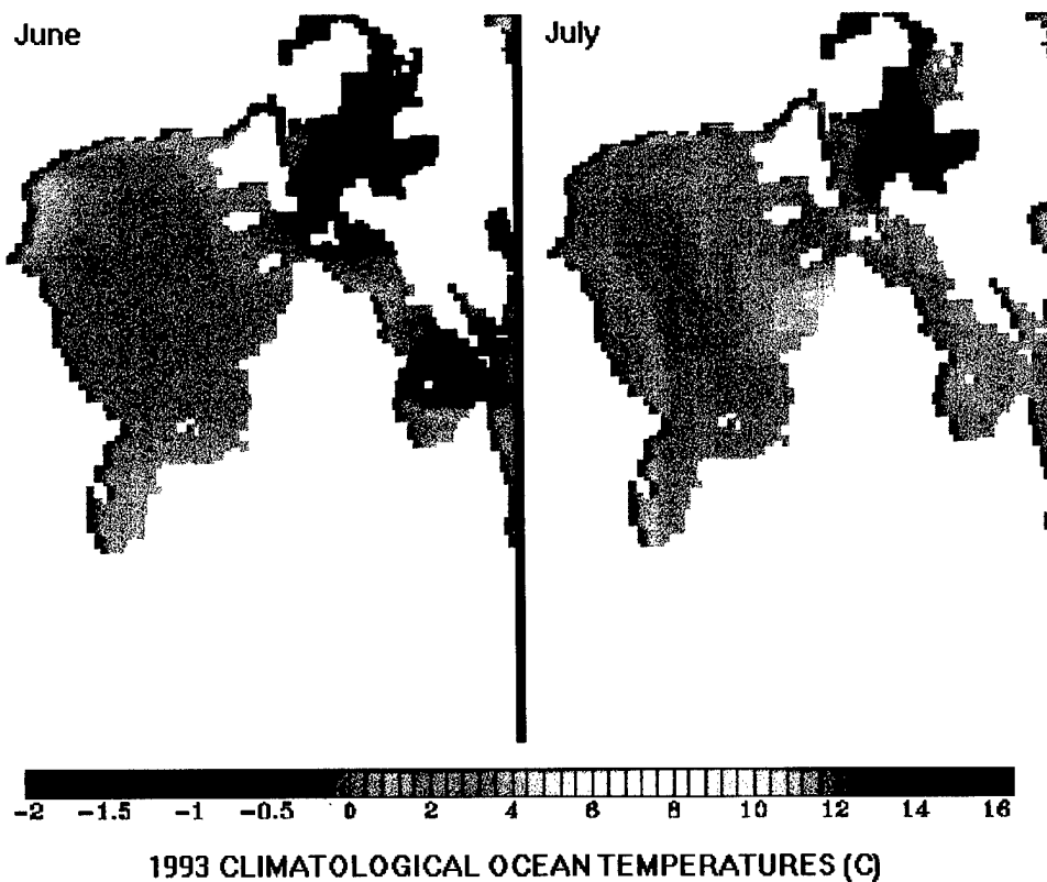
Figure 5-4. Levitus and Boyer ocean temperatures for June (left) and July (right) 1993. The figures show a delayed temperature increase in July.
