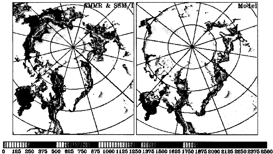
Figure 5-9. Variance for the satellite ice concentration observations (a) and model simulation (b). Favorable comparison is evident in the Barents Sea. The Beaufort, East Siberian, Chukchi and Laptev Seas all have significantly lower variance in the model simulation.
