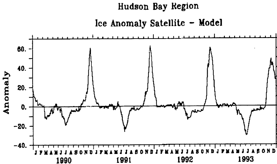
Figure 5-16 Hudson Bay sub-region anomaly curve for years 1990-93 shows strong positive anomaly peak in December followed by negative anomaly peak in July.
