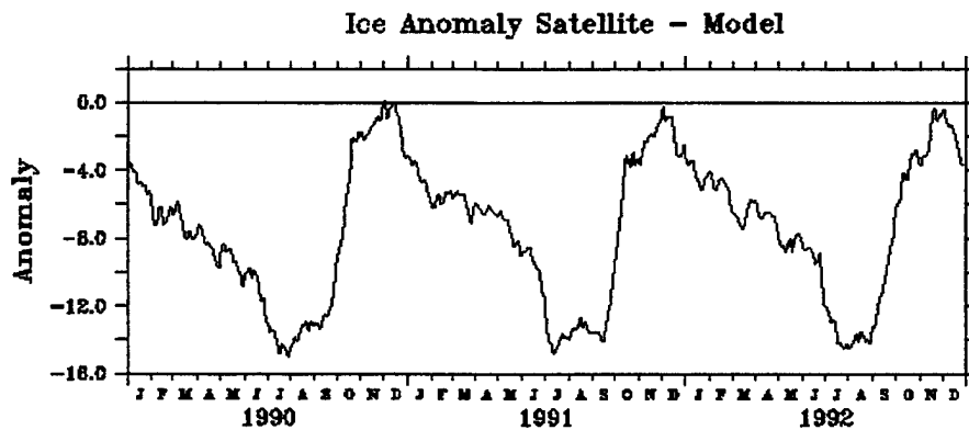
Figure 5-13. Time series of ice concentration anomaly (satellite observation minus model simulation) averaged over the entire model domain. Upper panel shows the seasonal variation over the 15-year model simulation. Lower panel provides detail on seasonal variation from 1990-92.
