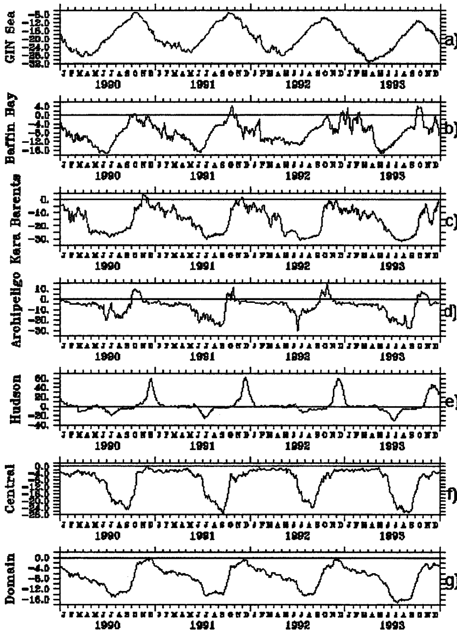
Figure 5-15. Time series of ice concentration anomaly for sub-regions (a-f) along with complete model domain (g). Sub-region boundaries are shown in Fig. 5-12.
