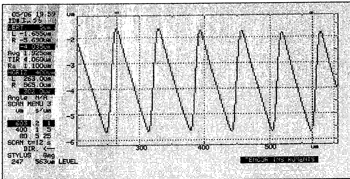
Figure 15. Profilometry scan of the off-axis field grating lens shown in Figure 14. Again, notice the linearity of the front blazed surfaces, the uniformity of each of the zones, and the smooth, continuous profile of the surface function.
