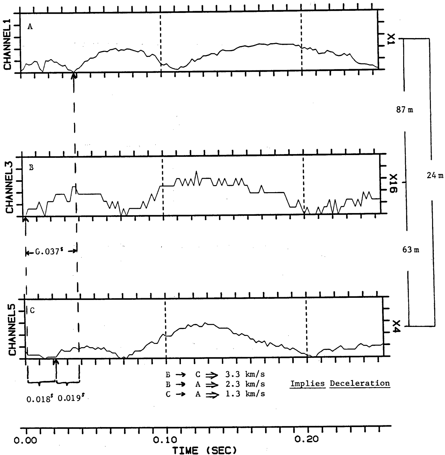
Figure 43. Time shifts in bistatic echoes during development of the echo power profile provide direct velocity measurement.
