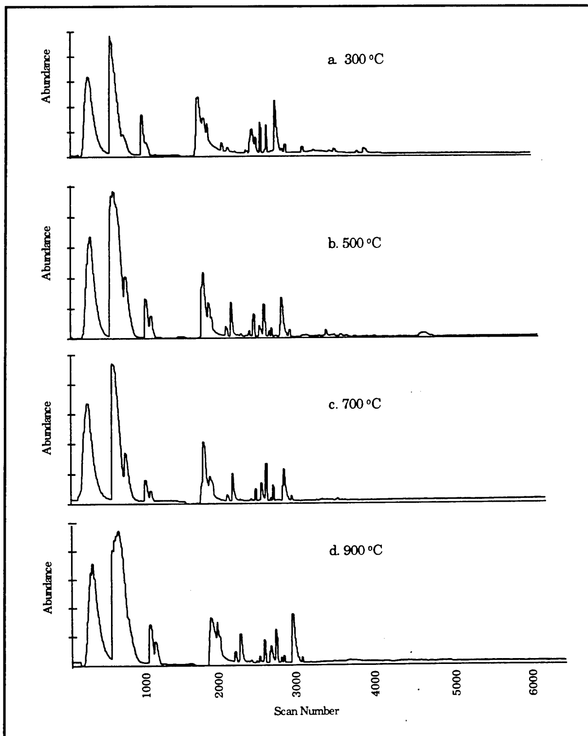
Figure 16. Pyrograms of PETN at (a) 300 °C, (b) 500 °C, (c) 700 °C, and (d) 900 °C using Configuration A2.
