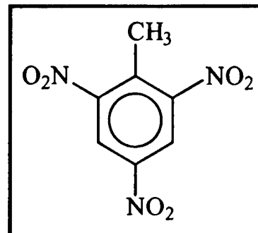
Figure 6. Structure of TNT.
