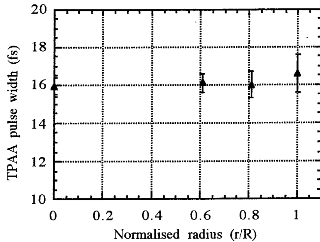
Figure 5. TPAA signal as a function of normalised radius at a dispersion pre-compensation setting giving the minimal pulse width at r/R=0 for the Zeiss CP-Apochromat 100x/1,25 oil microscope objective. The best fit was obtained assuming a \text{Sech}^2 input pulse.
