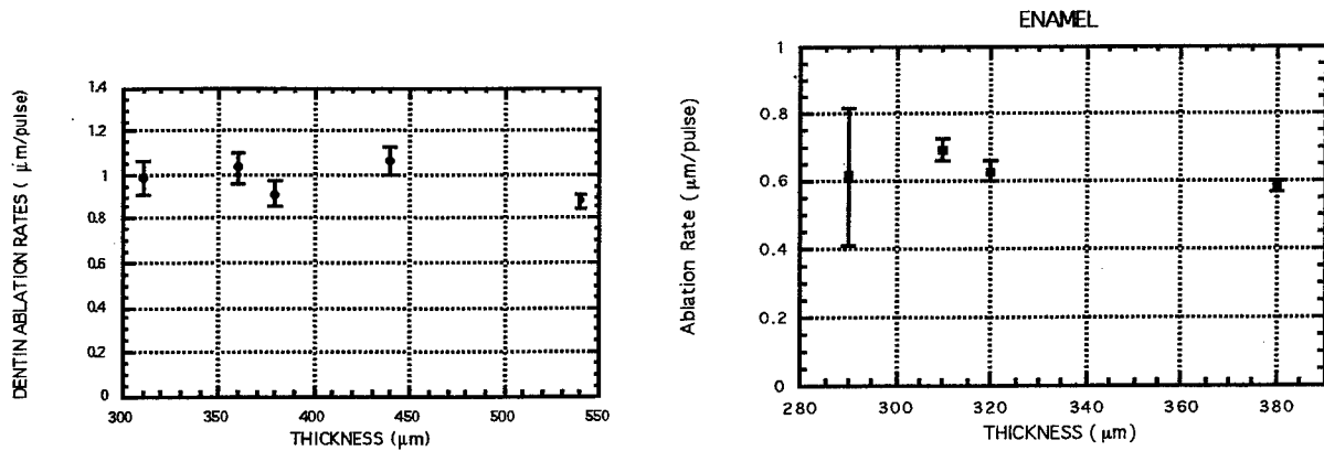
Figure 6. Enamel ablation rates as a function of ablated slice thickness
