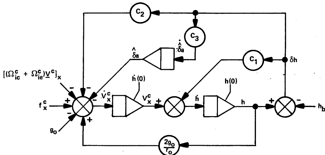
Figure 2-10. Third Order Damped Vertical Block Diagram
