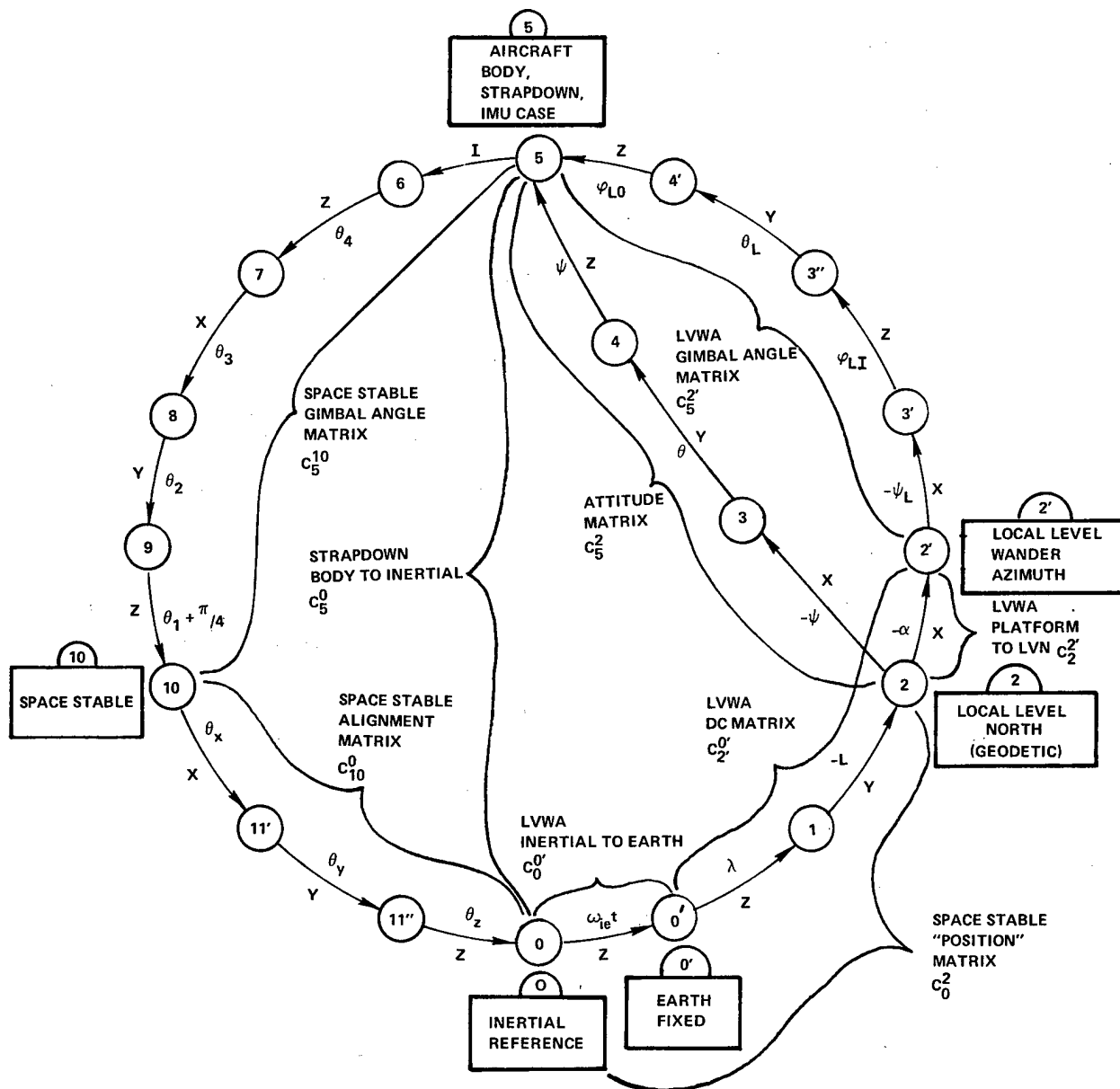
Figure A-9. General Circle Diagram for SS, SD, LVWA INS Computations
