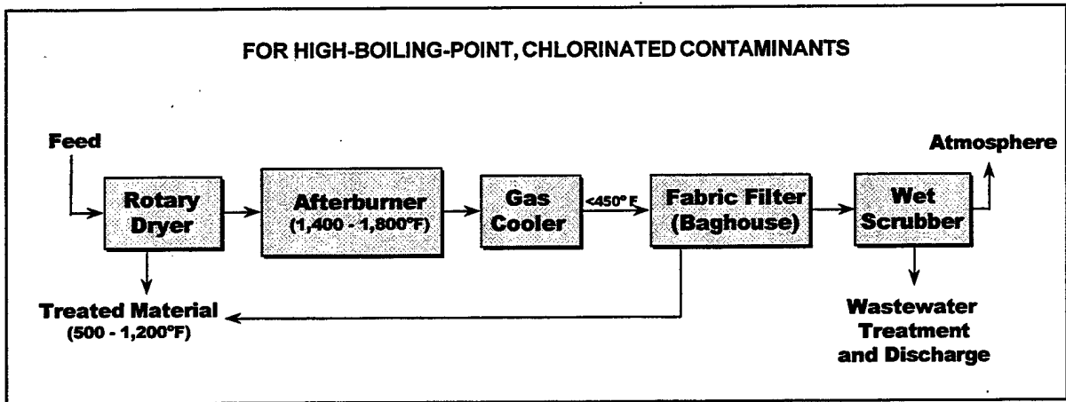
Figure 5. Third Generation—Direct-Contact Thermal Desorption Process
