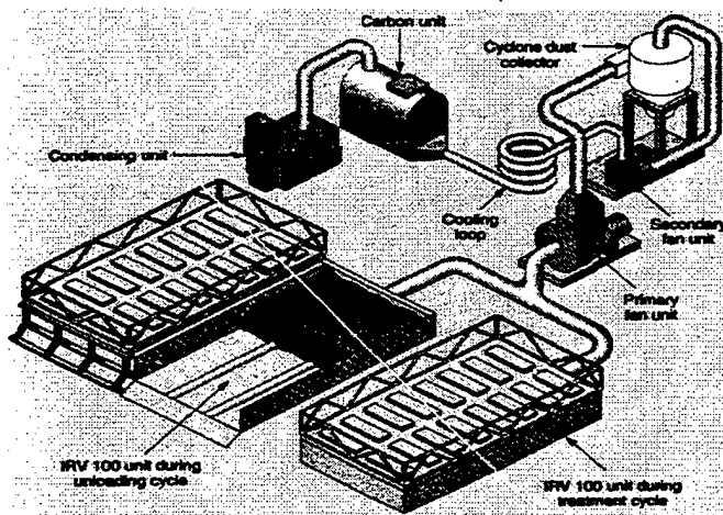
Figure 8. Batch-Feed Thermal Desorption System—Indirect-Contact Heated Oven
