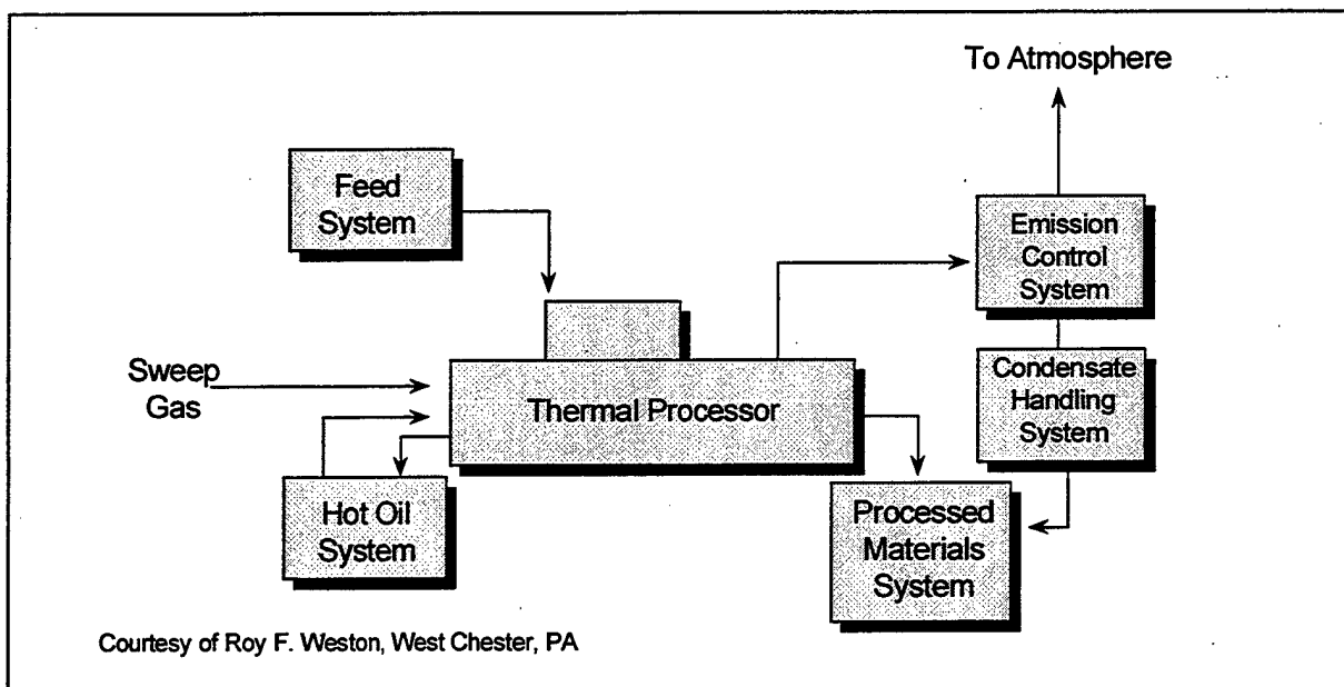
Figure 7. Typical Indirect-Contact Thermal Screw Thermal Desorption Process
