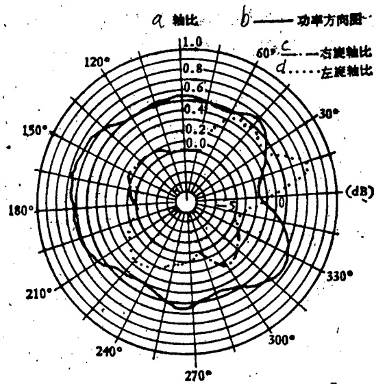
Fig. 7. Directional map at \varphi^n = 157.5^\circ
