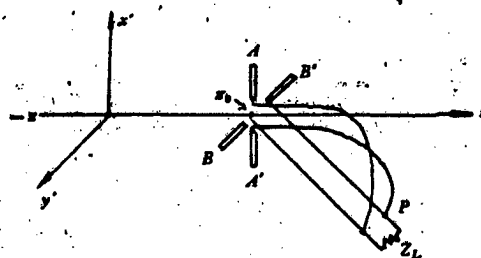
Fig. 2. Receiving antenna and its coordinate system
