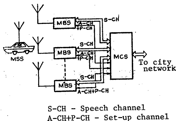
Figure 2. Structure of System's Signalling Channel
