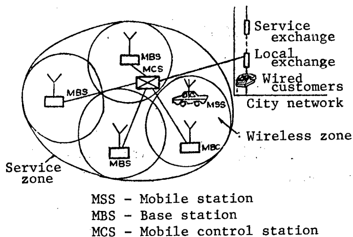
Figure 1. Network Structure
